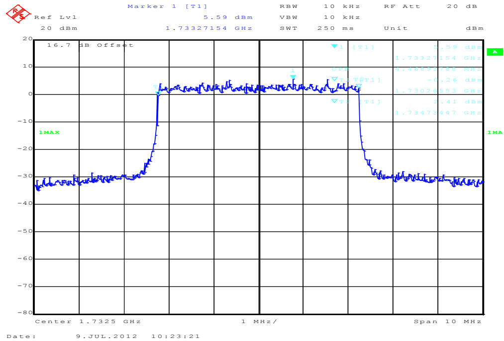
Plot 5: 5 MHz (99% - OBW)
