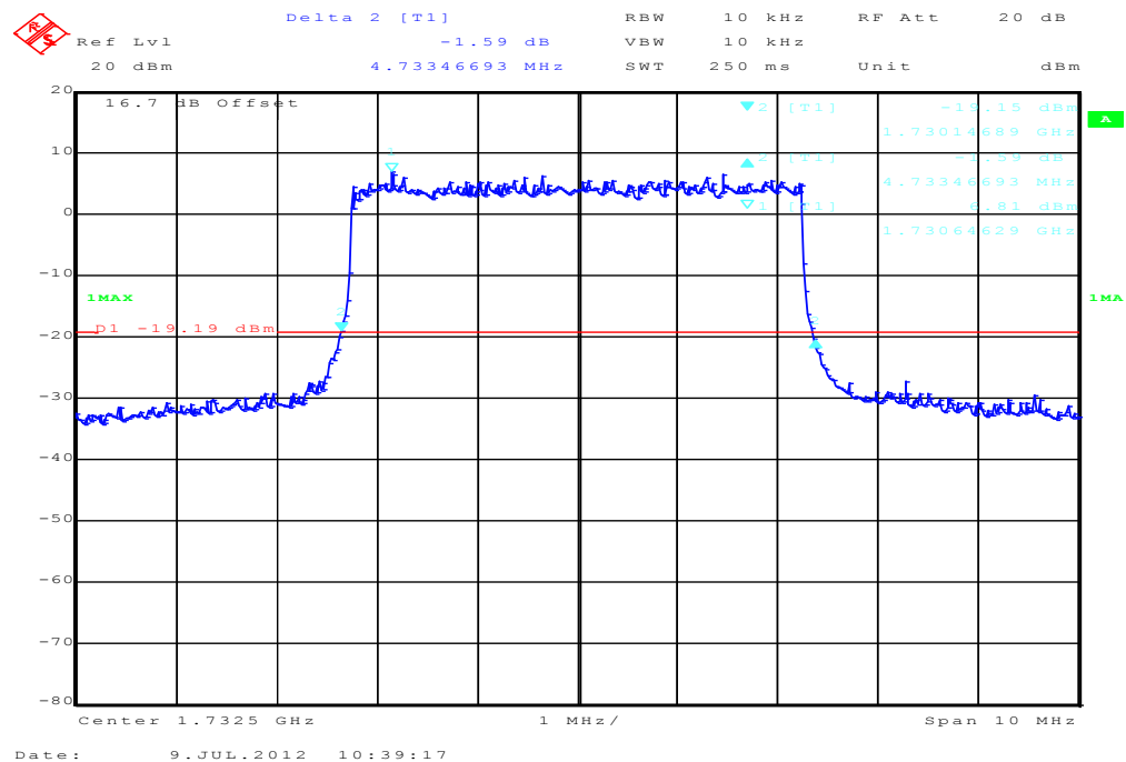
Plot 6: 5 MHz (-26 dBc BW)
