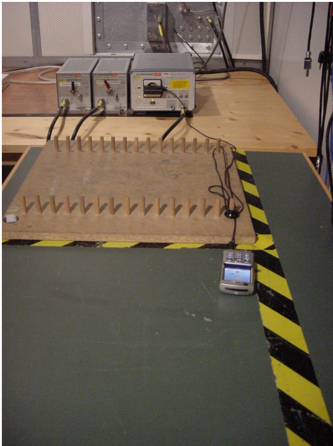
Photo 3 (Conducted Emissions):
