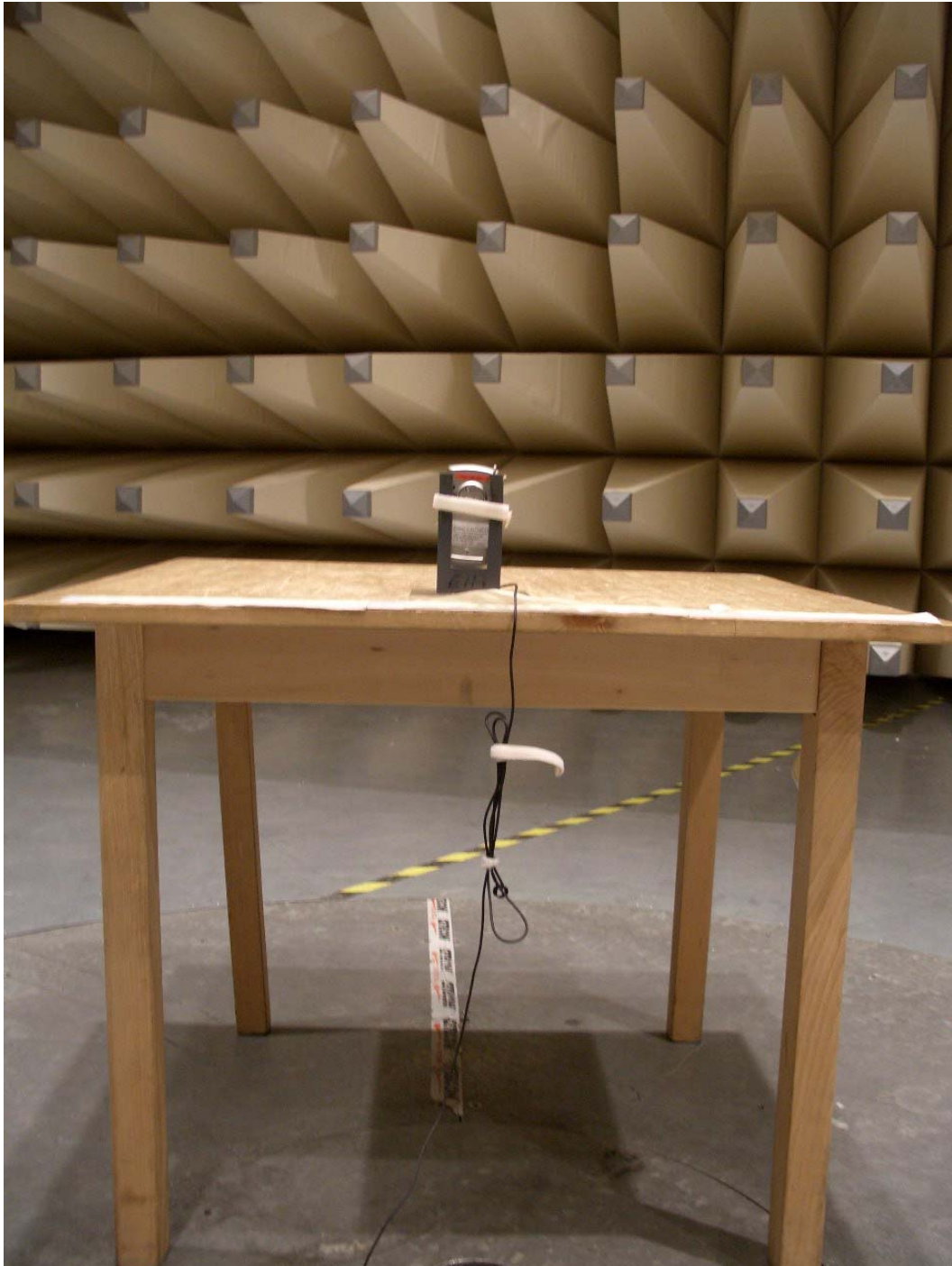
Photo 2 (Radiated Emissions):
