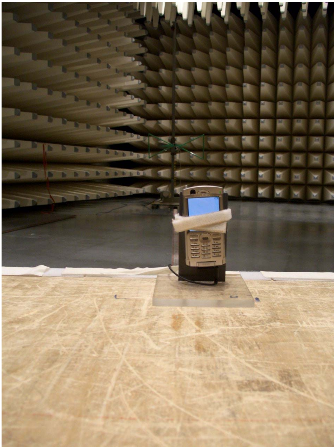
Photo 1 (Radiated Emissions):
