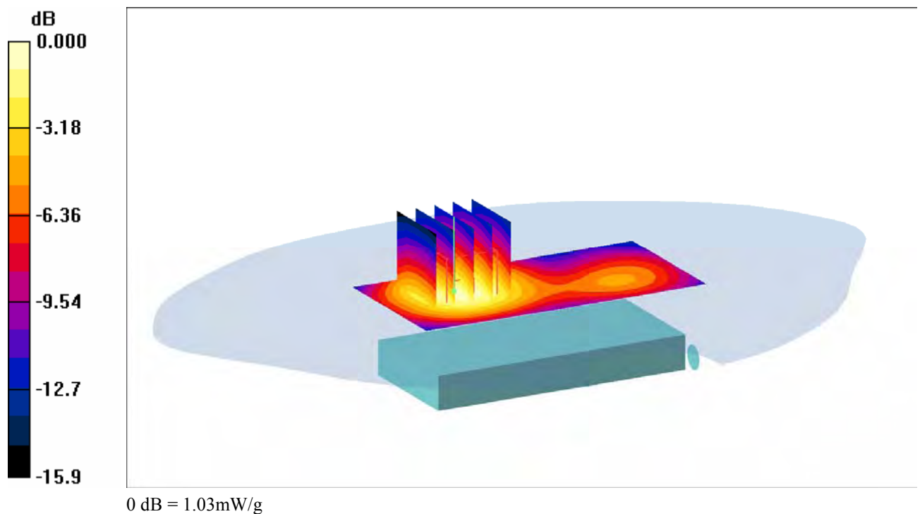
(f) Maximum SAR Distribution for EUT in GPRS(2TS)1900 mode measured with the back of the phone facing the flat section of phantom.
