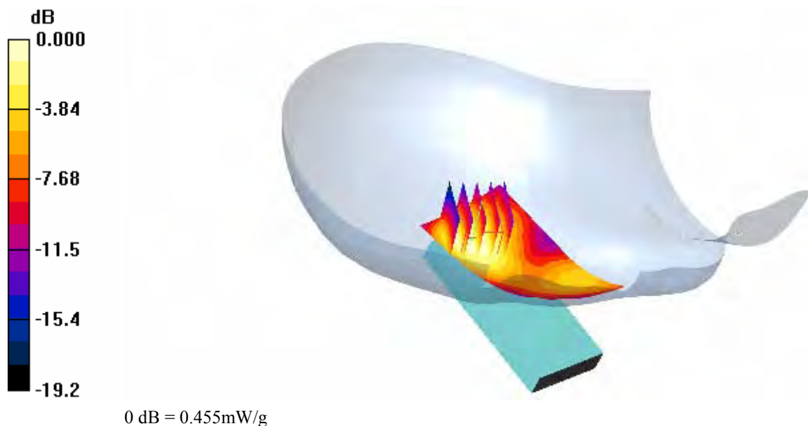
(b) SAR Distribution for EUT in GSM1900 mode measured against the right hand side phantom for the tilt phone position.
