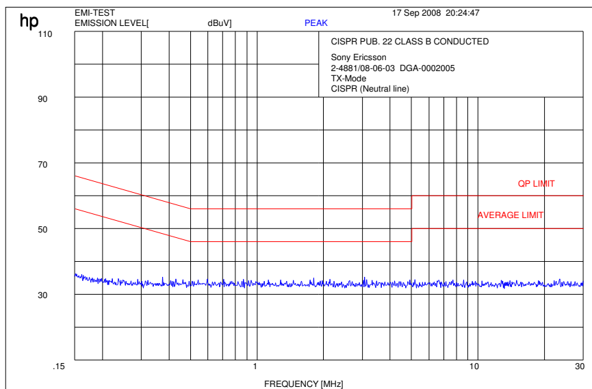
Plot 1: BT Testmode (Neutral line)
