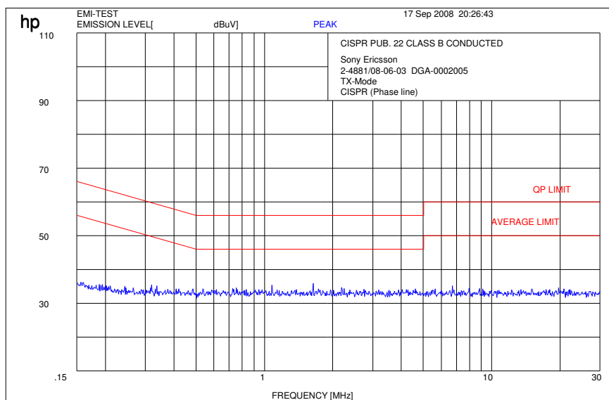
Plot 2: BT Testmode (Phase line)
