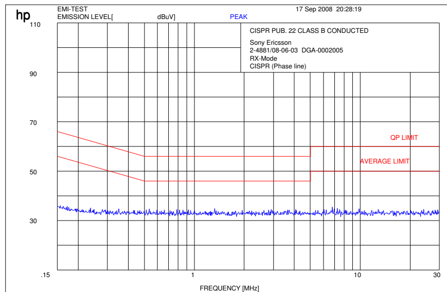
Plot 4: Idle Mode (Phase line)
