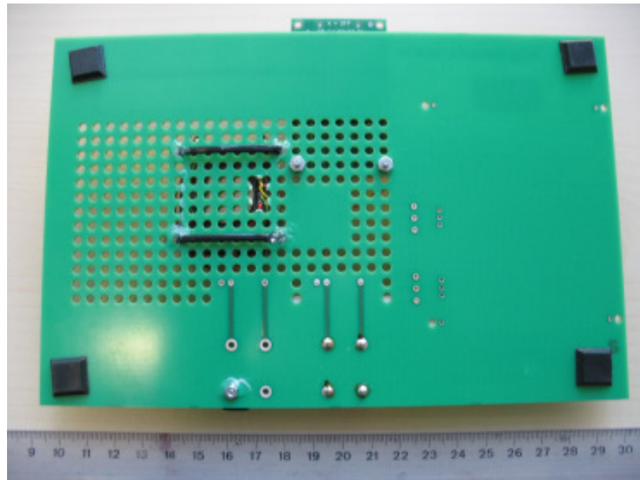
Photo 3: EUT mounted on a test board
