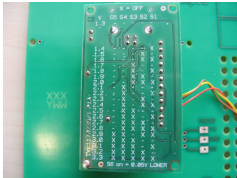
Photo 6: EUT mounted on a test board
