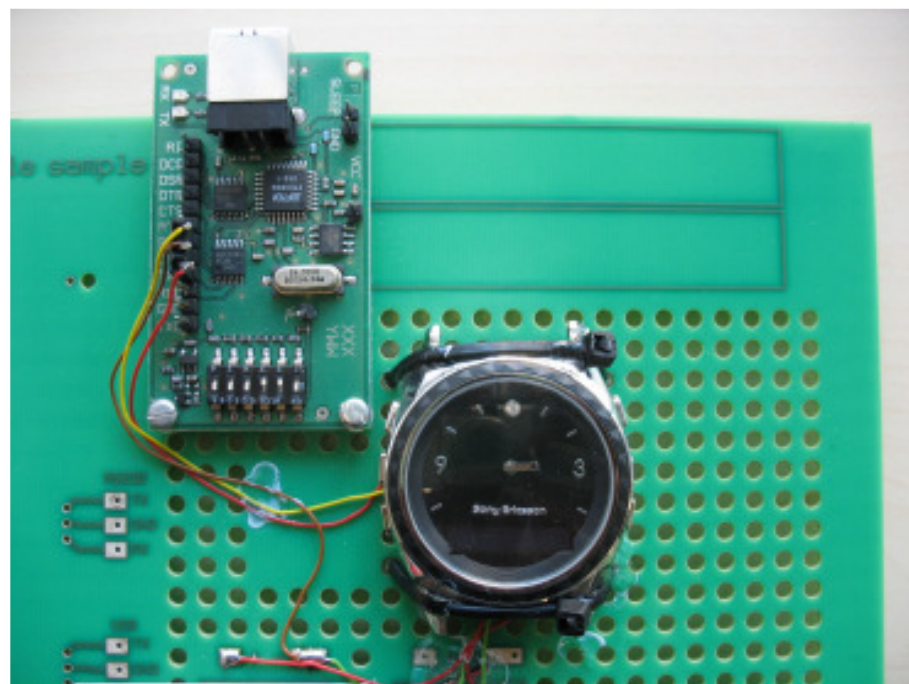
Photo 4: EUT mounted on a test board
