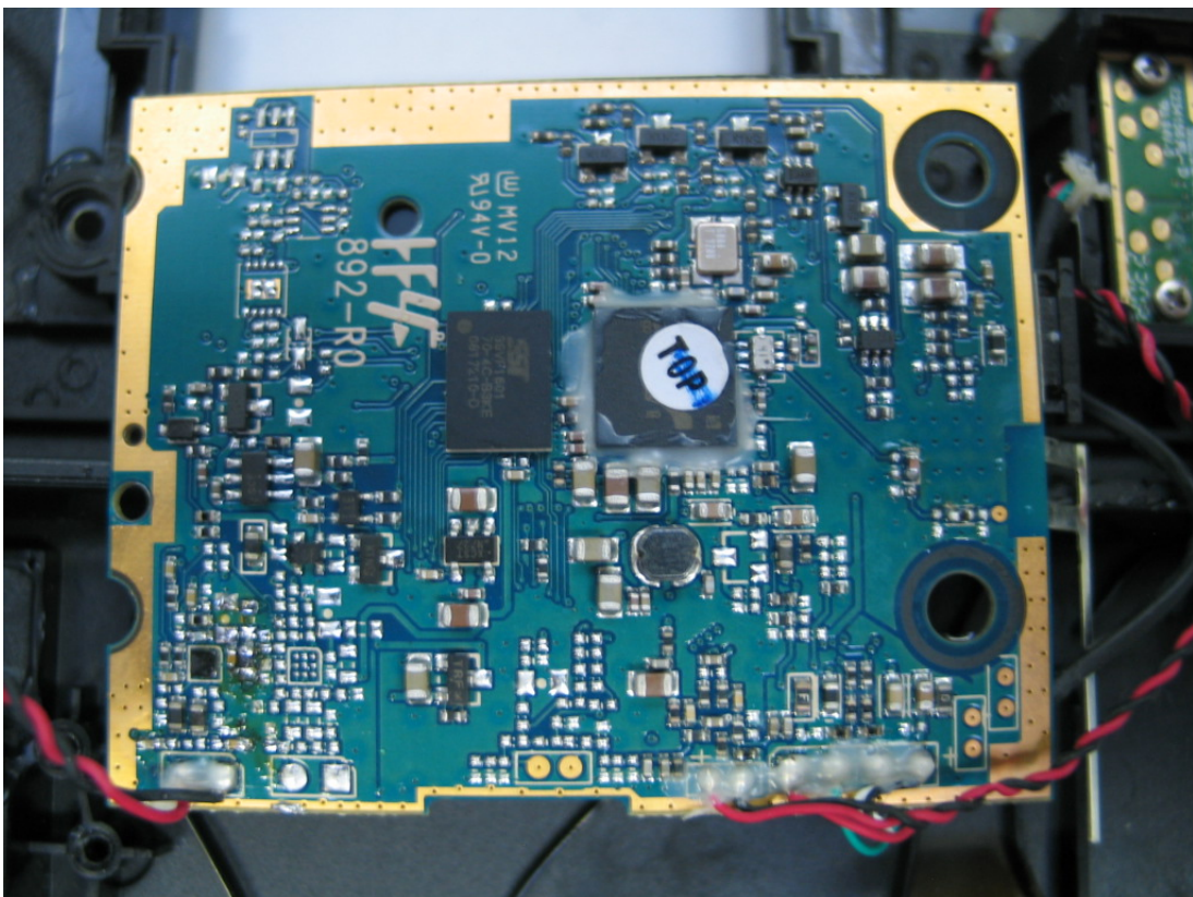
Photo 8: EUT (top side of PCB, detail view)
