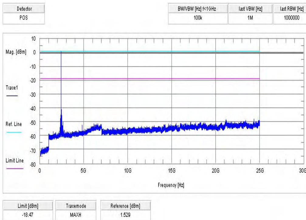
Plot 1 of 3: lowest channel
