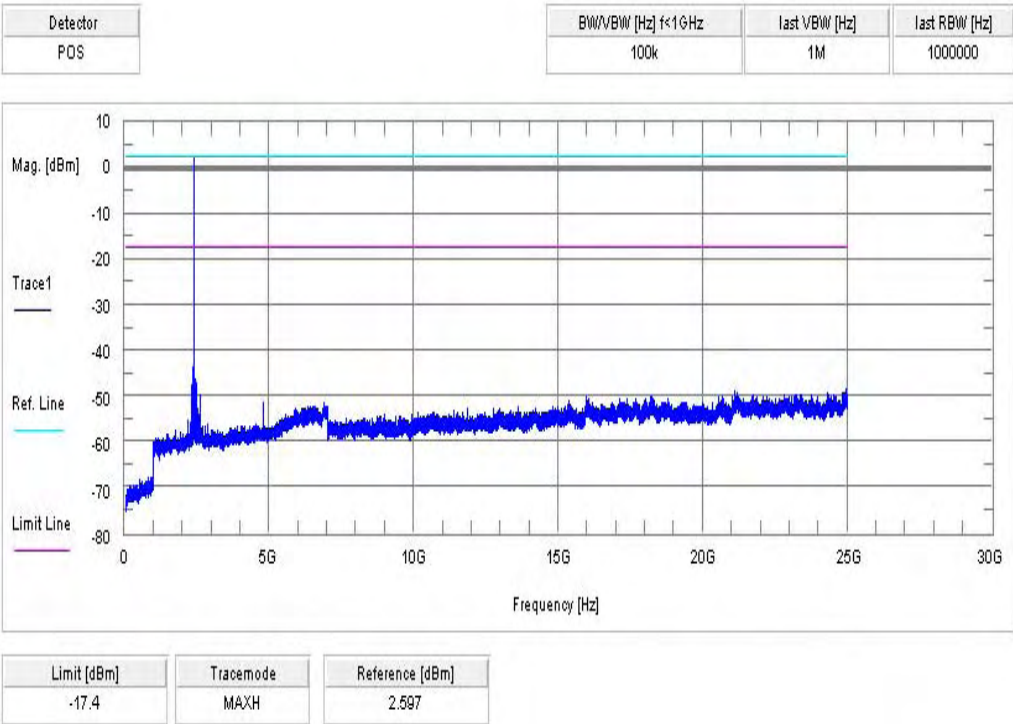
Plot 1 of 3: lowest channel
