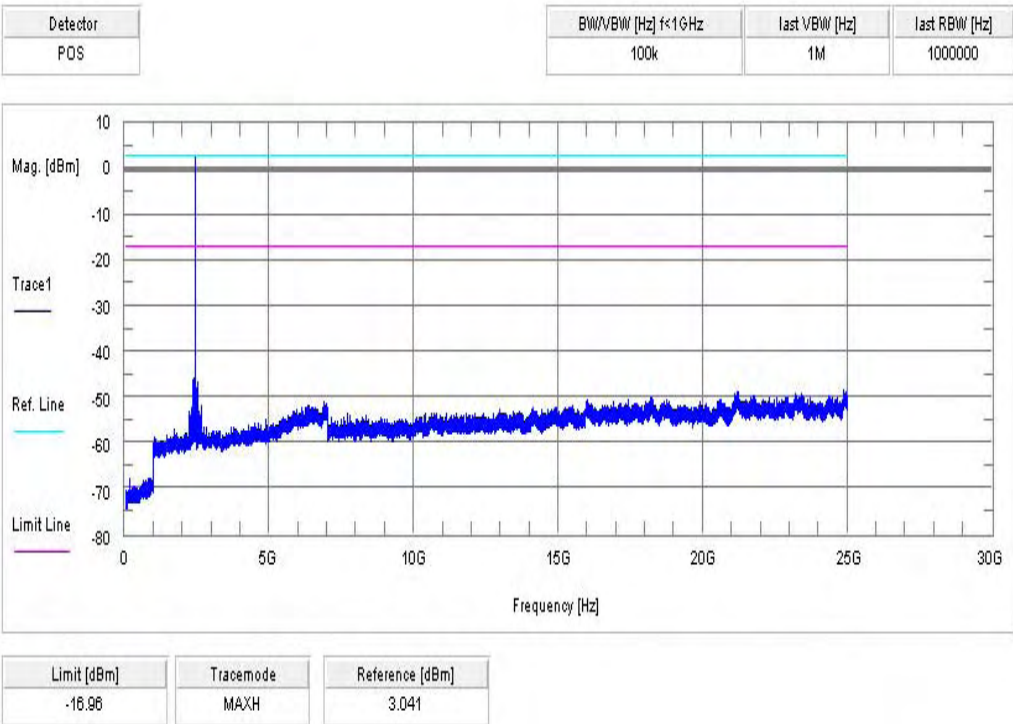
Plot 2 of 3: middle channel
