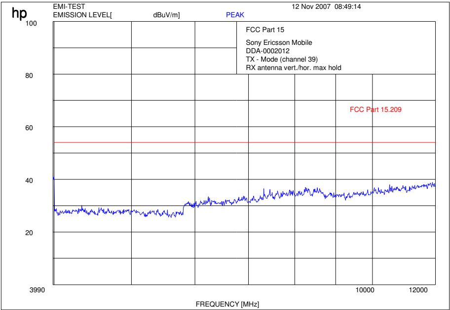
Plot 7: 4 - 12 GHz vertical/horizontal (middle channel)
