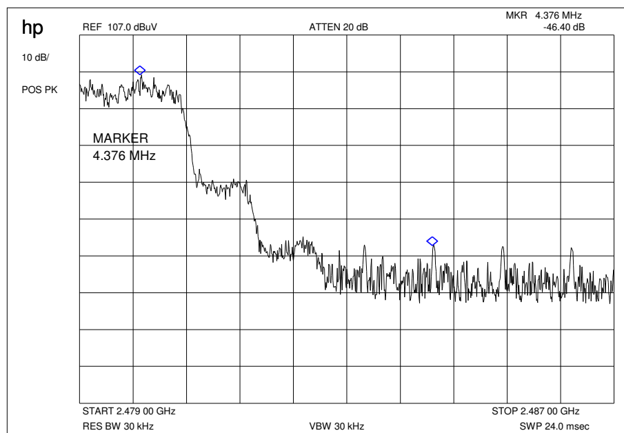
Plot 3: Marker-Delta Method (hopping)
