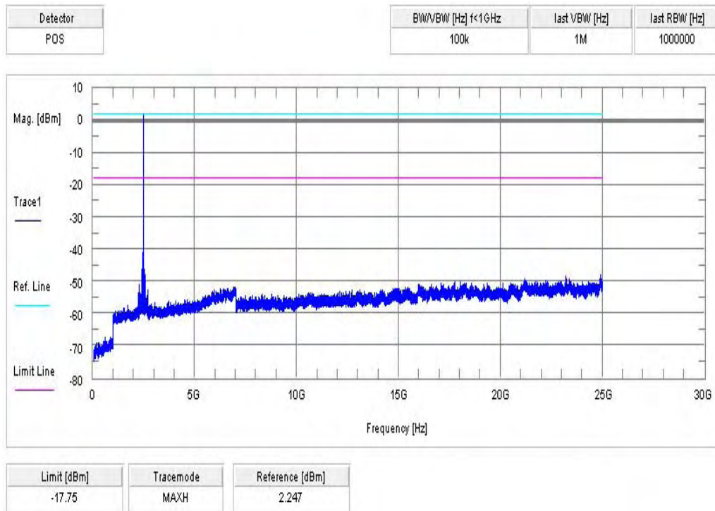
Plot 3 of 3: highest channel
