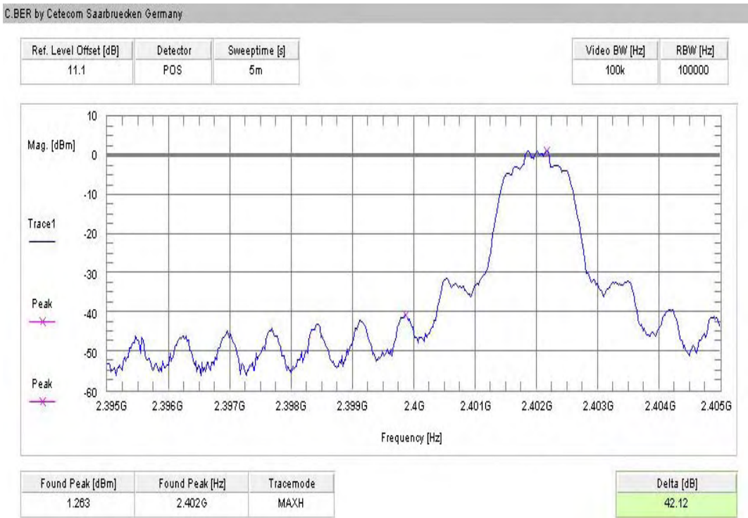
Plot 1 of 4 (hopping off, lowest frequency):
