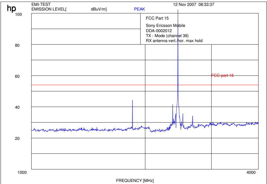
Plot 6: 1 - 4 GHz vertical/horizontal (middle channel)
