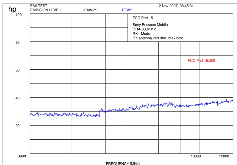
Plot 3: 4 - 12 GHz vertical/horizontal (receiver)
