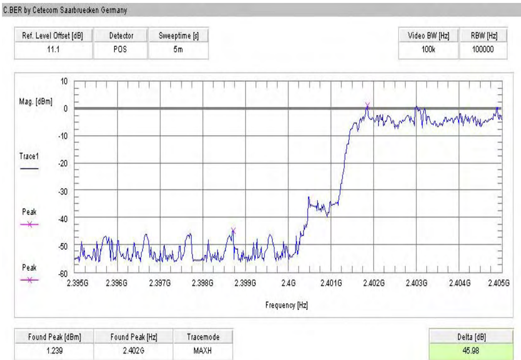
Plot 2 of 4 (hopping on, lowest frequency):
