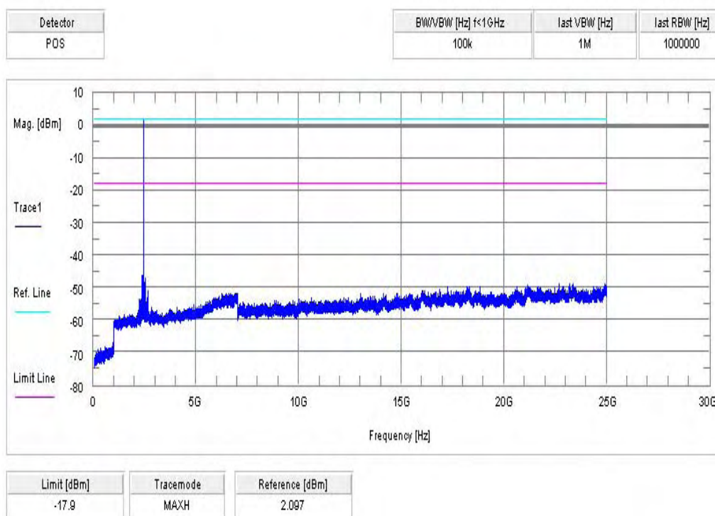
Plot 2 of 3: middle channel
