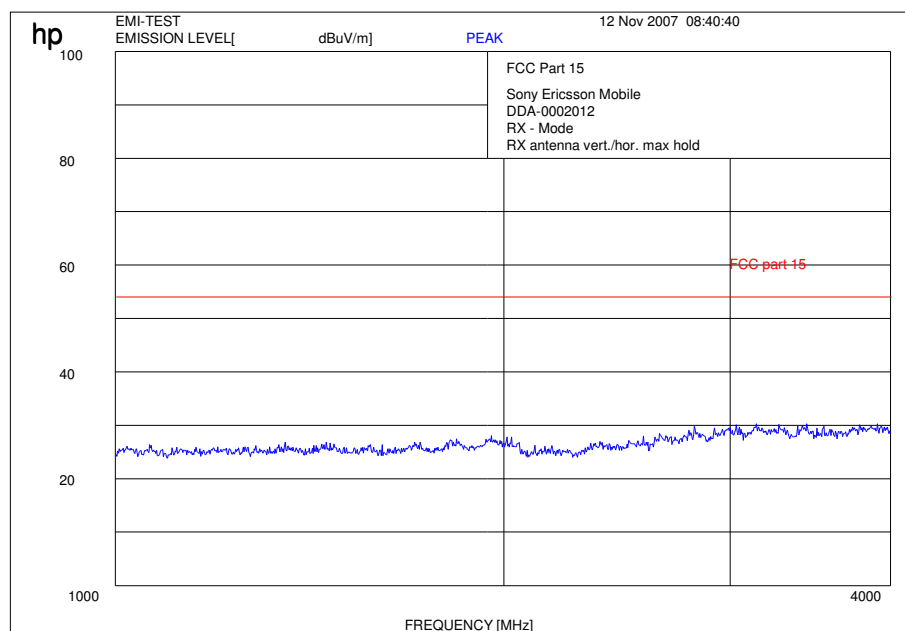
Plot 2: 1 - 4 GHz vertical/horizontal (receiver)
