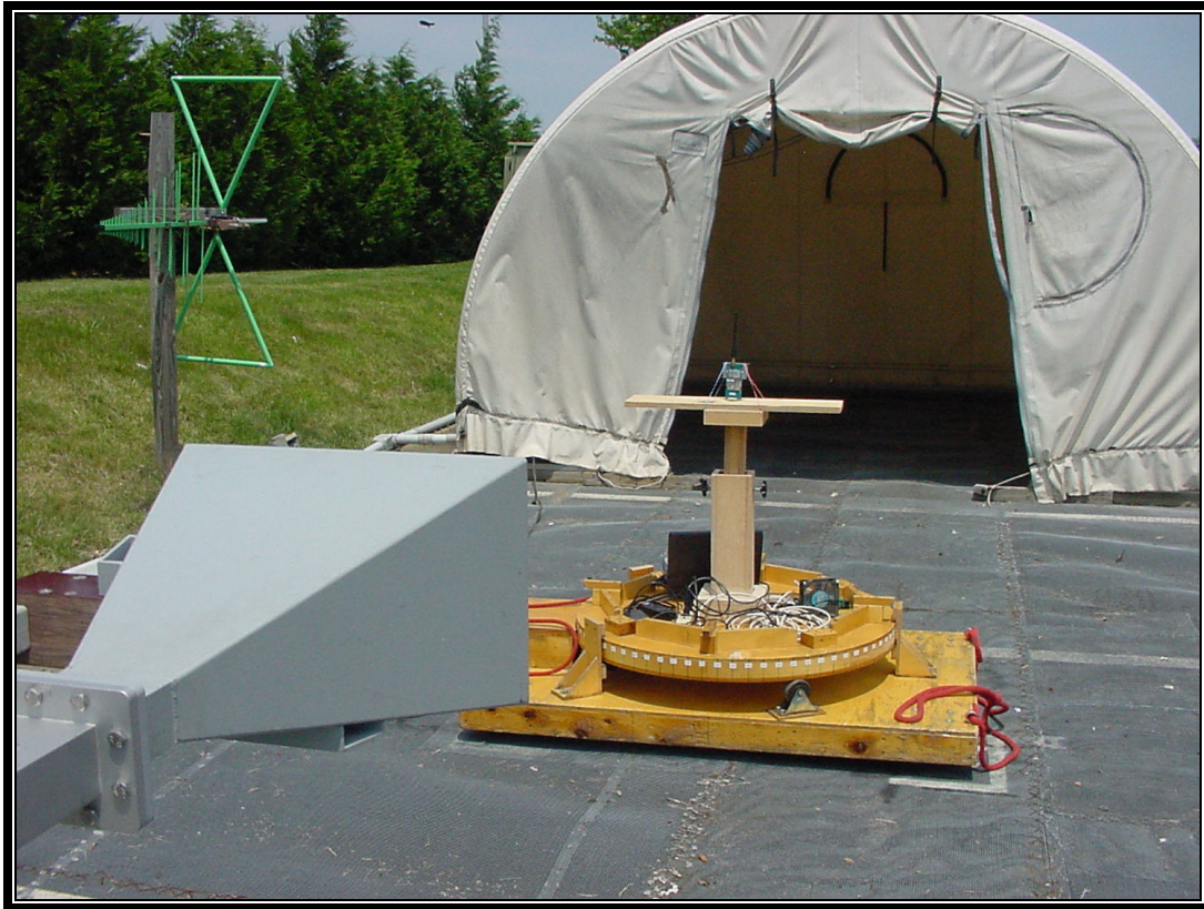
PHOTOGRAPH 3: RADIATED EMISSIONS – FRONT VIEW
