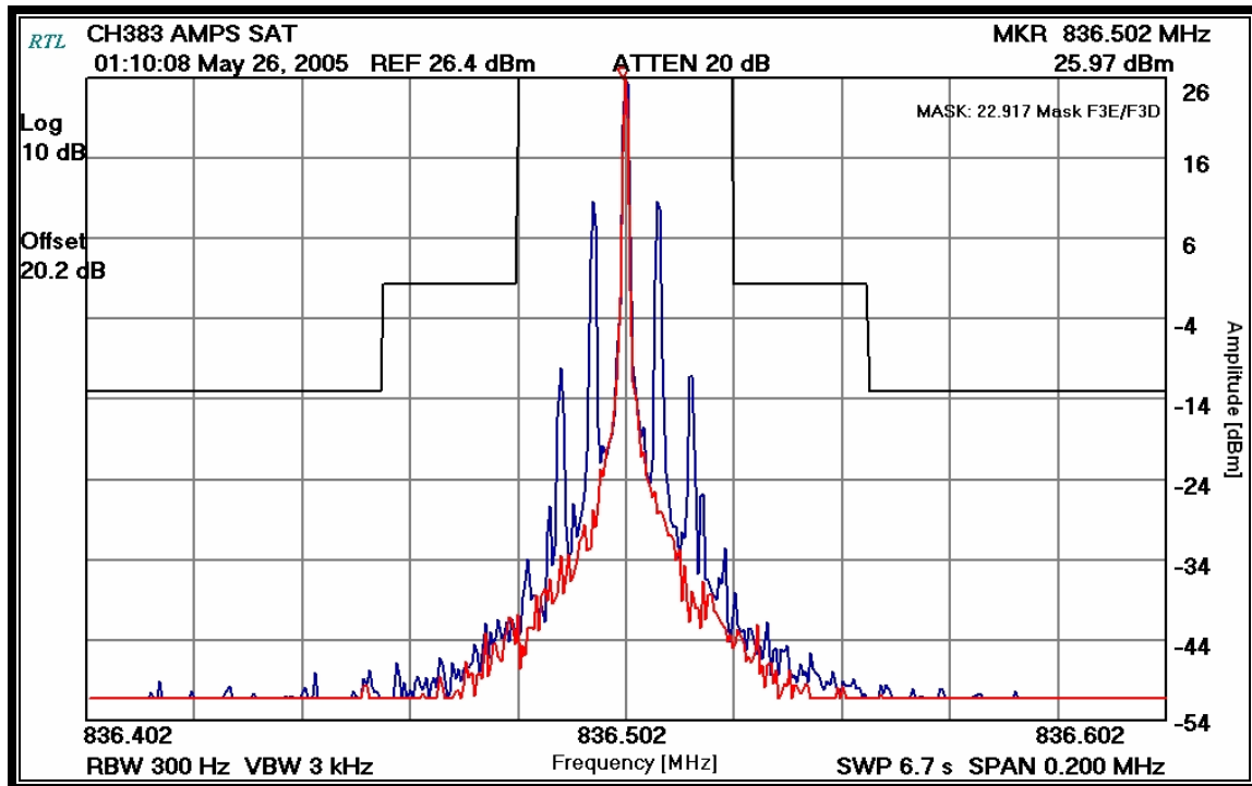
PLOT 7-3: OCCUPIED BANDWIDTH: AMPS SAT - (MASK 22.917)
