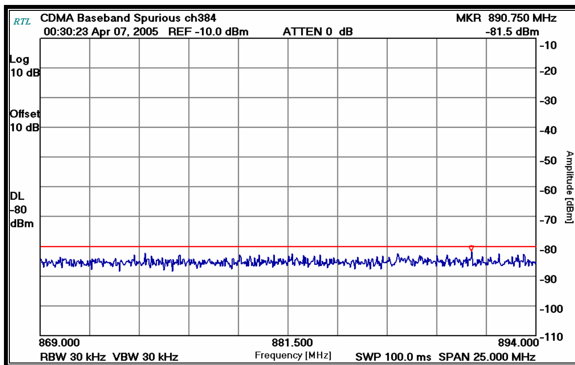
PLOT 8-2: MOBILE EMISSIONS IN BASE FREQUENCY RANGE – CDMA CH 384
