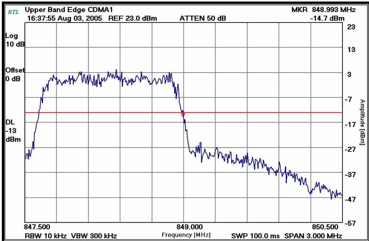
PLOT 7-9: UPPER BAND EDGE – CDMA 800 BAND
