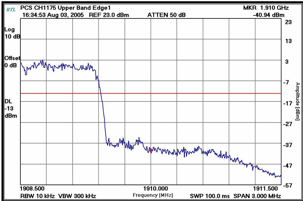
PLOT 7-11: UPPER BAND EDGE – CDMA PCS 1900 BAND
