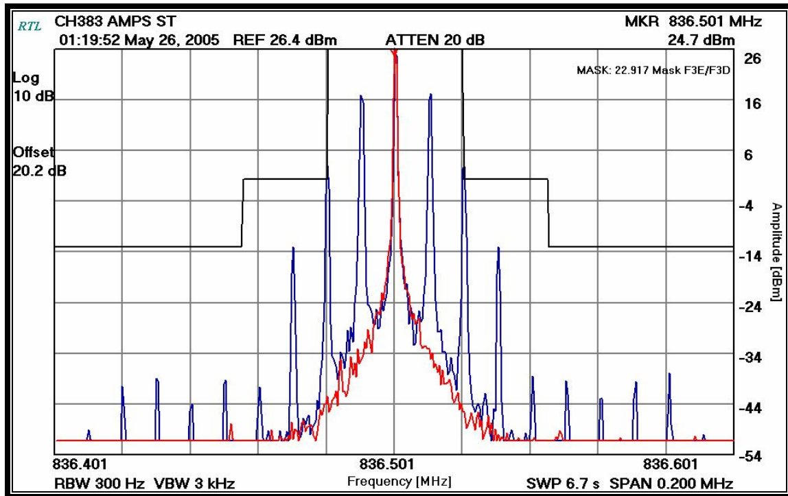
PLOT 7-4: OCCUPIED BANDWIDTH: AMPS ST - (MASK 22.917)
