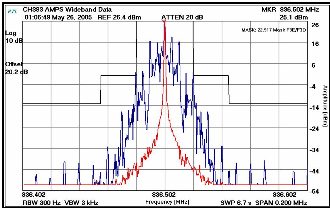
PLOT 7-1: 40 KHZ CHANNEL BANDWIDTH – WIDEBAND DATA 836.49 MHZ
