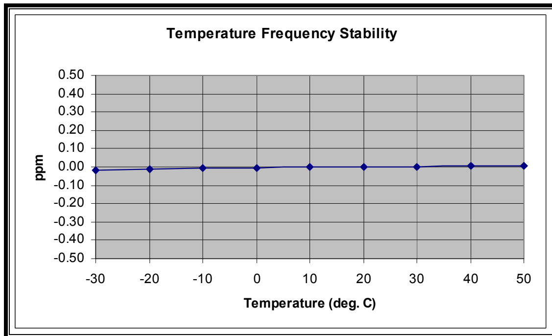
PLOT 10-1: TEMPERATURE FREQUENCY STABILITY
