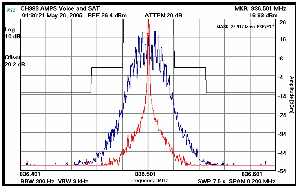
PLOT 7-2: OCCUPIED BANDWIDTH: AMPS VOICE/SAT - (MASK 22.917)
