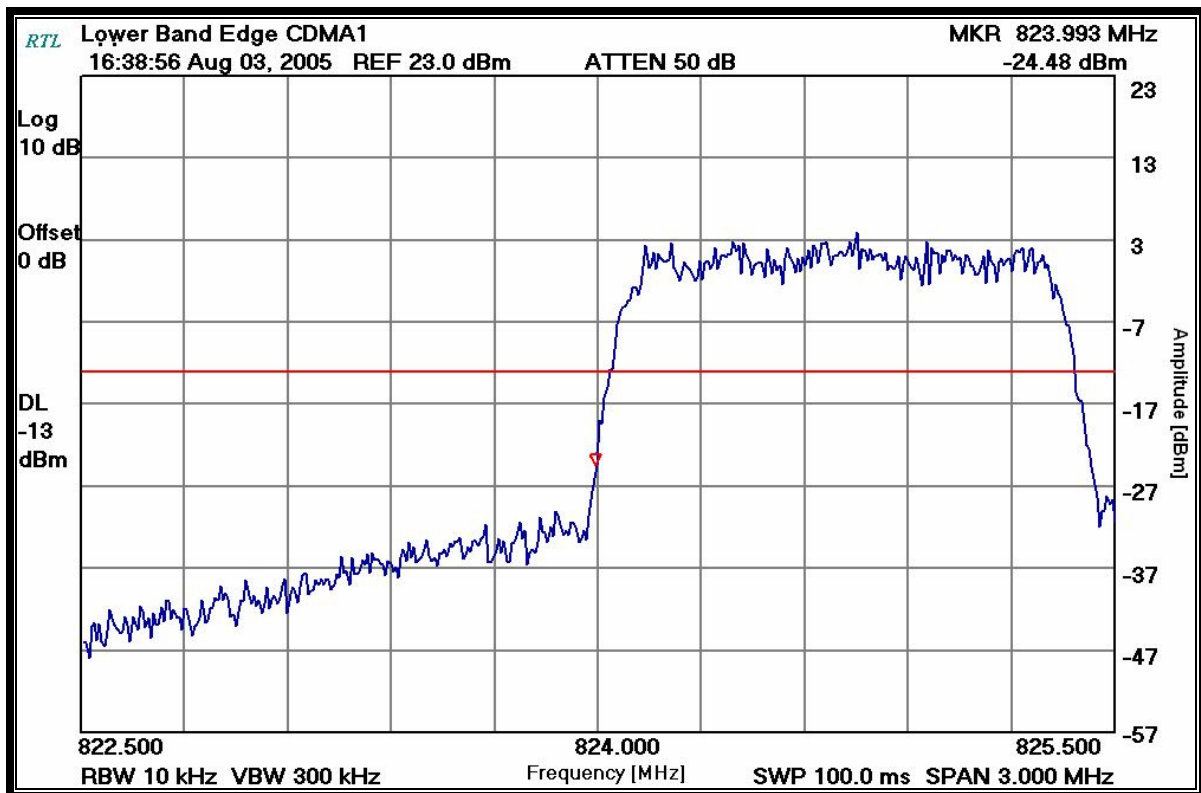
PLOT 7-8: LOWER BAND EDGE – CDMA 800 BAND
