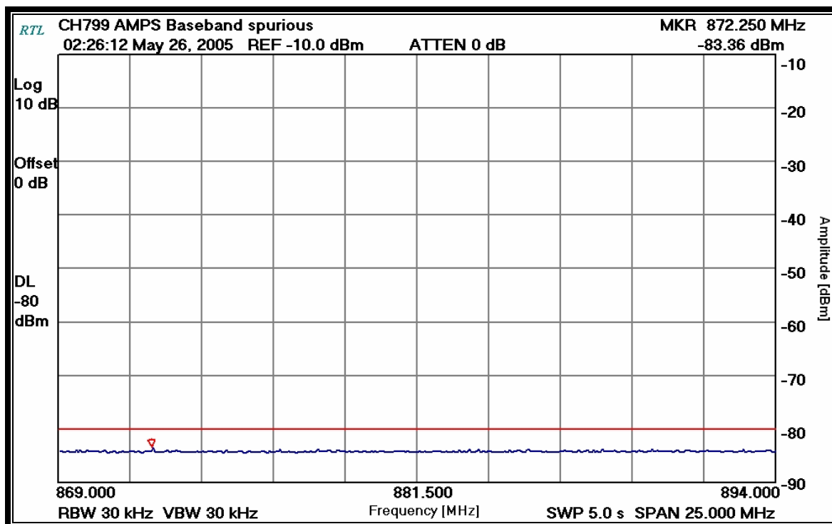
PLOT 8-1: MOBILE EMISSIONS IN BASE FREQUENCY RANGE – AMPS CH 799
