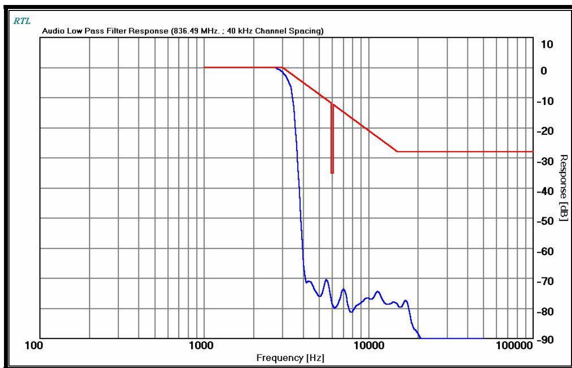
PLOT 11-1: MODULATION CHARACTERISTICS – AUDIO LOW PASS FILTER
