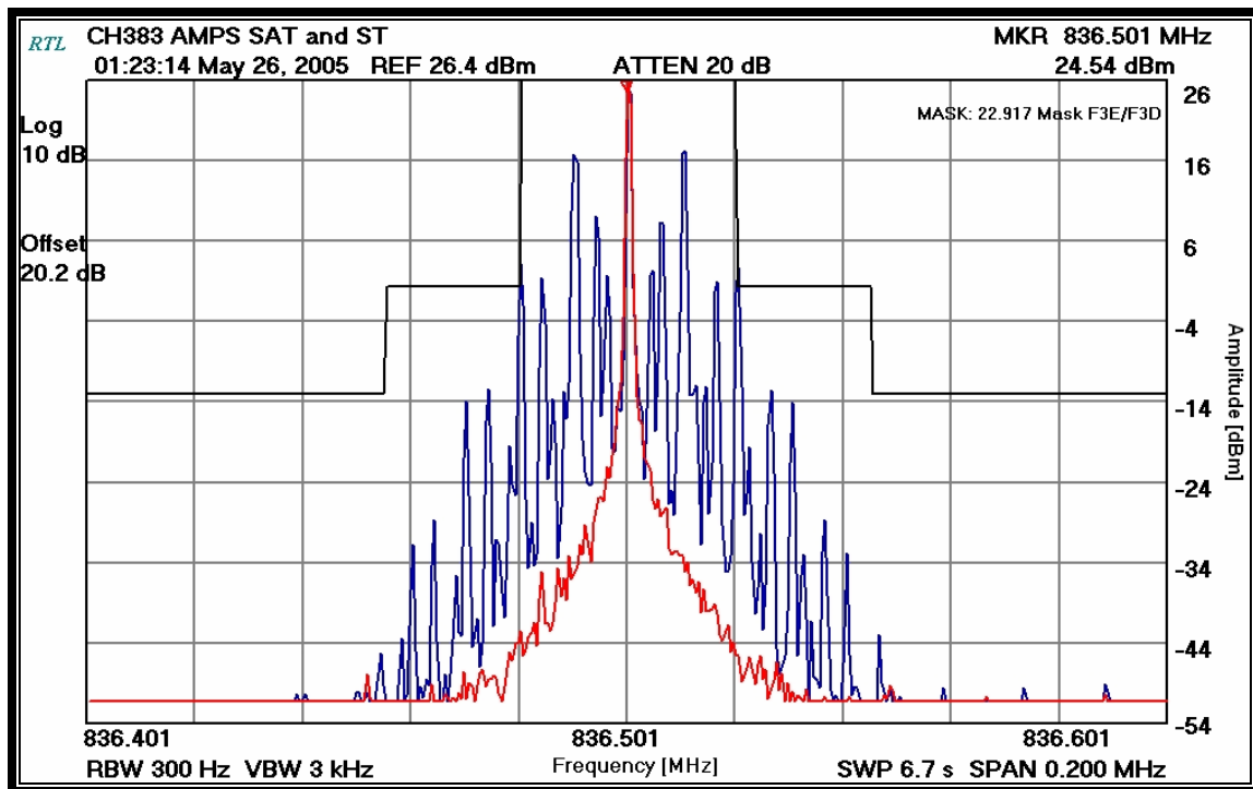
PLOT 7-5: OCCUPIED BANDWIDTH: AMPS SAT/ST - (MASK 22.917)
