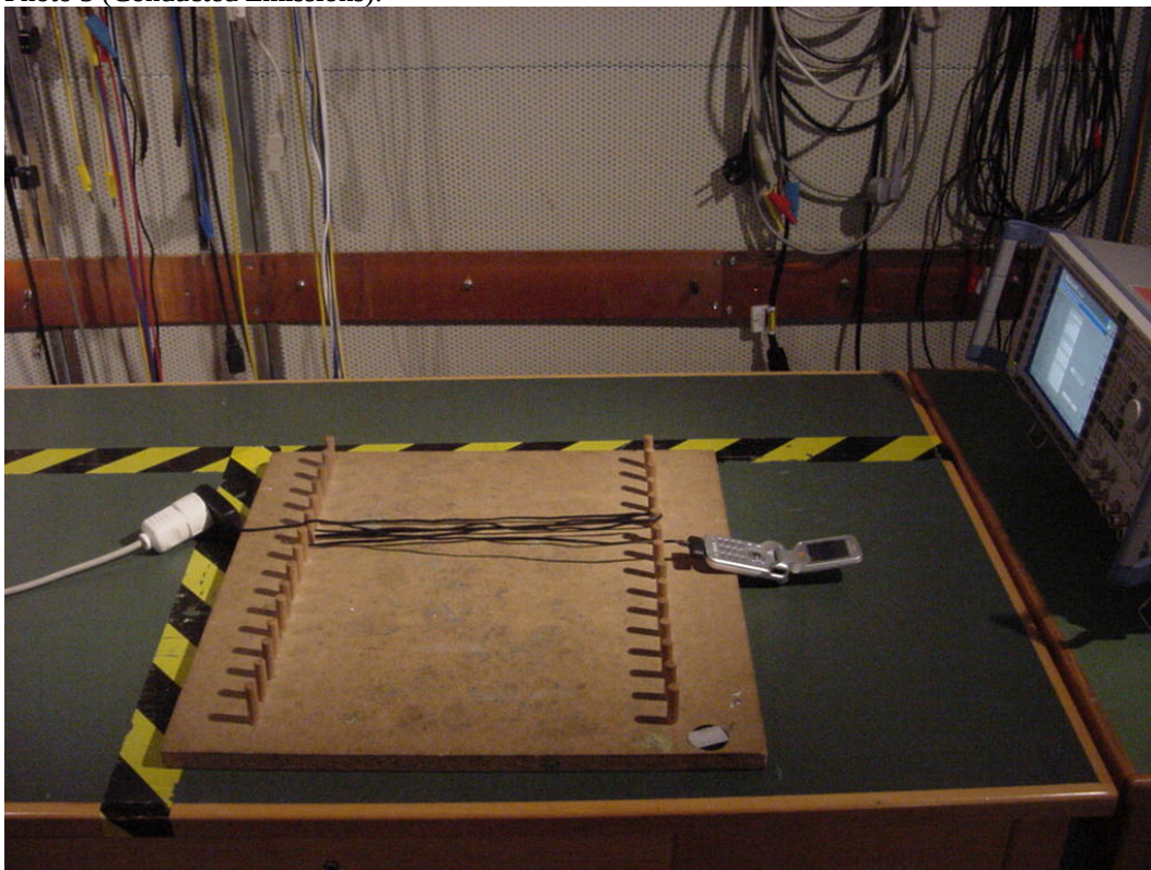
Photo 3 (Conducted Emissions):
