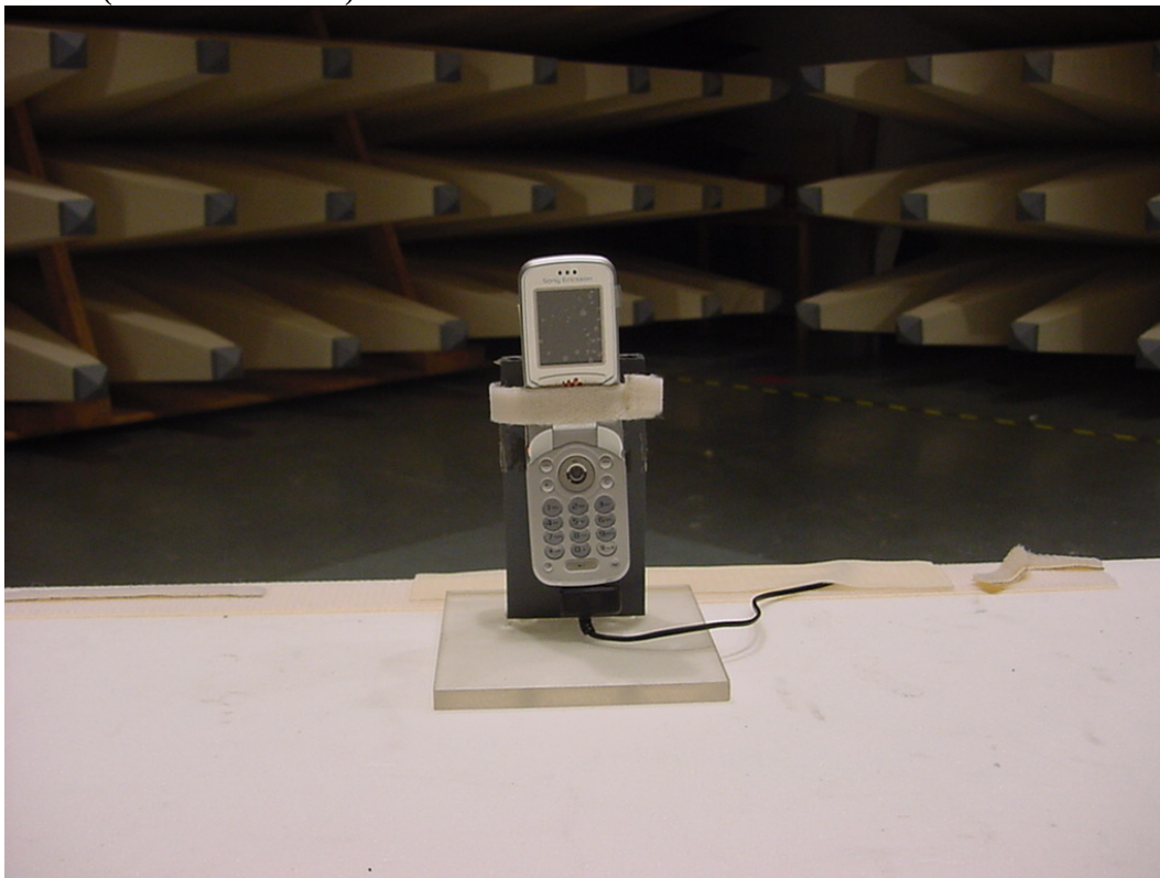
Photo 2 (Radiated Emissions):
