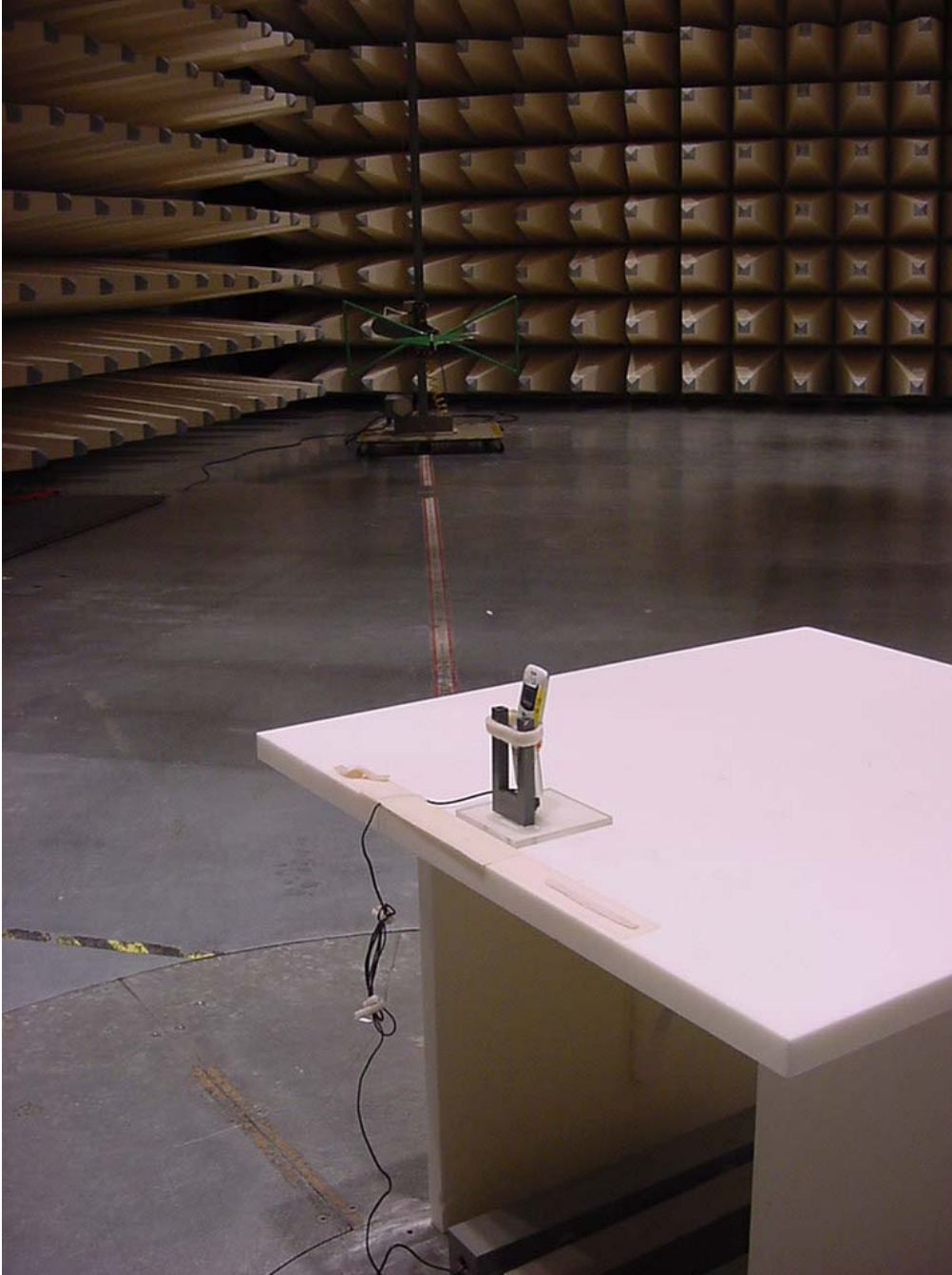
Photo 1 (Radiated Emissions):
