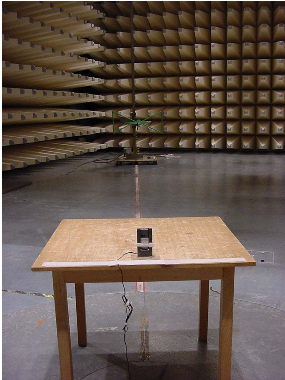
Photo 1: Radiated Emissions
