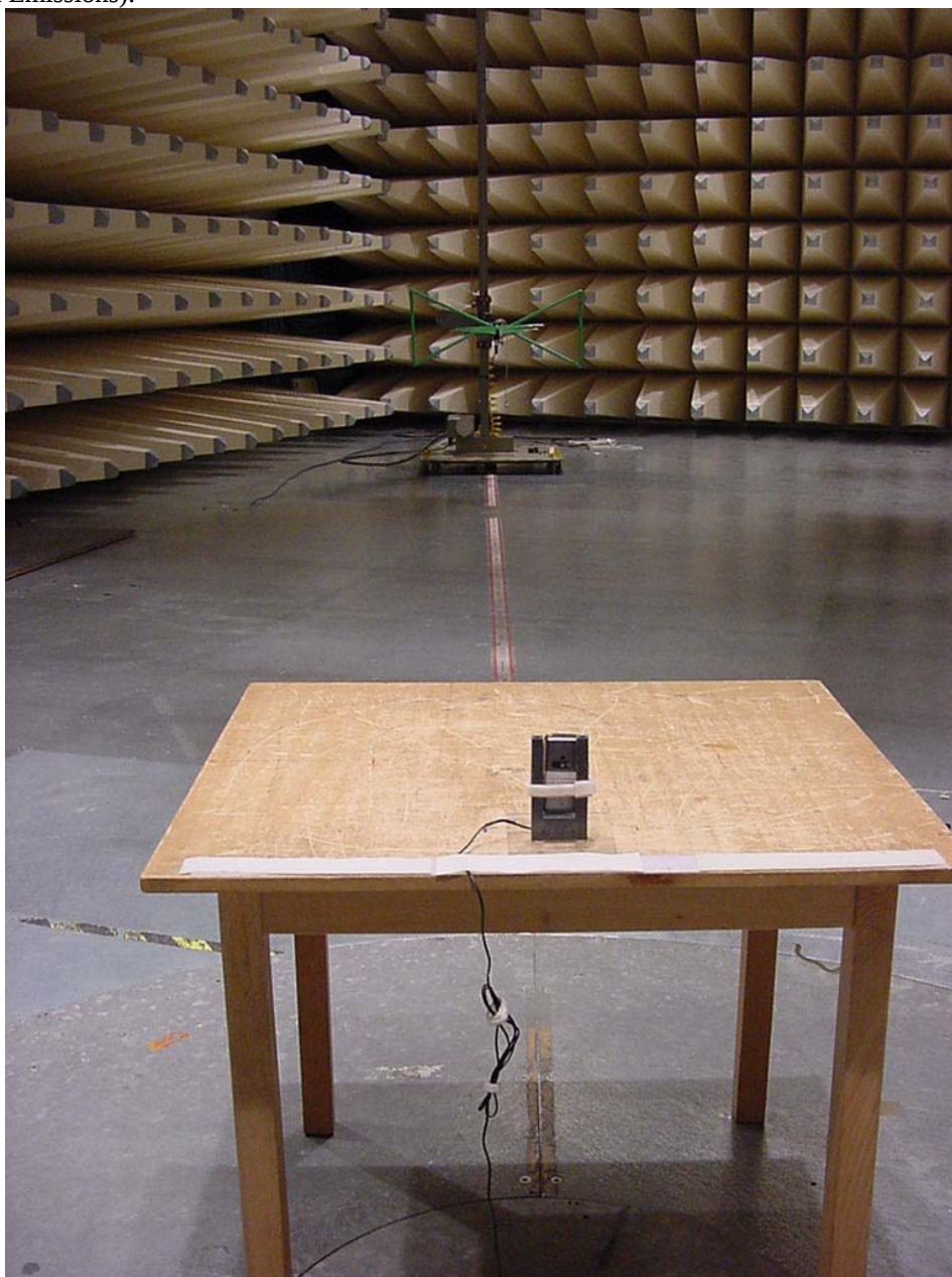
Photo 1 (Radiated Emissions):
