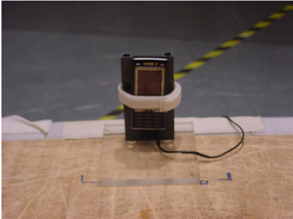
Photo 3 (Radiated Emissions):
