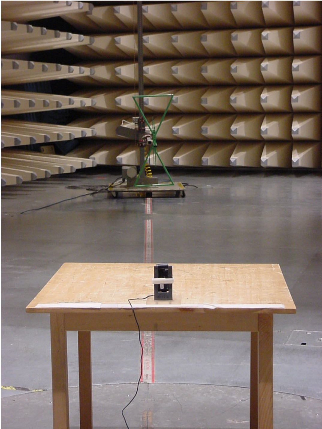
Photo 1 (Radiated Emissions):
