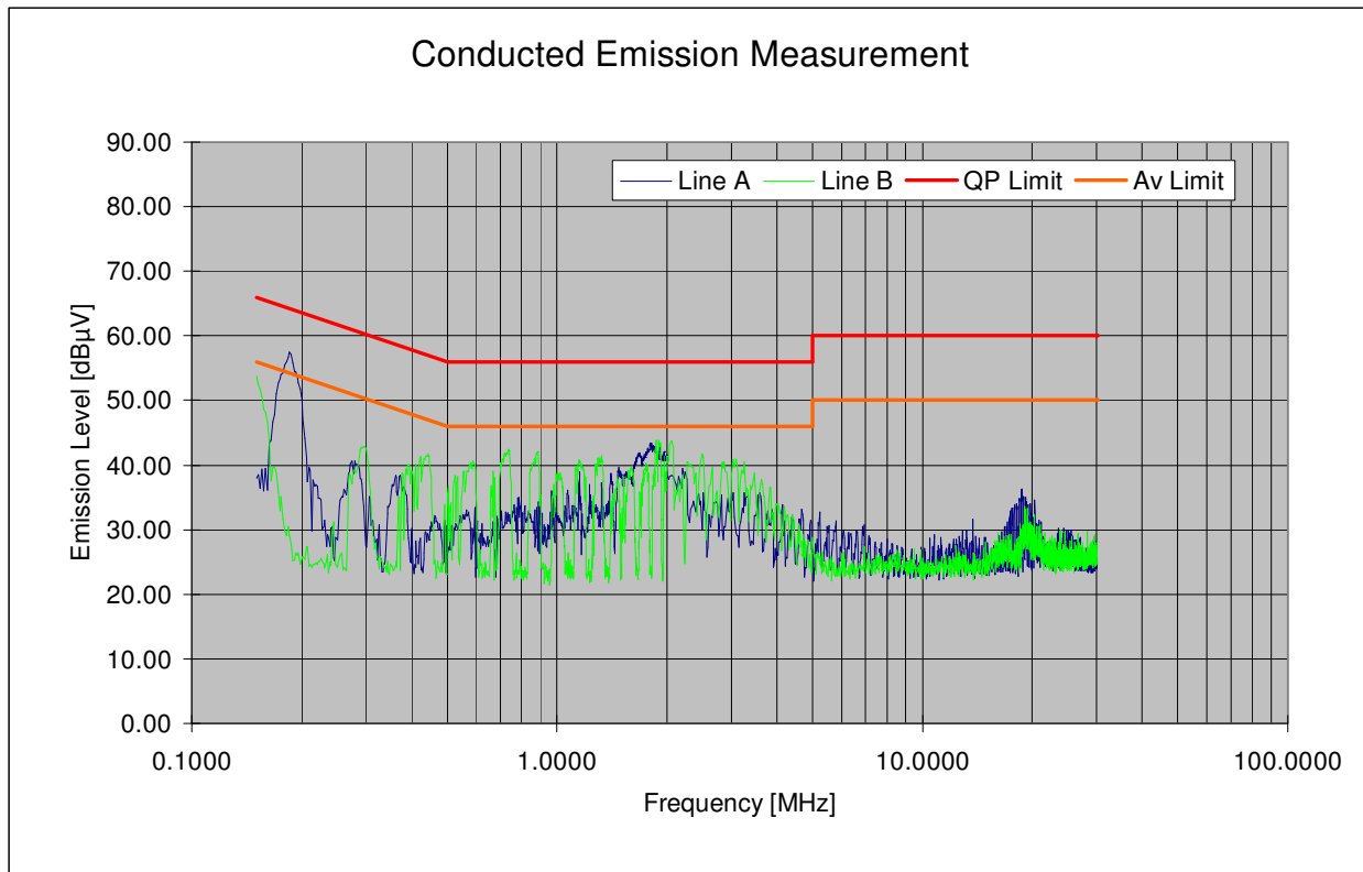
Plot 7-1. Line-Conducted Test Plot
