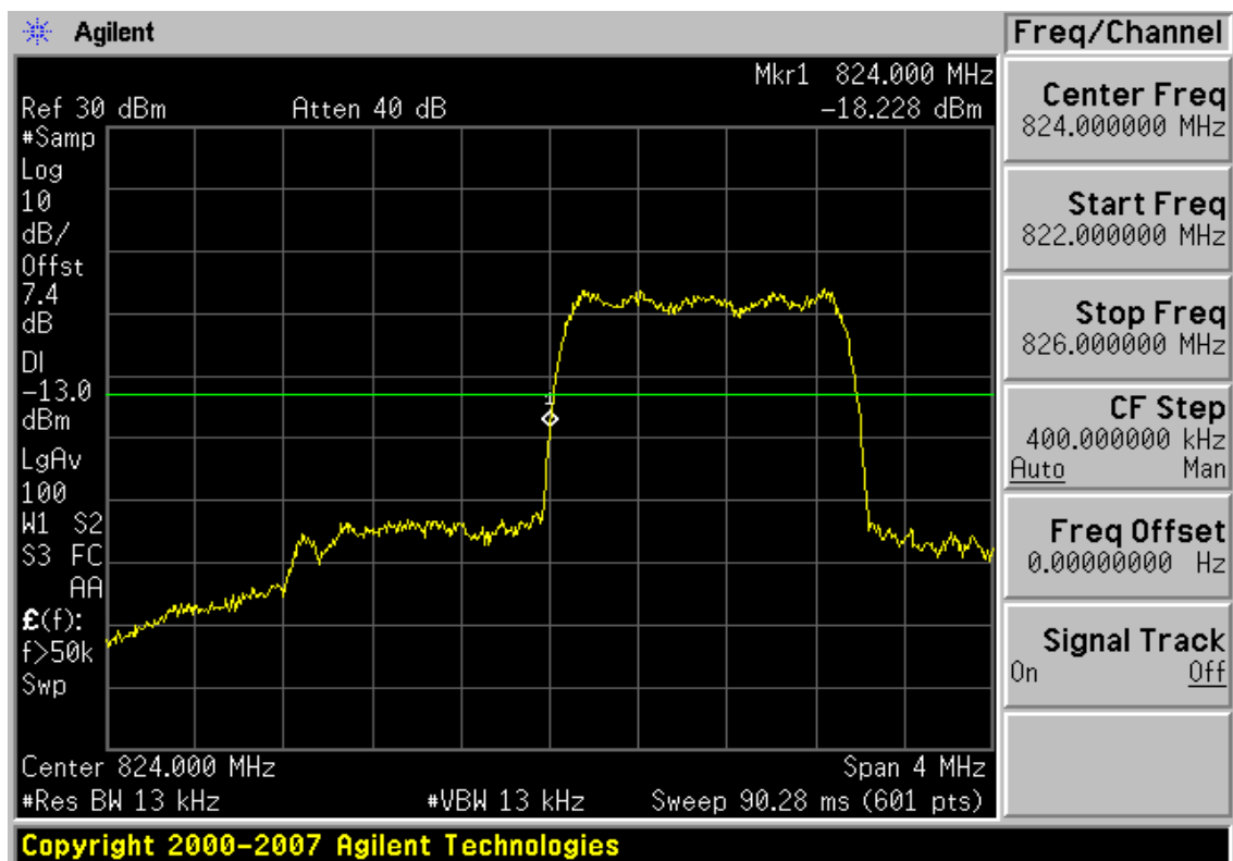
Plot 7-13. Band Edge Plot (Cellular CDMA Mode – Ch. 1013)
