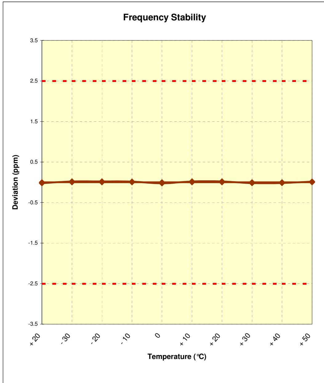
Plot 6-1. Frequency Stability Graph (Cellular CDMA Mode – Ch. 384)
