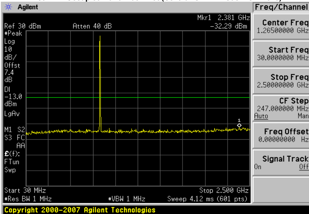
Plot 7-18. Conducted Spurious Plot (Cellular CDMA Mode – Ch. 777)
