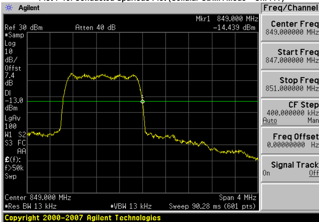
Plot 7-20. Band Edge Plot (Cellular CDMA Mode – Ch. 777)
