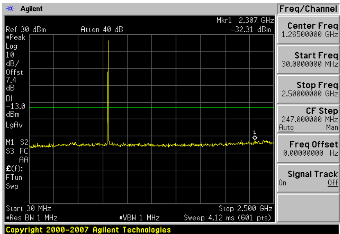
Plot 7-11. Conducted Spurious Plot (Cellular CDMA Mode – Ch. 1013)
