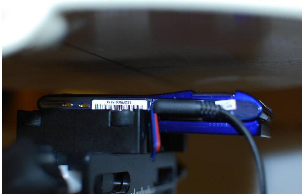
Figure 19-9 SAR Test Setup Photo 9
