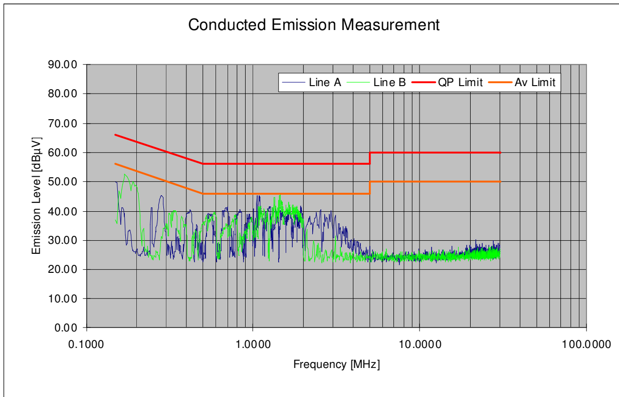
Plot 6-18. Line Conducted Plot with Bluetooth
