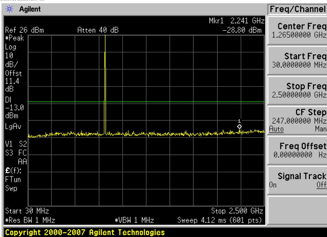
Plot 7-15. Conducted Spurious Plot (Cellular CDMA Mode – Ch. 384)
