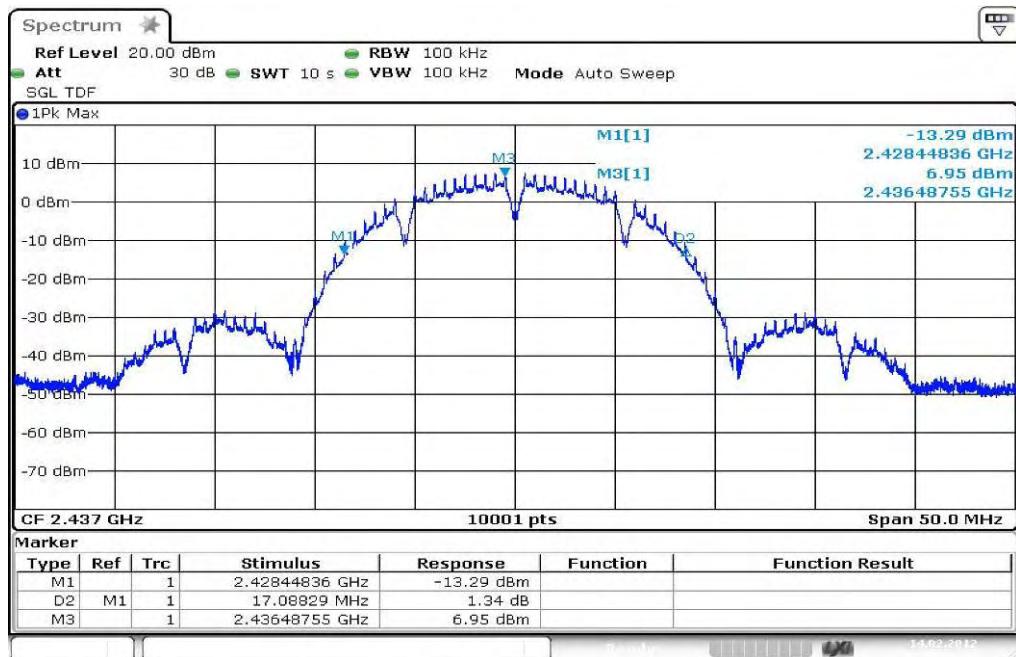
Plot 2: TX mode, middle channel, 20 dB bandwidth
