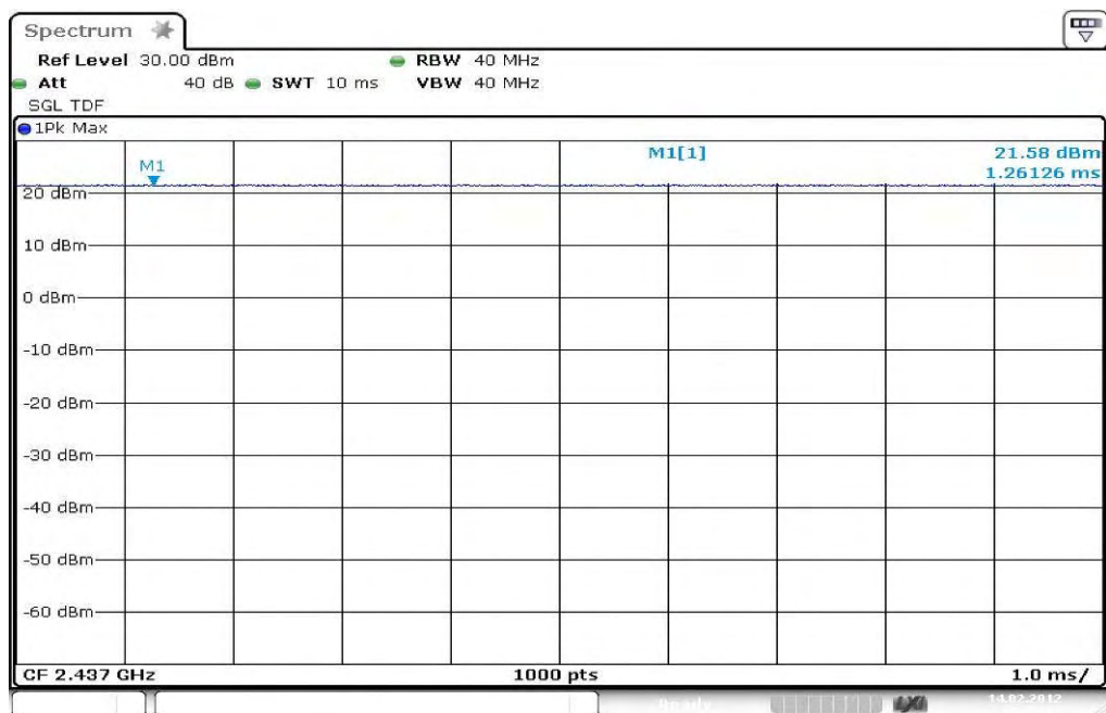
Plot 5: TX mode, middle channel, MCS4
