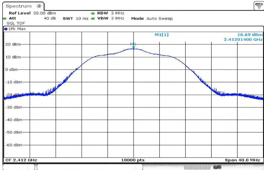
Plot 1: lowest channel, conducted
