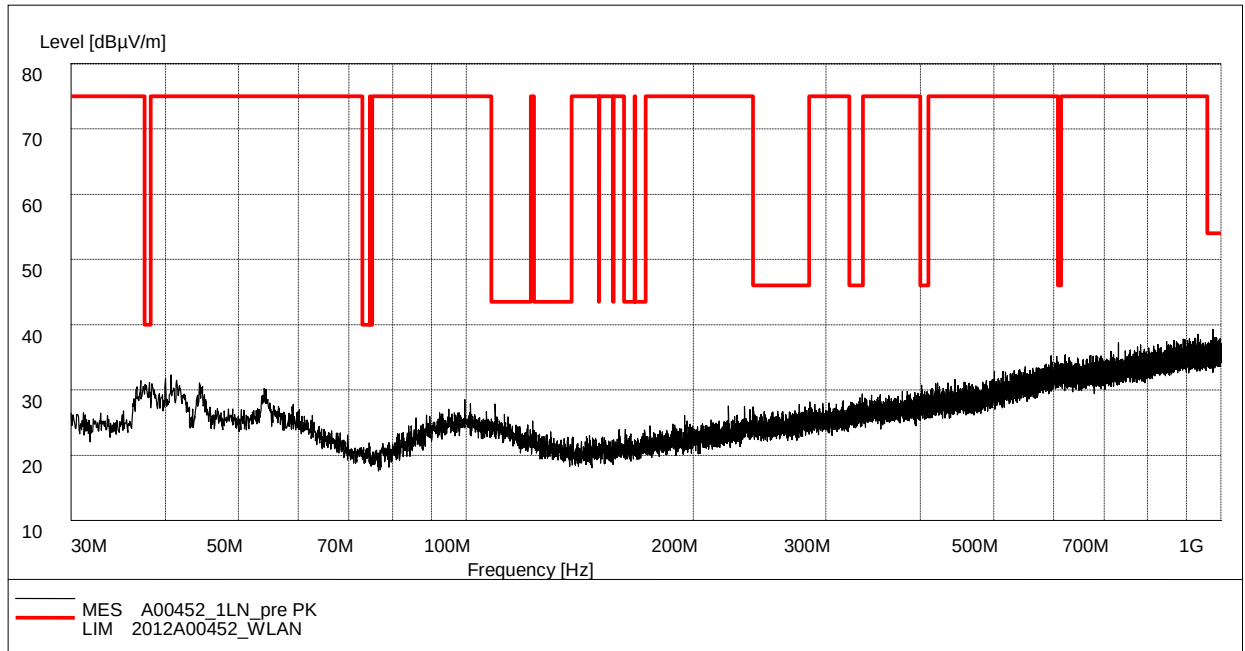
Fig. 66 Radiated Spurious Emission (802.11n-HT20, Ch1, 30 MHz-1 GHz)
