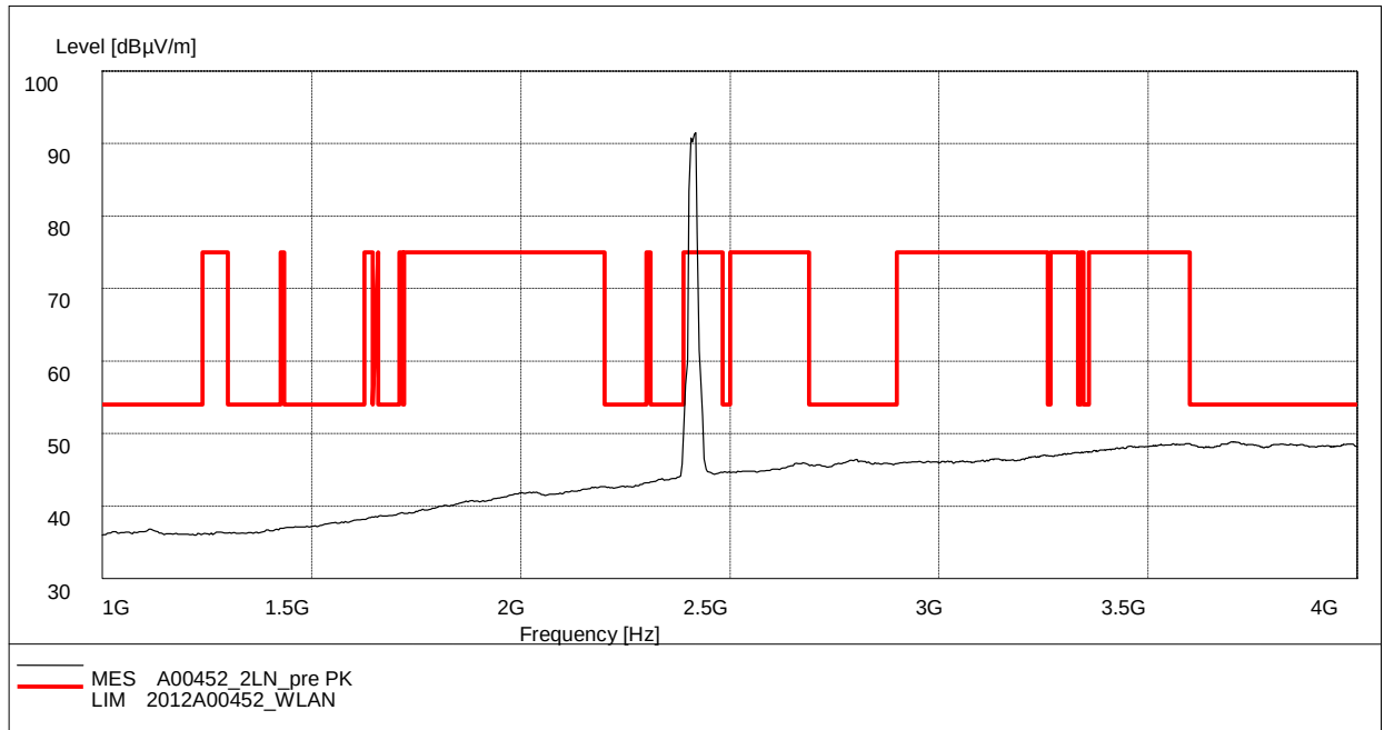
Fig. 67 Radiated Spurious Emission (802.11n-HT20, Ch1, 1 GHz-4 GHz)
