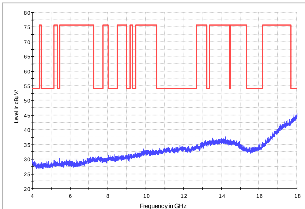
Fig. 68 Radiated Spurious Emission (802.11n-HT20, Ch1, 4 GHz-18 GHz)
