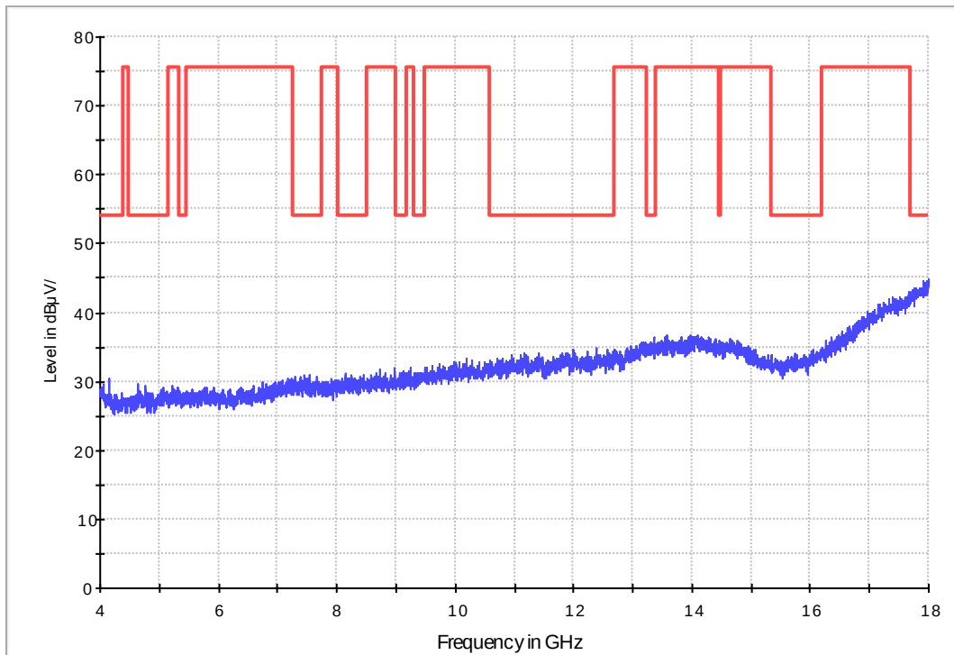
Fig. 71 Radiated Spurious Emission (802.11n-HT20, Ch6, 4 GHz-18 GHz)
