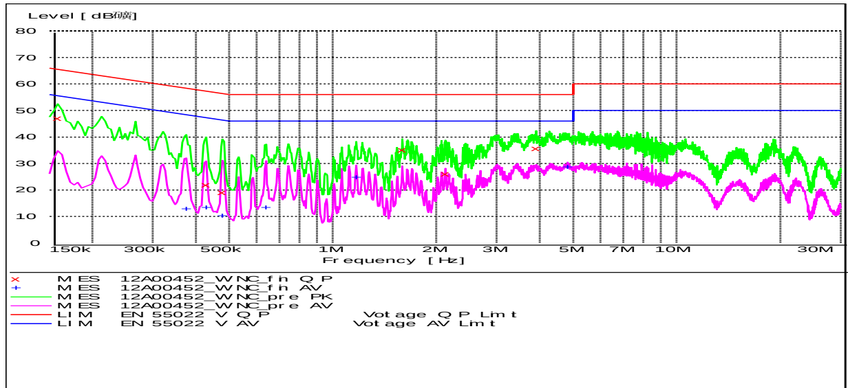
Fig. 86 AC Powerline Conducted Emission
