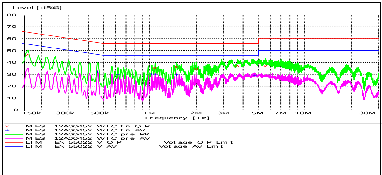
Fig. 87 AC Powerline Conducted Emission
