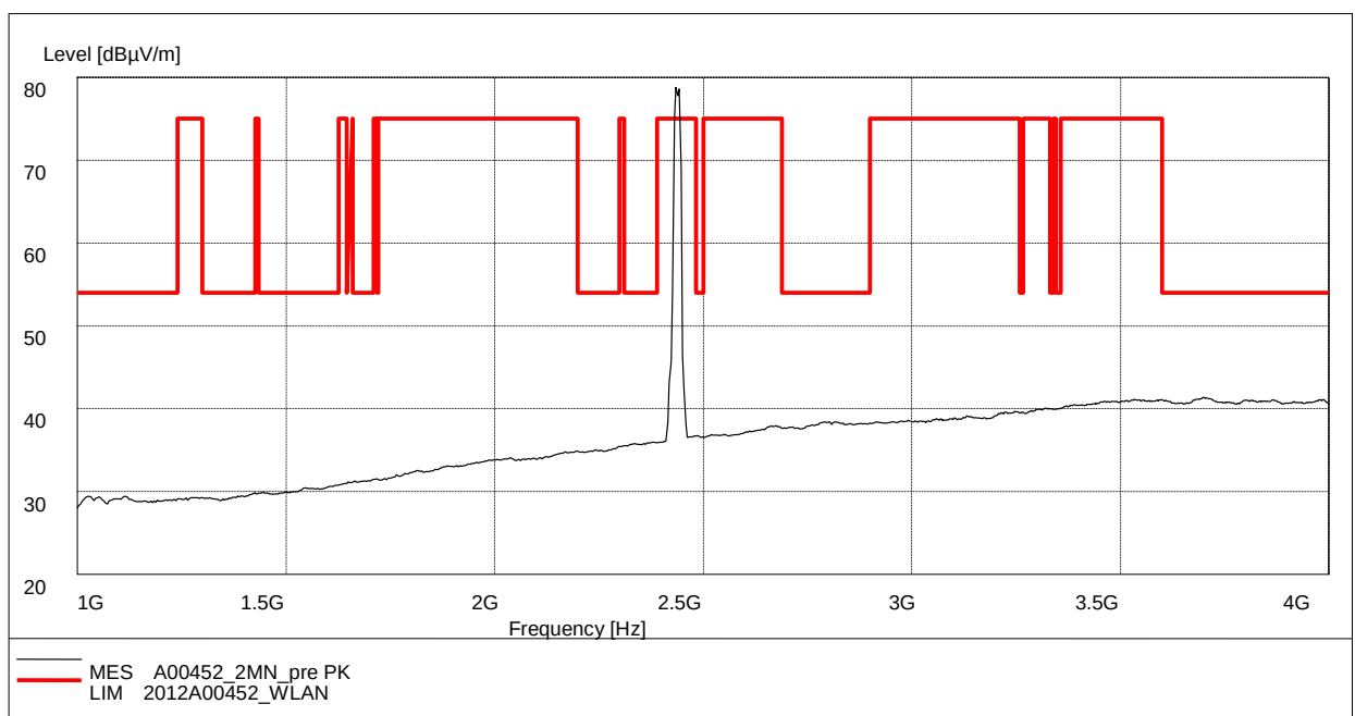
Fig. 70 Radiated Spurious Emission (802.11n-HT20, Ch6, 1 GHz-4 GHz)
