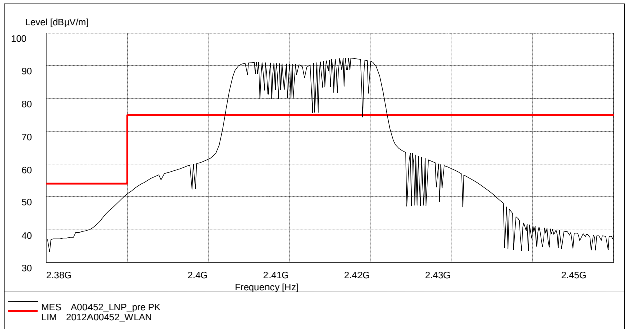
Fig. 65 Radiated Spurious Emission (Power): 802.11n-HT20, ch1, 2.38 GHz - 2.45GHz
