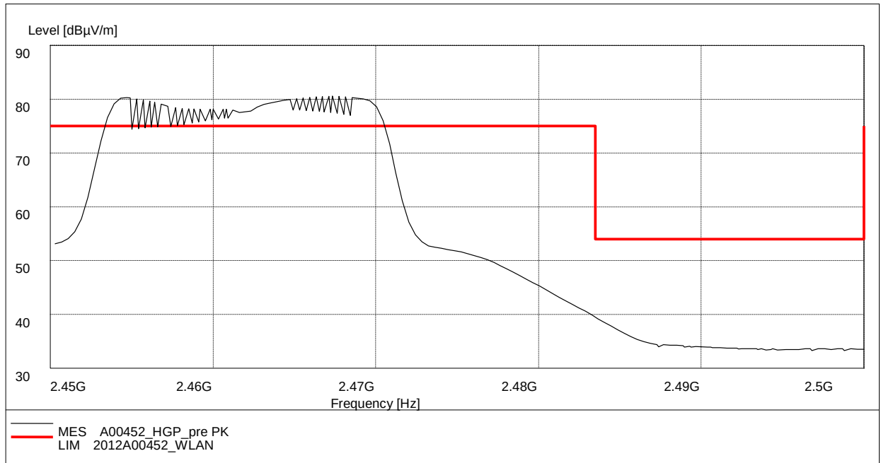
Fig. 61 Radiated Spurious Emission (Power): 802.11g, ch11, 2.45 GHz - 2.5GHz
