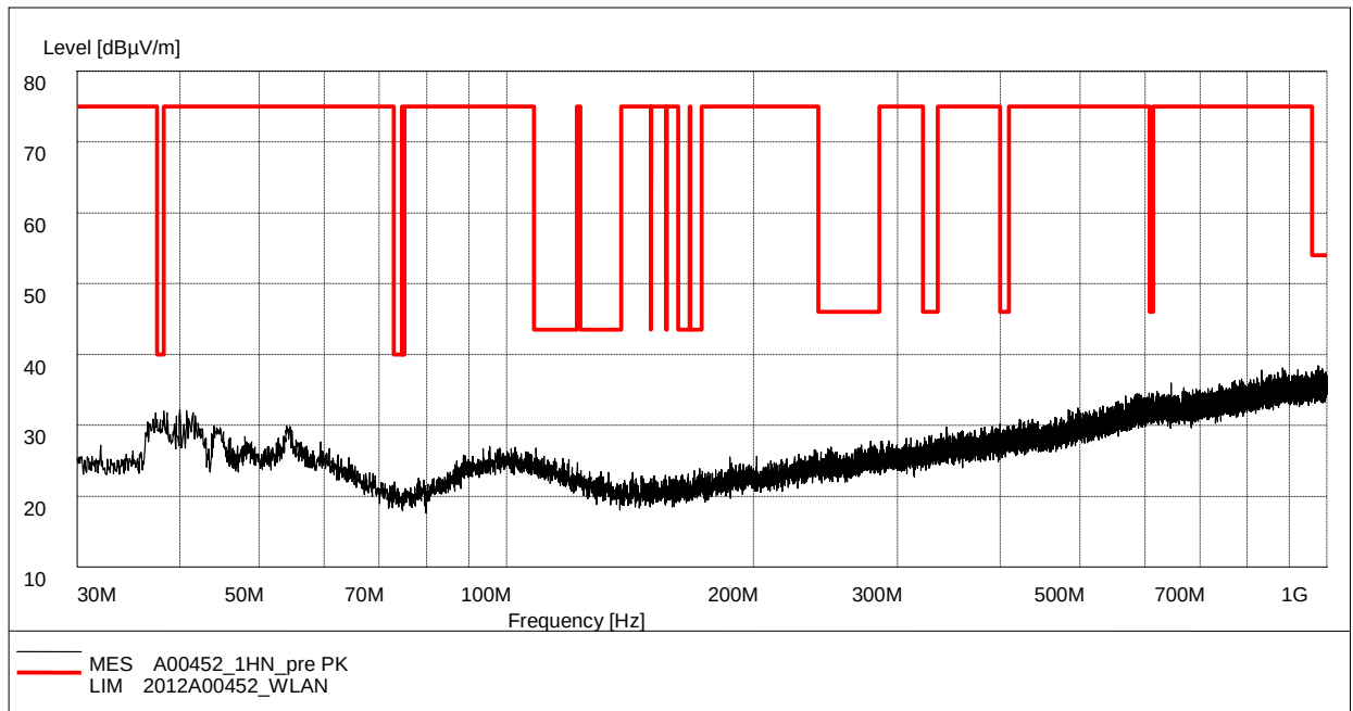
Fig. 73 Radiated Spurious Emission (802.11n-HT20, Ch11, 30 MHz-1 GHz)
