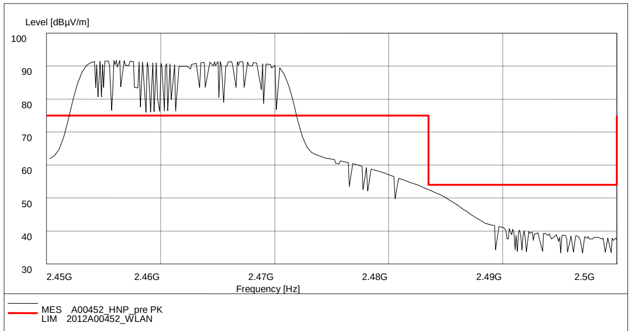
Fig. 72 Radiated Spurious Emission (Power): 802.11n-HT20, ch11, 2.45 GHz - 2.5GHz
