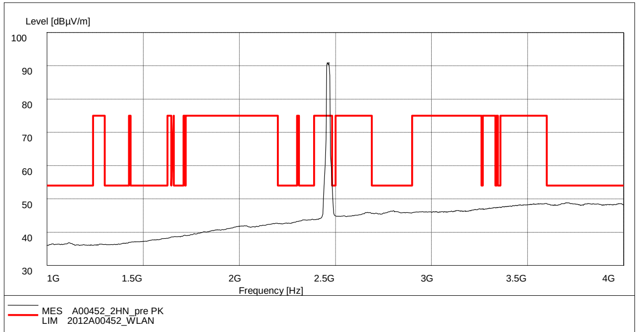
Fig. 74 Radiated Spurious Emission (802.11n-HT20, Ch11, 1 GHz-4 GHz)
