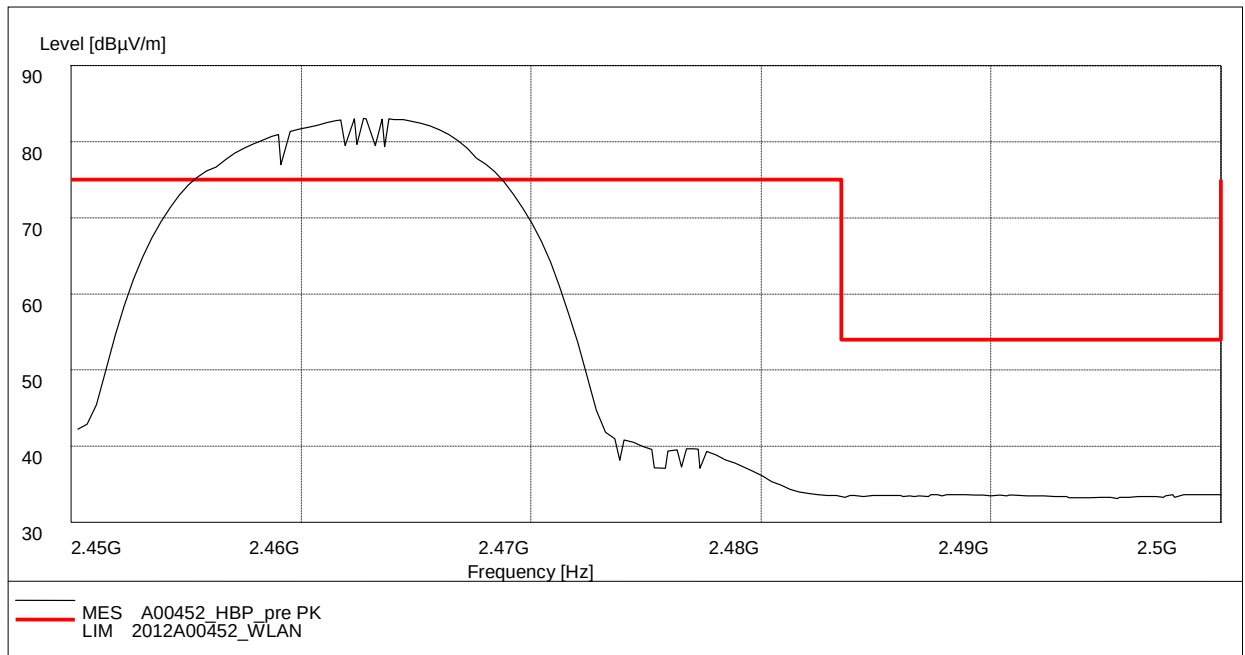
Fig. 50 Radiated Spurious Emission (Power): 802.11b, ch11, 2.45 GHz - 2.5GHz
