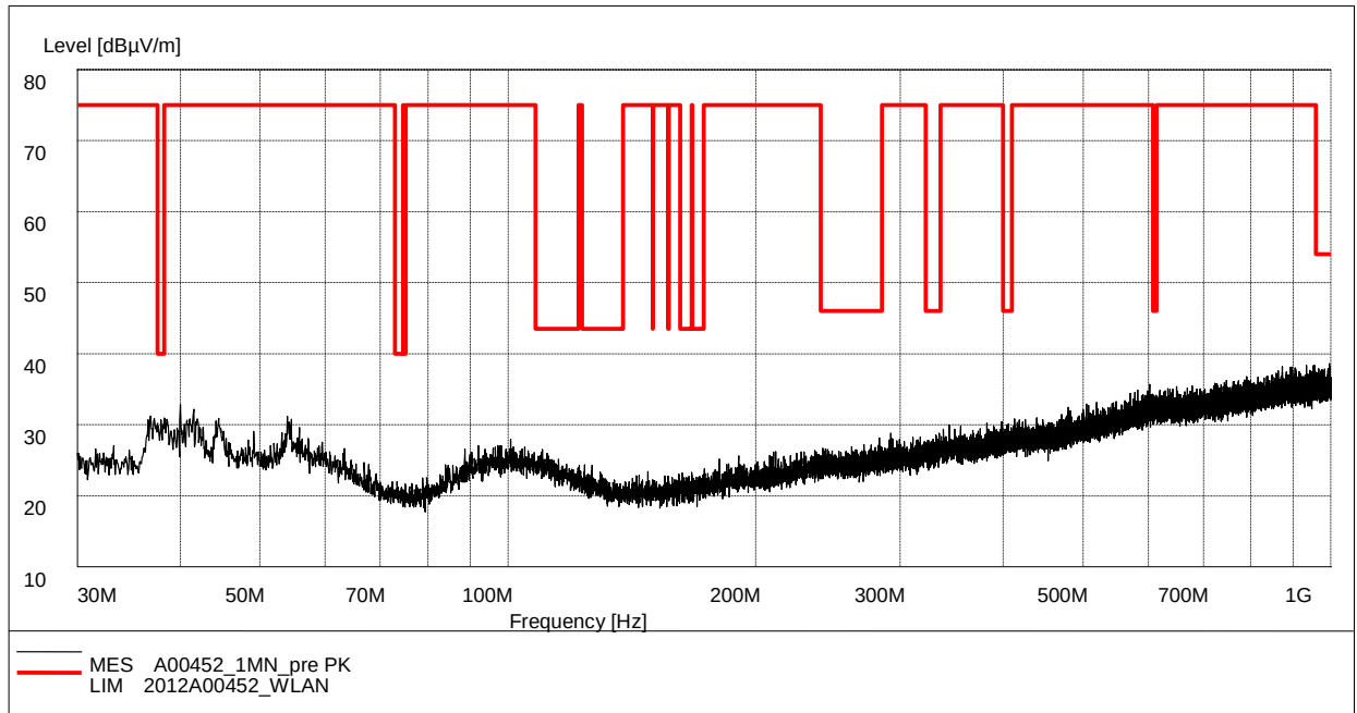
Fig. 69 Radiated Spurious Emission (802.11n-HT20, Ch6, 30 MHz-1 GHz)
