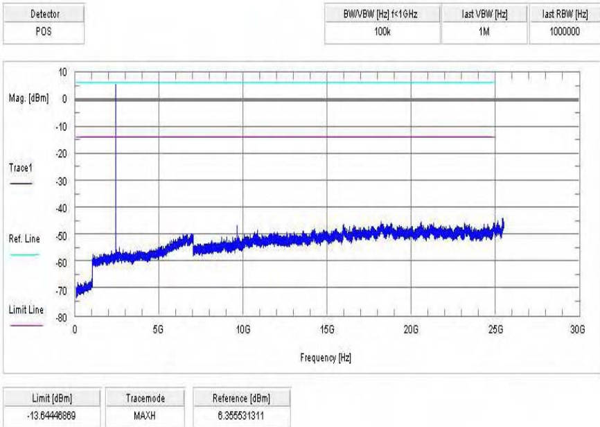
Plot 1: Channel 00 / GFSK
