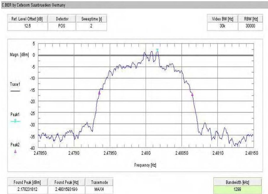
Plot 9: Channel 78 / 8DPSK
