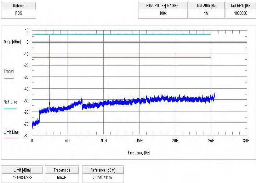
Plot 8: Channel 00 / 8DPSK
