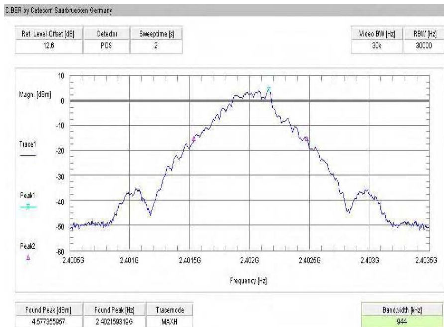
Plot 1: Channel 00 / GFSK
