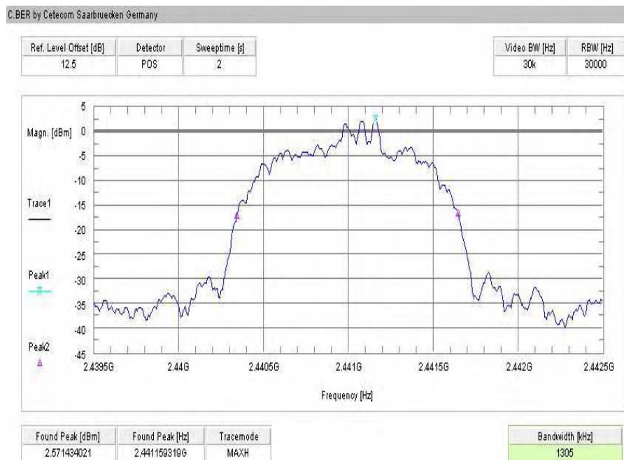
Plot 8: Channel 39 / 8DPSK
