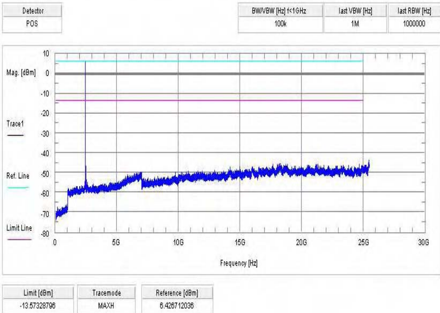
Plot 2: Channel 39 / GFSK
