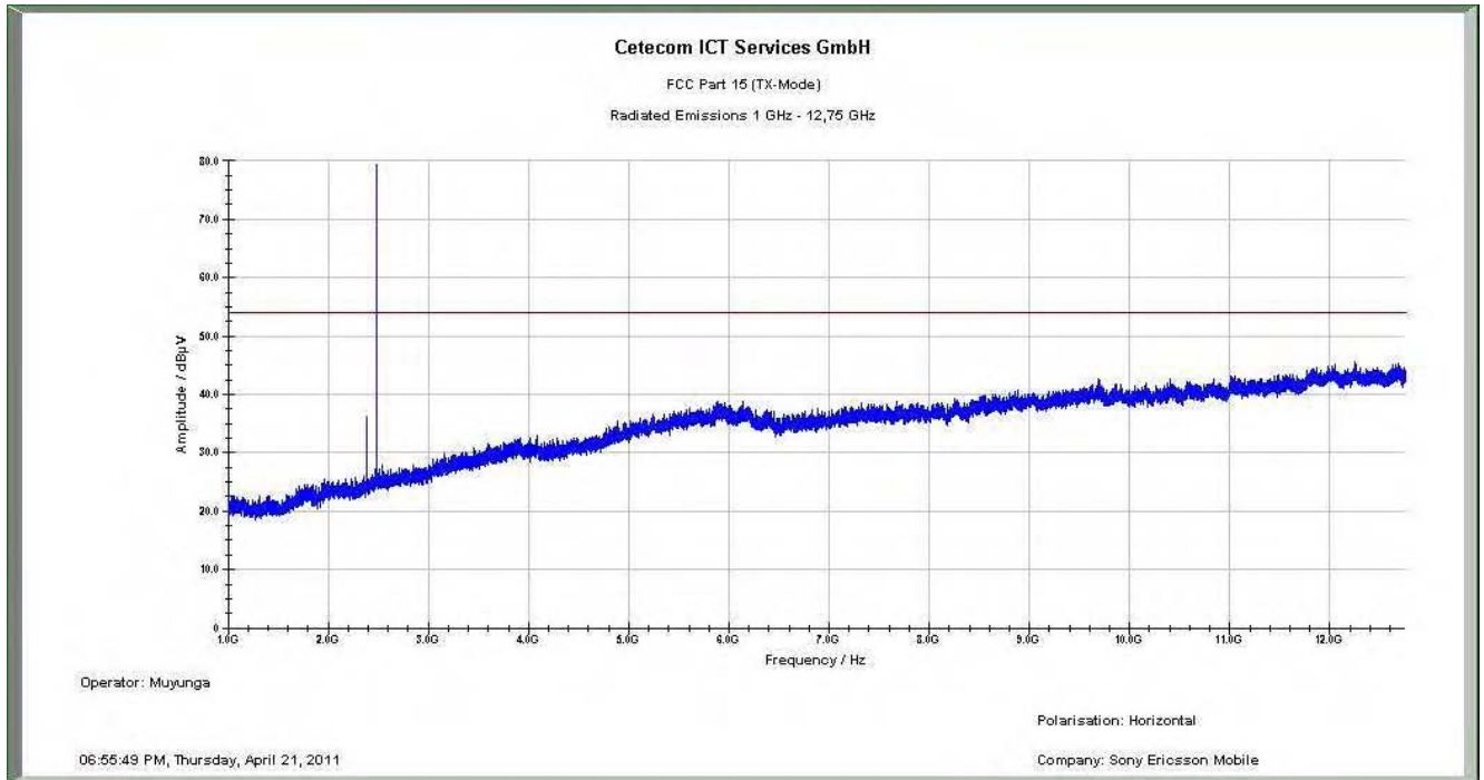
Plot 7: 1 GHz to 12.75 GHz / channel 78 (horizontal/vertical)
