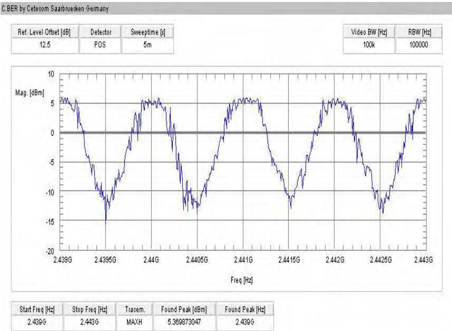
Plot 1: Carrier Frequency Separation (GFSK)
