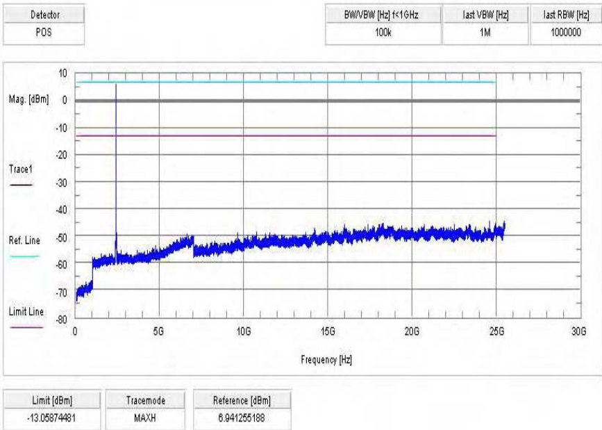
Plot 7: Channel 00 / 8DPSK
