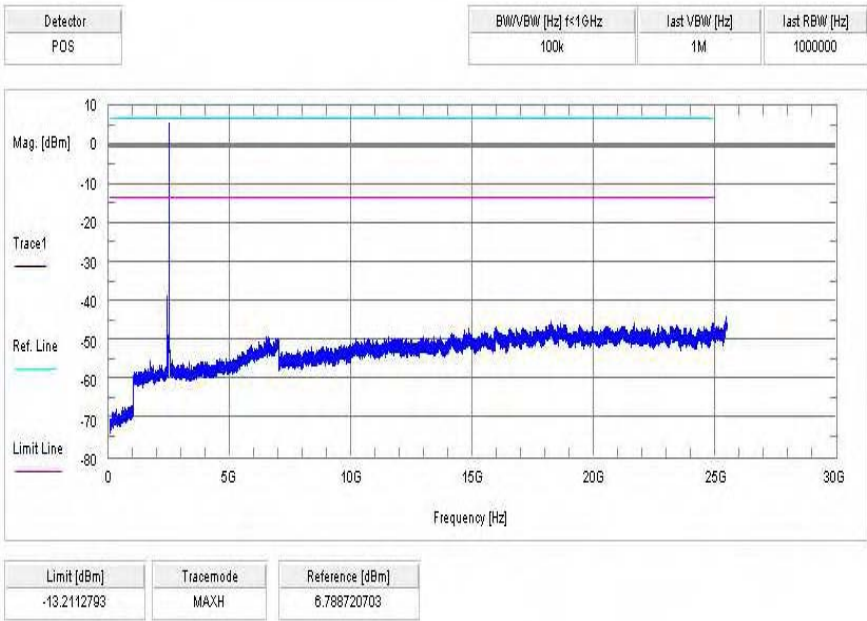
Plot 9: Channel 00 / 8DPSK
