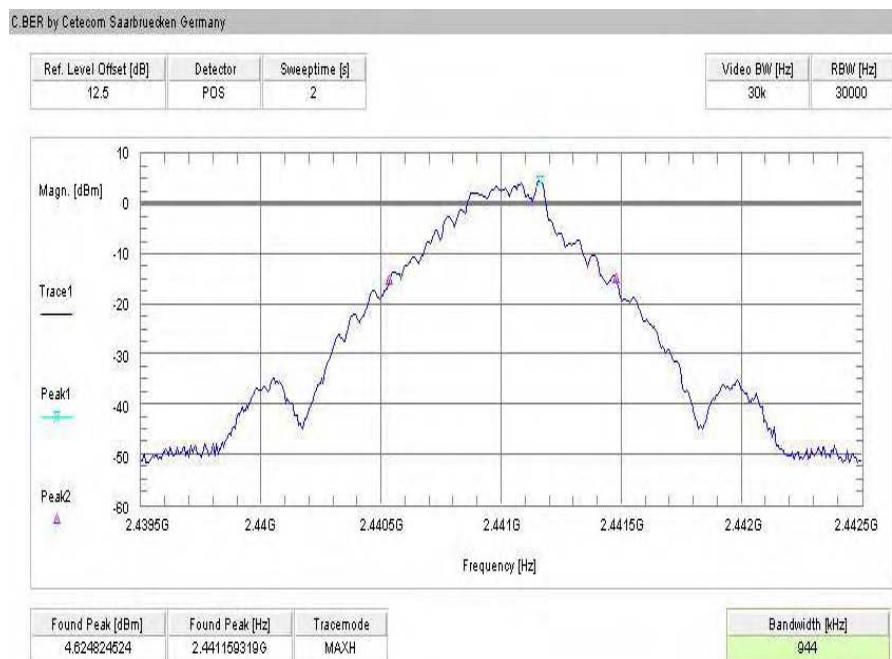
Plot 2: Channel 39 / GFSK
