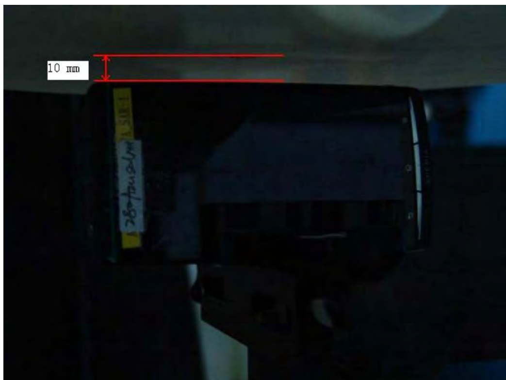
Picture G9: Body-worn Position (EUT's right side towards phantom, the distance from handset to the bottom of the Phantom is 10 mm)
