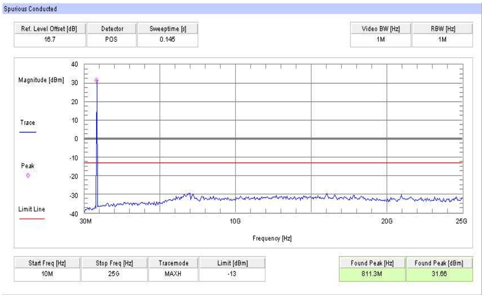
Plot 2: Channel 189 (10 MHz - 25 GHz)
