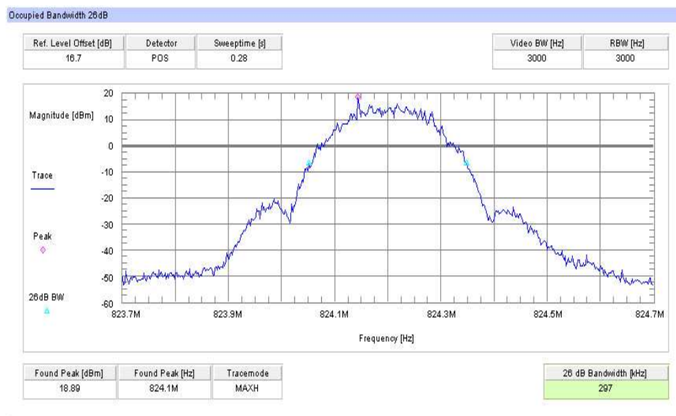
Plot 8: Channel 128 (-26 dBc BW) - EDGE
