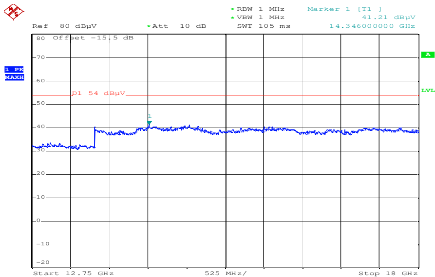
Plot 4: 12.75 GHz to 18 GHz / channel 00 (horizontal & vertical)
