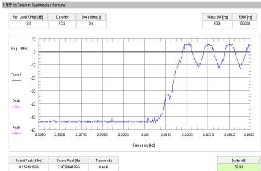
Plot 1: Lower band edge – hopping on / GFSK (conducted)
