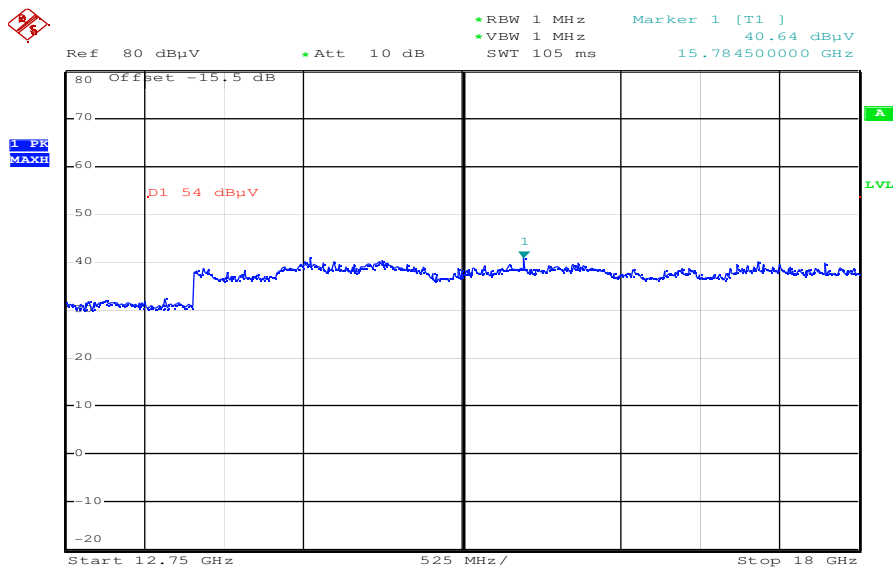
Plot 4: 12.75 GHz to 18 GHz / idle-mode (horizontal & vertical)
