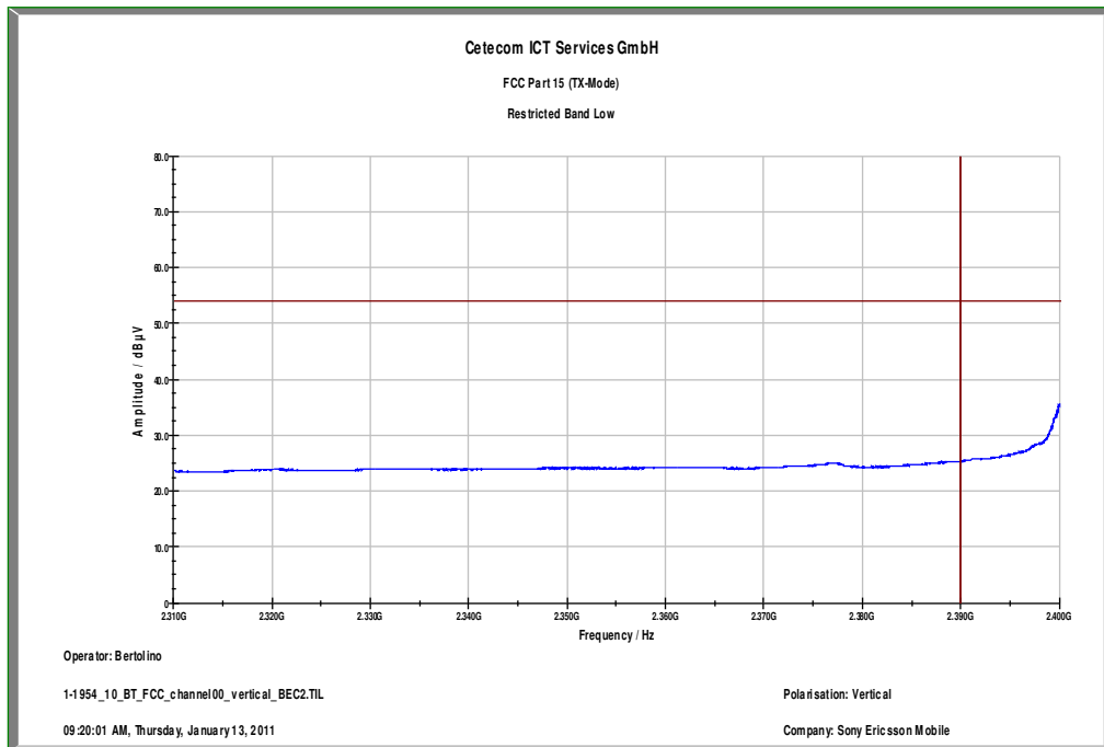
Plot 5: Lower Restricted Band / Pi/4 DQPSK (radiated), vertical polarization
