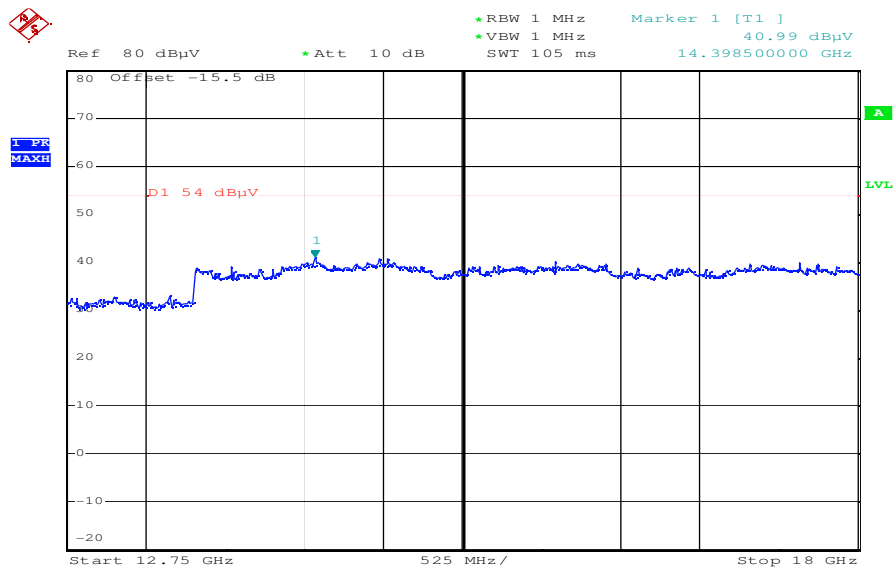
Plot 14: 12.75 GHz to 18 GHz / channel 78 (horizontal & vertical)
