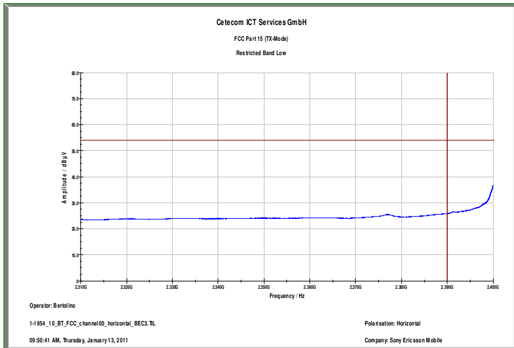
Plot 11: Lower Restricted Band / 8DPSK (radiated), horizontal polarization
