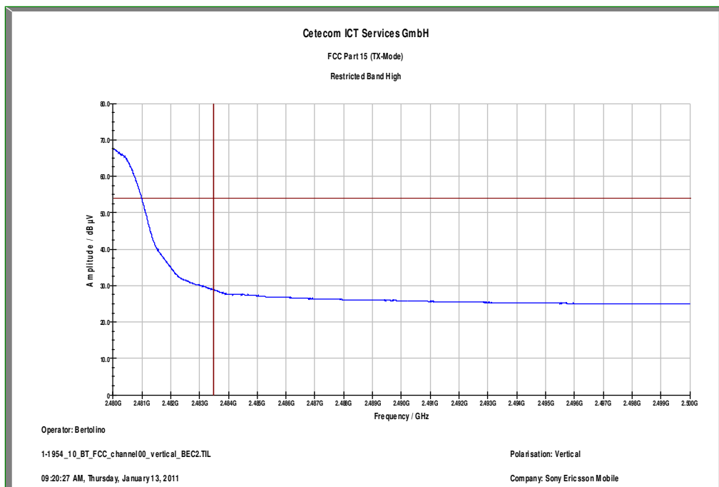
Plot 6: Upper Restricted Band / Pi/4 DQPSK (radiated), vertical polarization
