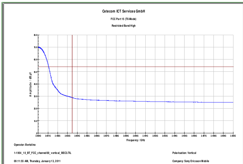
Plot 10: Upper Restricted Band / 8DPSK (radiated), vertical polarization
