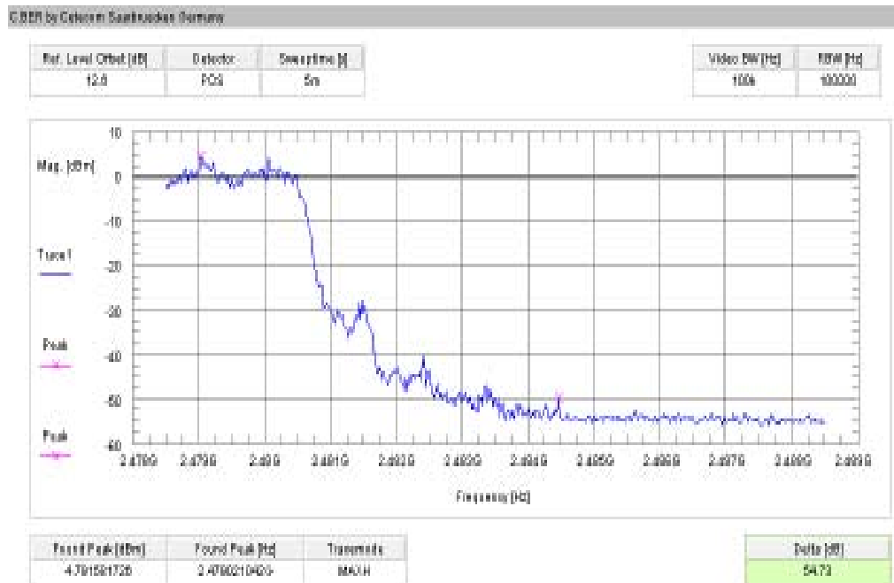
Plot 10: Upper band edge – hopping on / 8DPSK (conducted)
