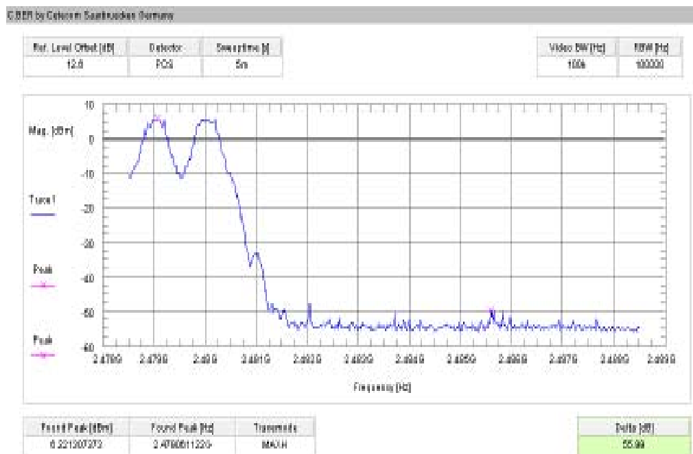
Plot 2: Upper band edge – hopping on / GFSK (conducted)
