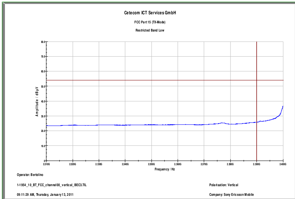
Plot 9: Lower Restricted Band / 8DPSK (radiated), vertical polarization
