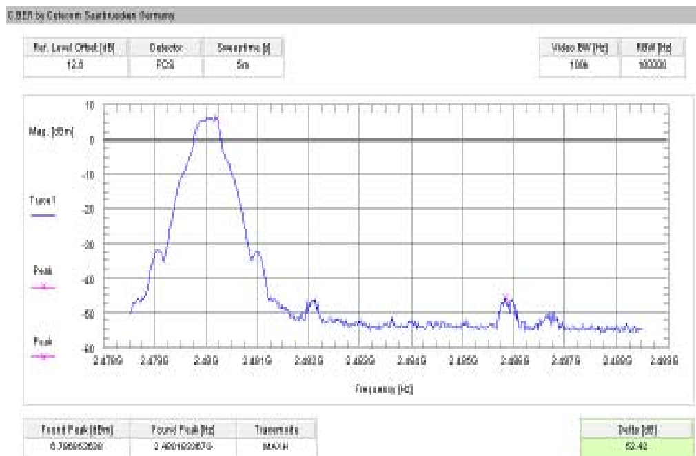
Plot 4: Upper band edge – hopping off / GFSK (conducted)
