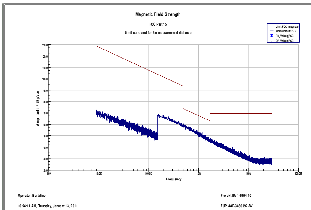
Plot 4: 9 kHz to 30 MHz / RX
