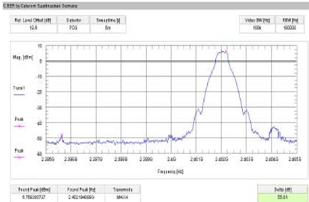
Plot 3: Lower band edge – hopping off / GFSK (conducted)
