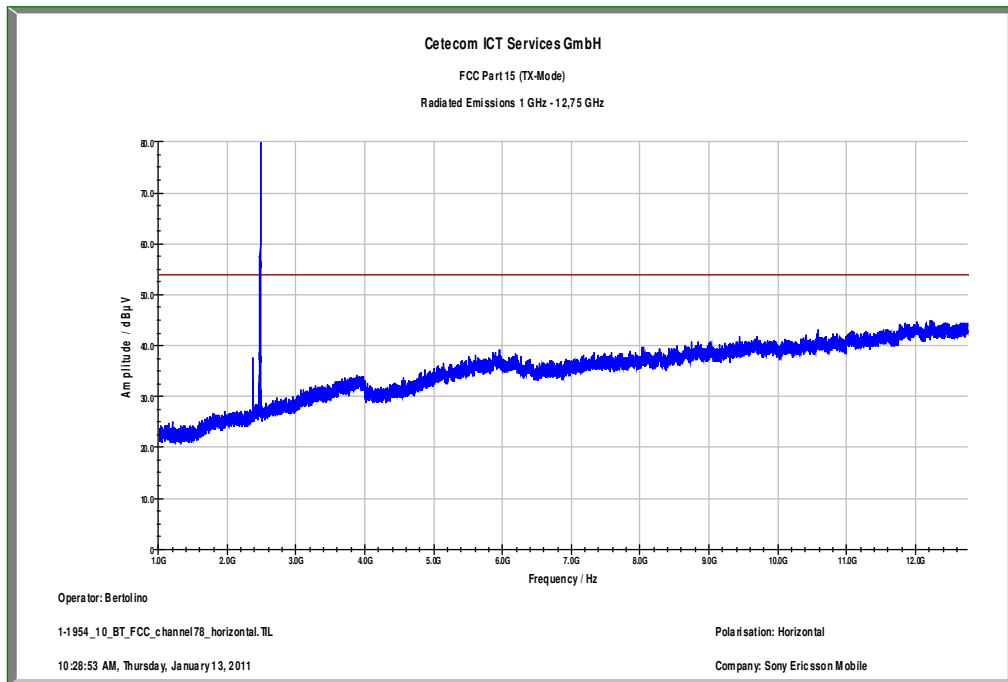
Plot 13: 1 GHz to 12.75 GHz / channel 78 (horizontal)
