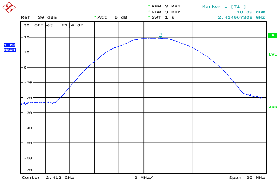
Plot 1: TX mode, lowest channel, 5.5 MBit/s
