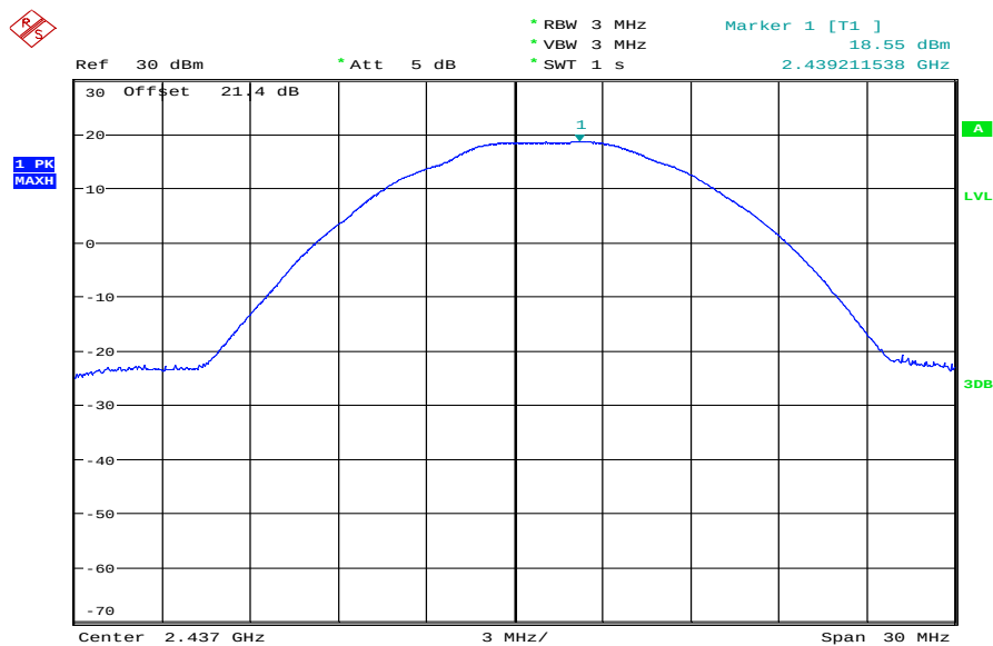
Plot 2: TX mode, middle channel, 5.5 MBit/s
