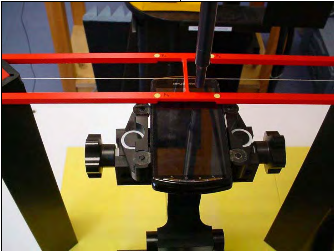
Photo 7: Test position
