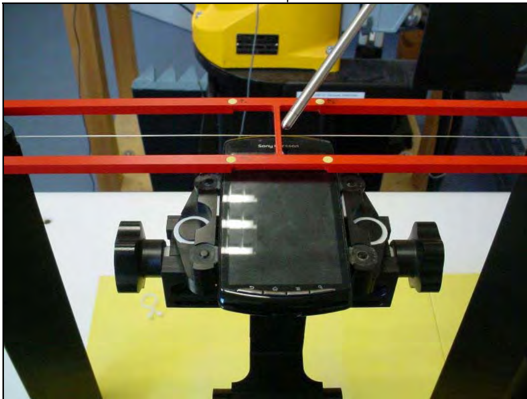
Photo 6: Test position
