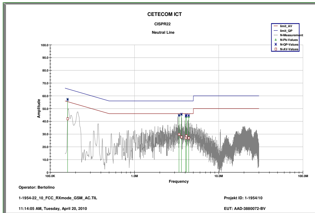
Plot 2: RX mode, neutral line
