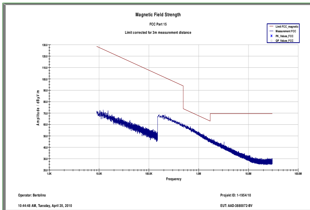
Plot 1: RX mode, 10 kHz – 30 MHz (valid for all channels)
