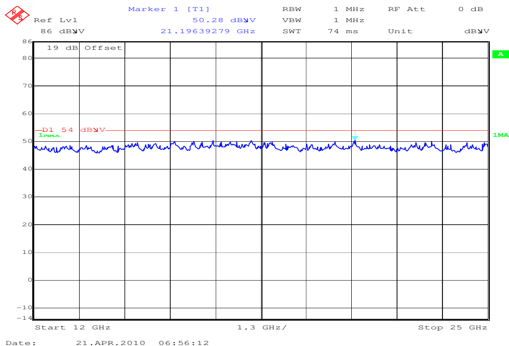
Plot 5: RX mode, 12 GHz – 25 GHz (valid for all channels)
