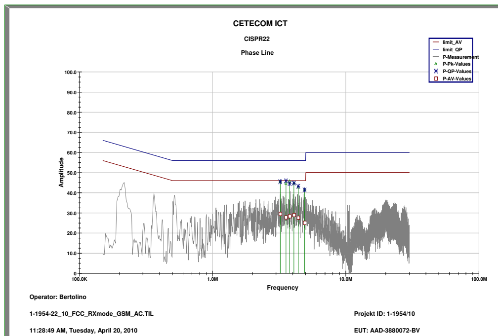
Plot 1: RX mode, phase line
