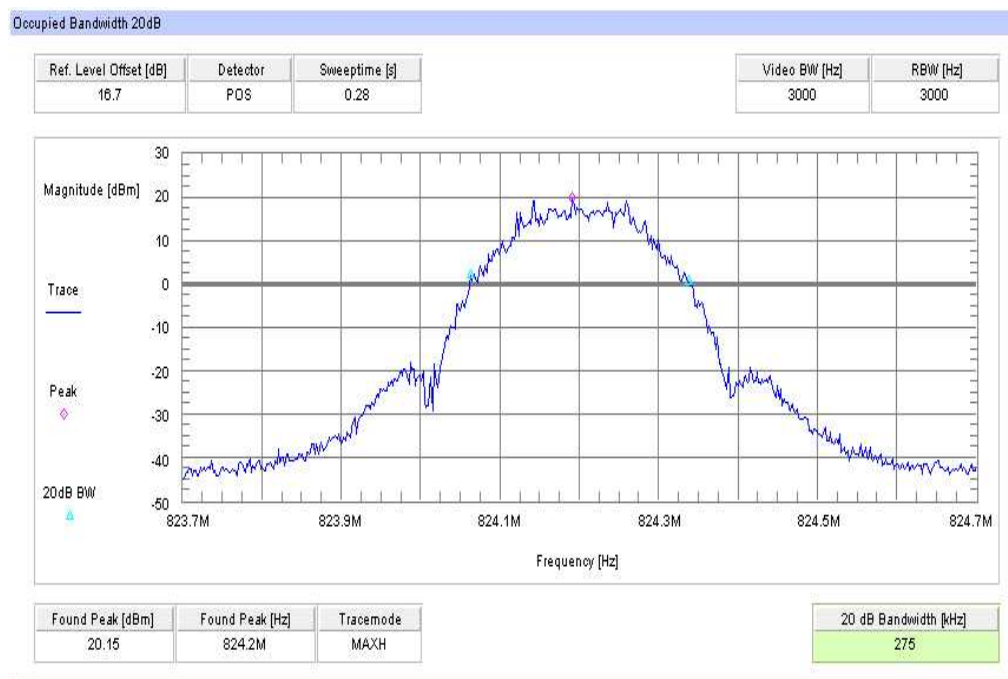
Plot 7: TX mode, channel 128, EGPRS / EDGE, 99% (-20 dB) Occupied Bandwidth
