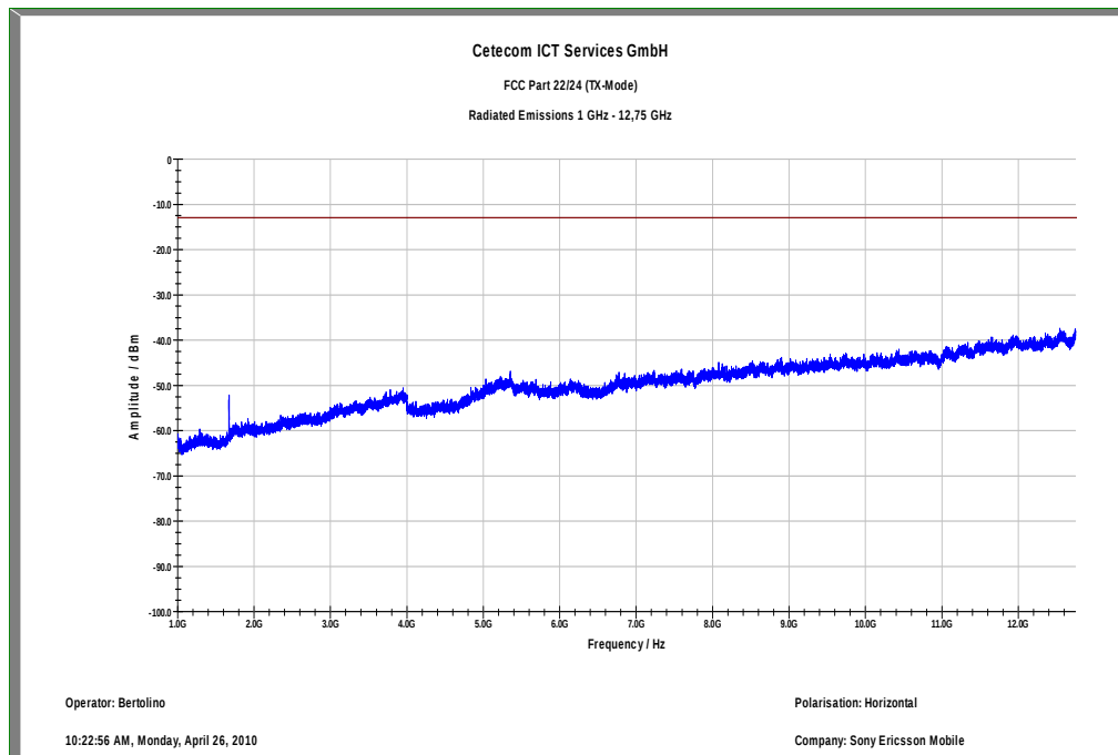
Plot 10: TX mode, channel 4180, UMTS / WCDMA, 1 GHz – 12.75 GHz, horizontal polarization
