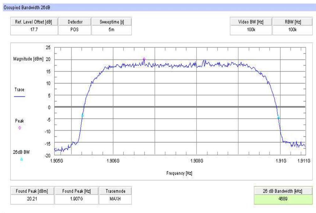
Plot 6: TX mode, channel 9538, UMTS / WCDMA, -26 dBc Bandwidth
