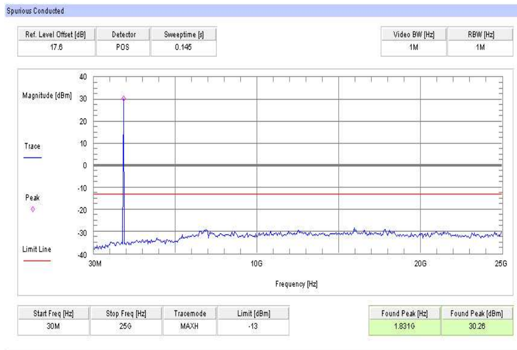
Plot 1: TX mode, channel 512, GSM, 30 MHz – 25 GHz
