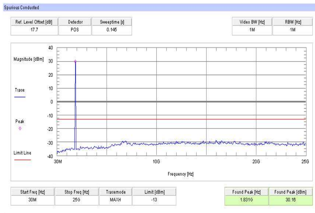
Plot 2: TX mode, channel 661, GSM, 30 MHz – 25 GHz
