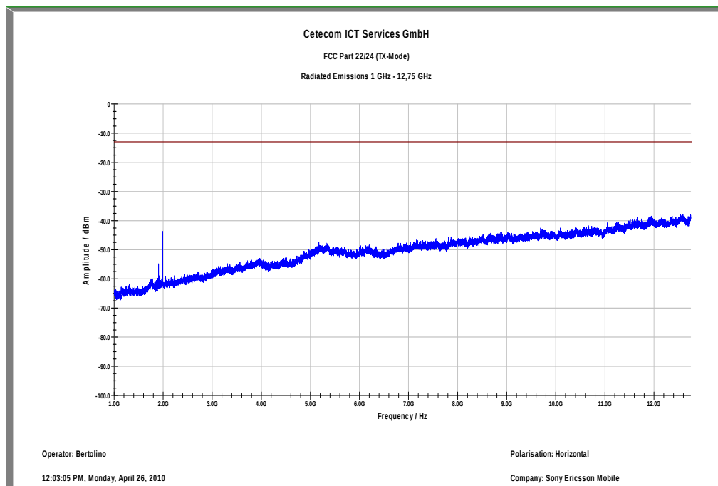
Plot 15: TX mode, channel 9538, UMTS / WCDMA, 1 GHz – 12.75 GHz, horizontal polarization
