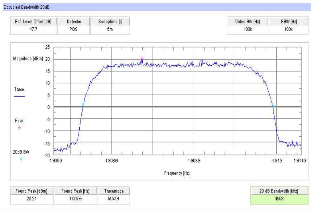
Plot 5: TX mode, channel 9538, UMTS / WCDMA, 99% (-20 dB) Occupied Bandwidth
