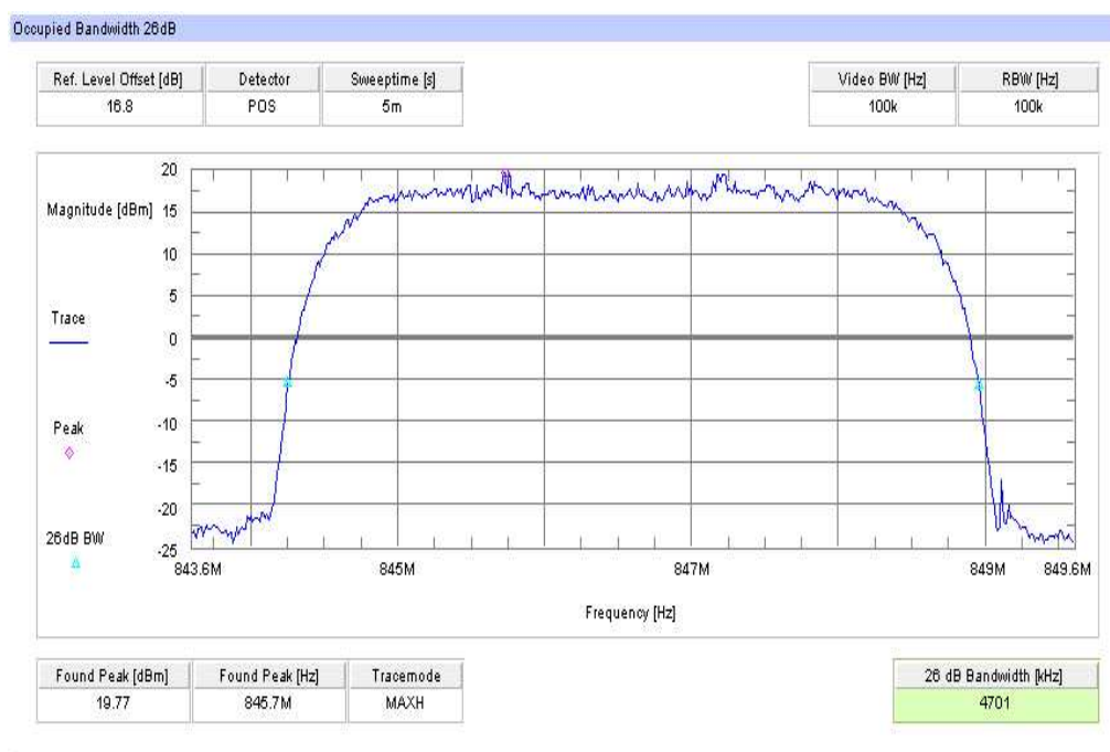
Plot 6: TX mode, channel 4233, UMTS / WCDMA, -26 dBc Bandwidth
