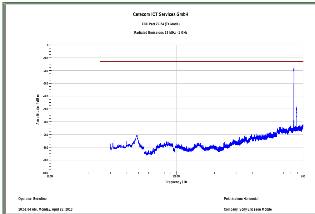
Plot 14: TX mode, channel 4233, UMTS / WCDMA, 30 MHz – 1 GHz, horizontal polarization
