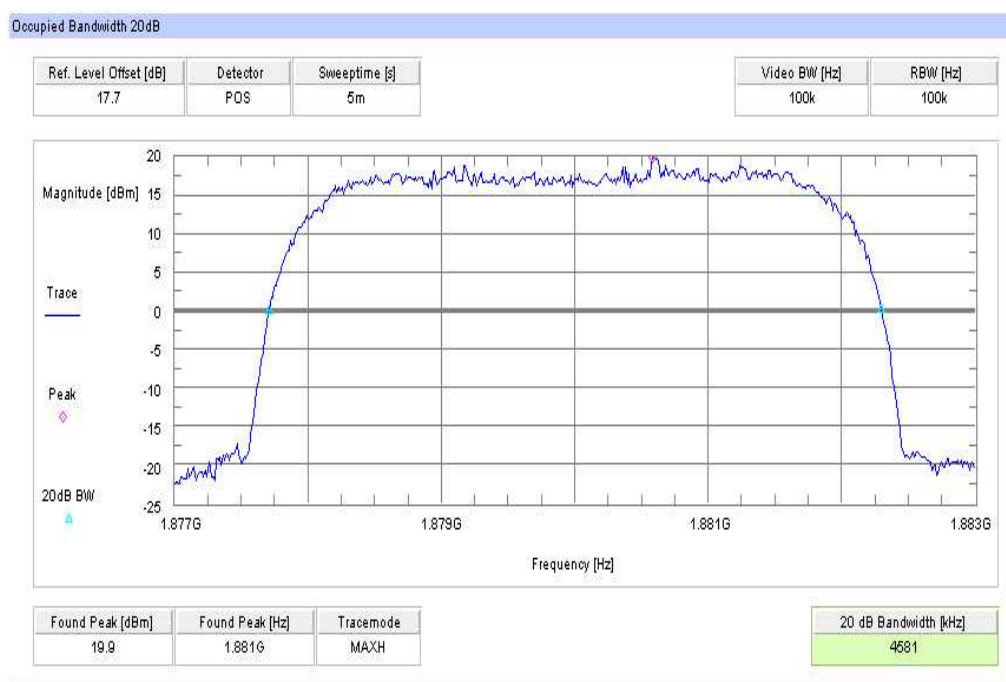
Plot 3: TX mode, channel 9400, UMTS / WCDMA, 99% (-20 dB) Occupied Bandwidth
