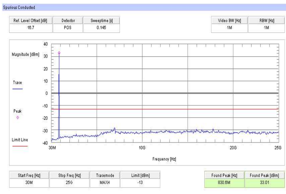
Plot 2: TX mode, channel 189, GSM, 30 MHz – 25 GHz
