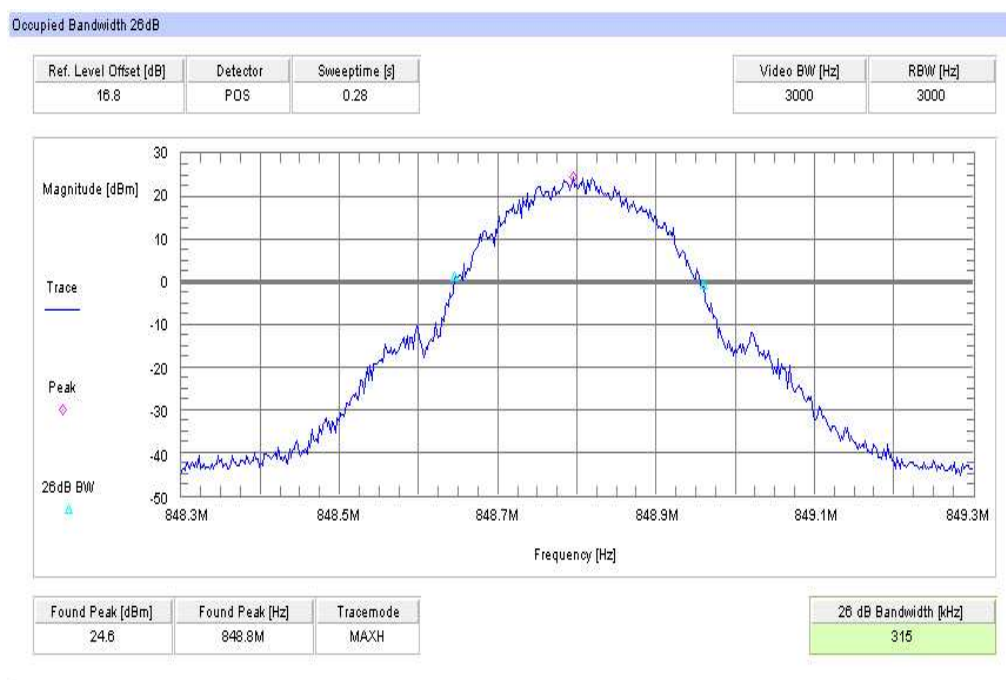
Plot 6: TX mode, channel 251, GSM, -26 dBc Bandwidth
