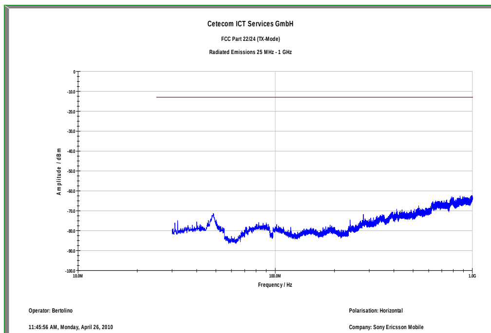
Plot 9: TX mode, channel 9400, UMTS / WCDMA, 30 MHz – 1 GHz, horizontal polarization
