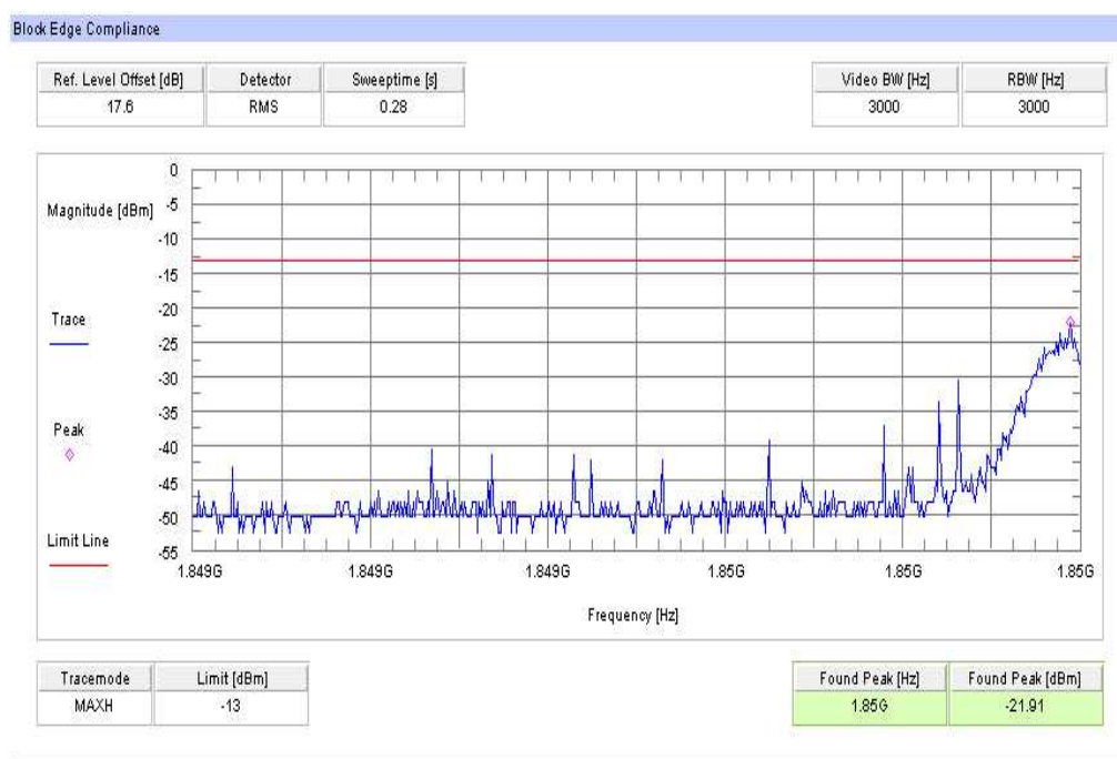
Plot 3: TX mode, channel 512, EGPRS / EDGE, block 1
