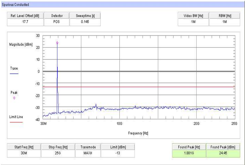
Plot 3: TX mode, channel 9538, UMTS / WCDMA, 30 MHz – 25 GHz
