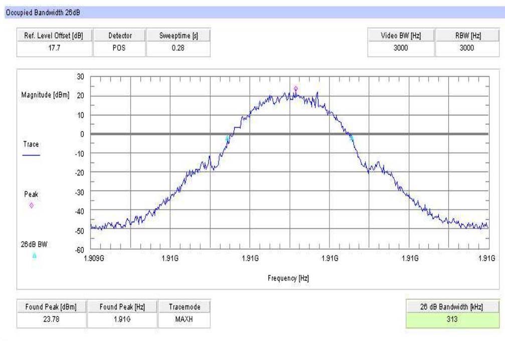
Plot 6: TX mode, channel 810, GSM, -26 dBc Bandwidth
