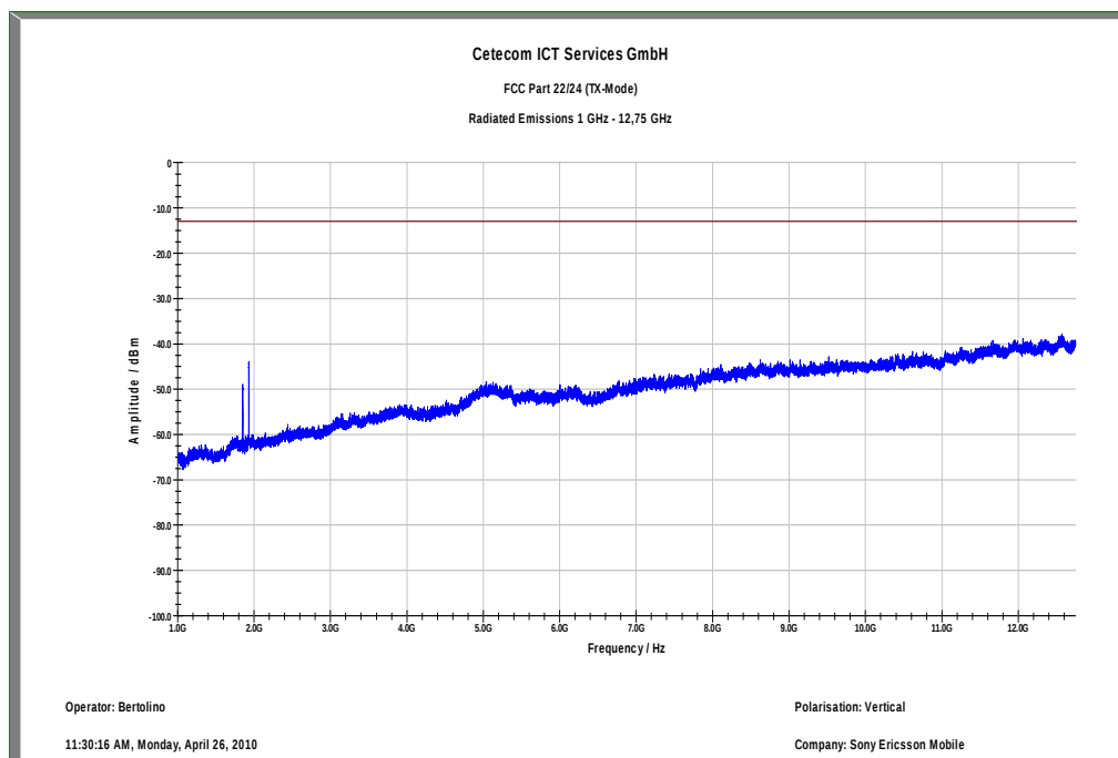
Plot 2: TX mode, channel 9262, UMTS / WCDMA, 1 GHz – 12.75 GHz, vertical polarization
