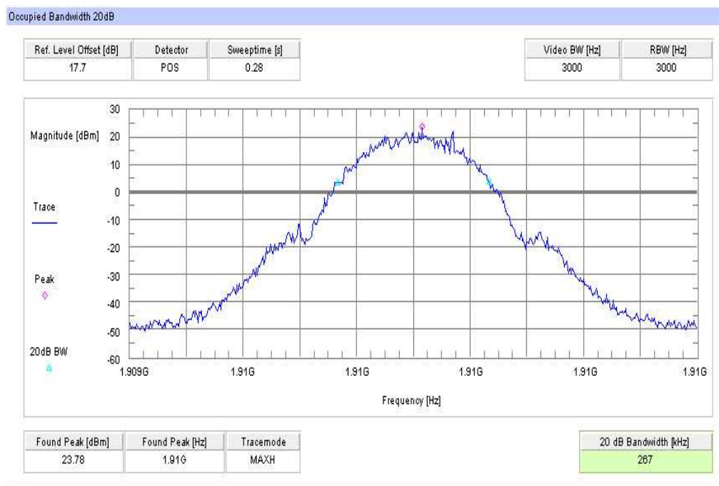
Plot 5: TX mode, channel 810, GSM, 99% (-20 dB) Occupied Bandwidth
