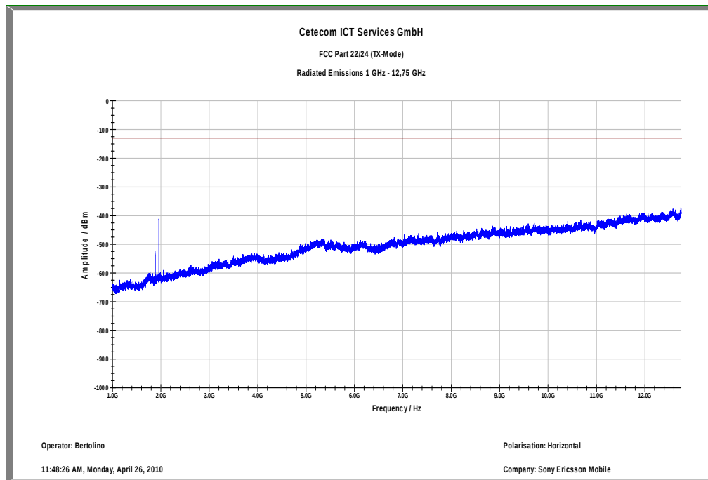
Plot 10: TX mode, channel 9400, UMTS / WCDMA, 1 GHz – 12.75 GHz, horizontal polarization
