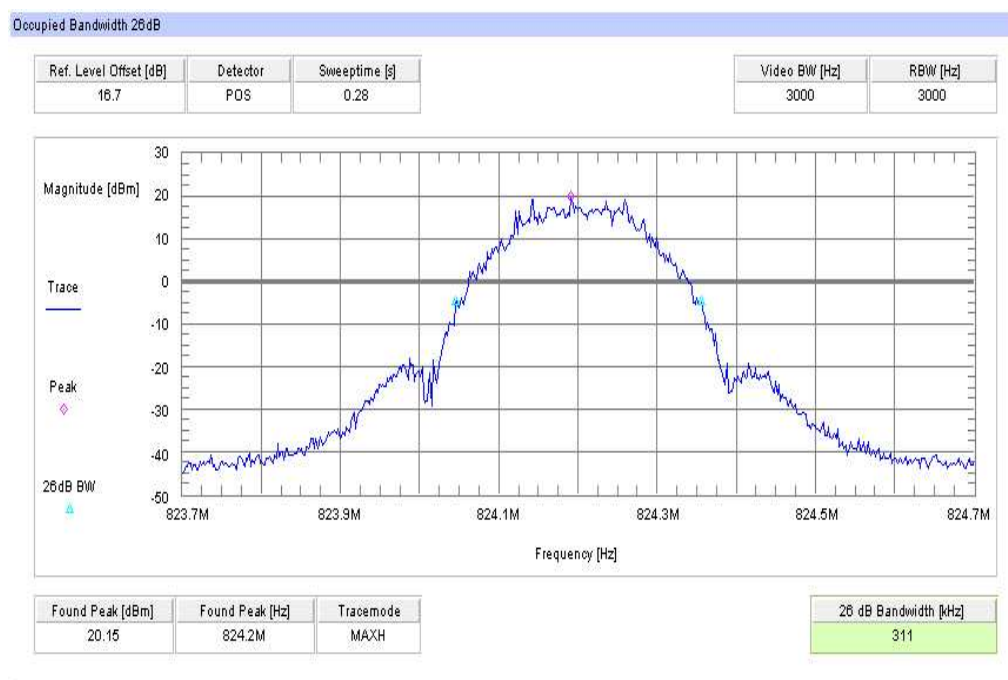
Plot 8: TX mode, channel 128, EGPRS / EDGE, -26 dBc Bandwidth
