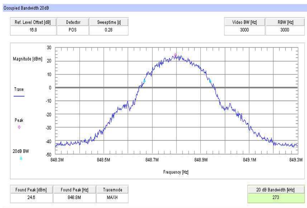
Plot 5: TX mode, channel 251, GSM, 99% (-20 dB) Occupied Bandwidth
