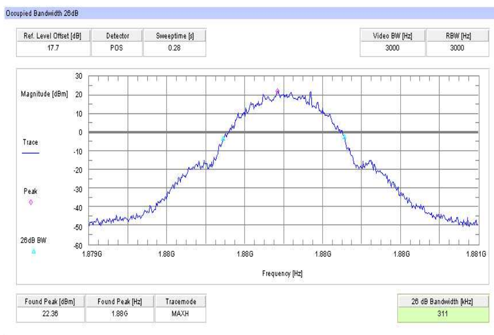
Plot 4: TX mode, channel 661, GSM, -26 dBc Bandwidth
