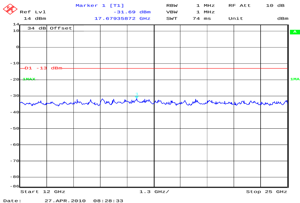
Plot 11: TX mode, channel 189, GSM, 12 GHz - 25 GHz (valid for all channels)
