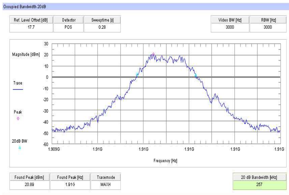
Plot 11: TX mode, channel 810, EGPRS / EDGE, 99% (-20 dB) Occupied Bandwidth
