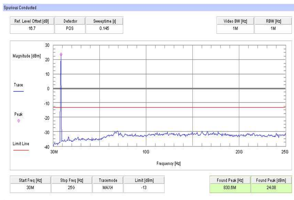
Plot 2: TX mode, channel 4180, UMTS / WCDMA, 30 MHz – 25 GHz
