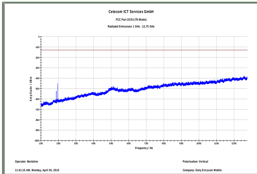
Plot 8: TX mode, channel 9400, UMTS / WCDMA, 1 GHz – 12.75 GHz, vertical polarization
