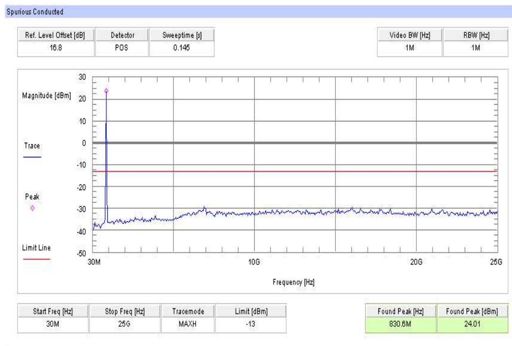
Plot 3: TX mode, channel 4233, UMTS / WCDMA, 30 MHz – 25 GHz
