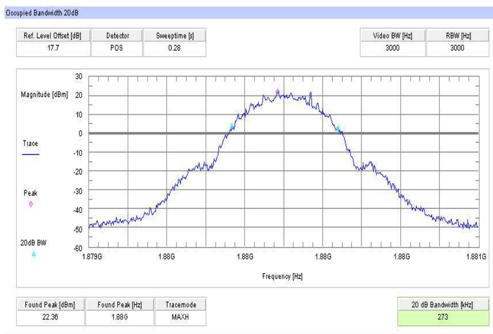
Plot 3: TX mode, channel 661, GSM, 99% (-20 dB) Occupied Bandwidth
