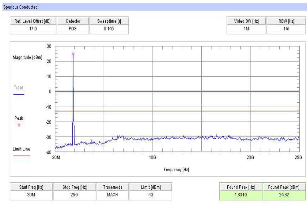
Plot 1: TX mode, channel 9262, UMTS / WCDMA, 30 MHz – 25 GHz
