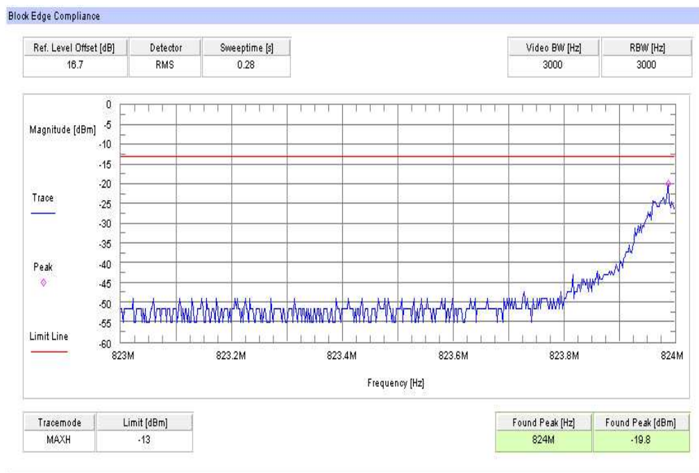
Plot 3: TX mode, channel 128, EGPRS / EDGE, block 1
