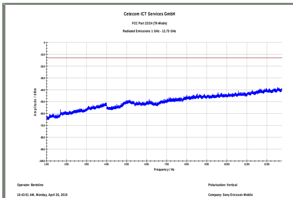
Plot 13: TX mode, channel 4233, UMTS / WCDMA, 1 GHz – 12.75 GHz, vertical polarization
