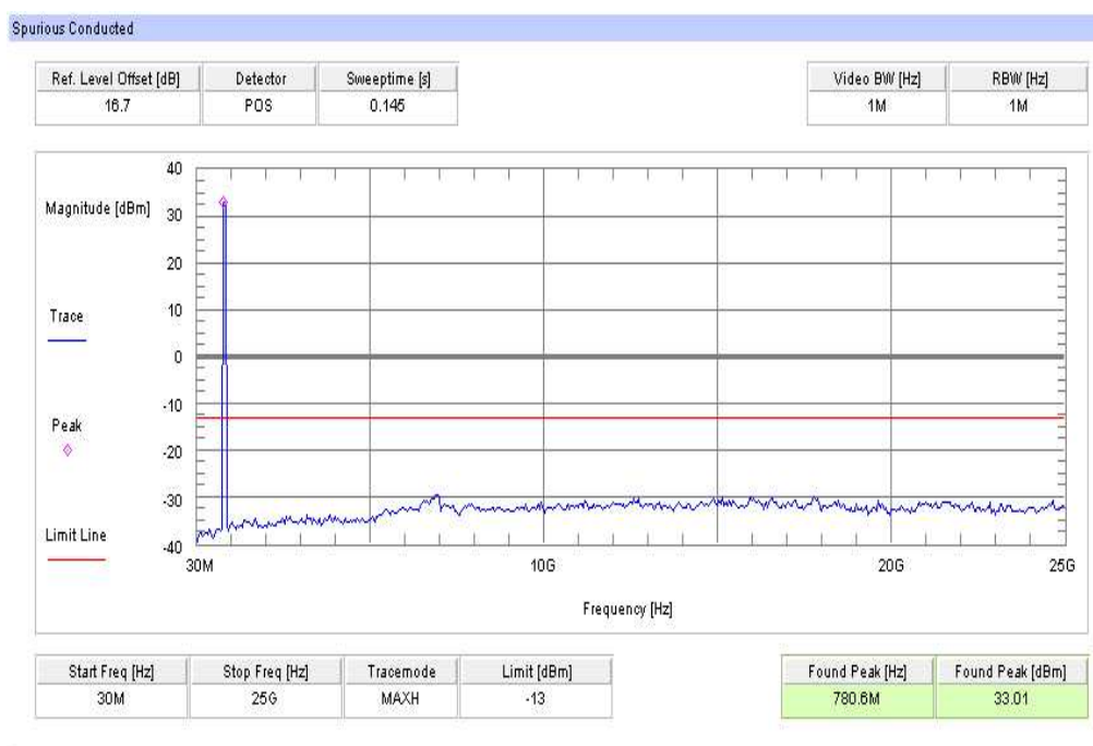
Plot 1: TX mode, channel 128, GSM, 30 MHz – 25 GHz
