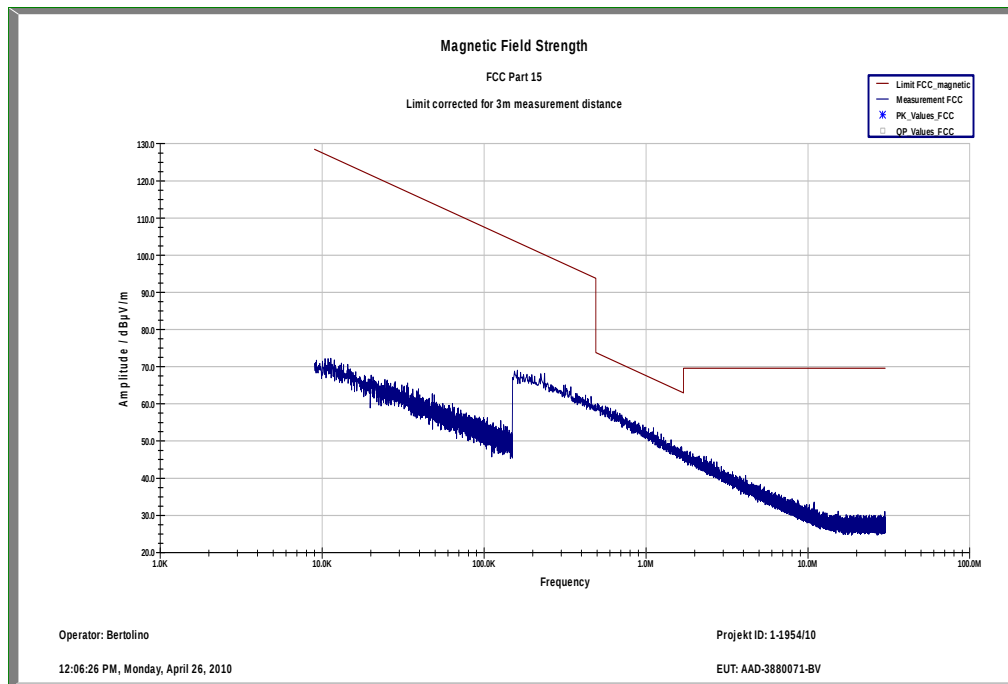
Plot 5: TX mode, channel 9400, UMTS / WCDMA, 10 kHz - 30 MHz (valid for all channels)
