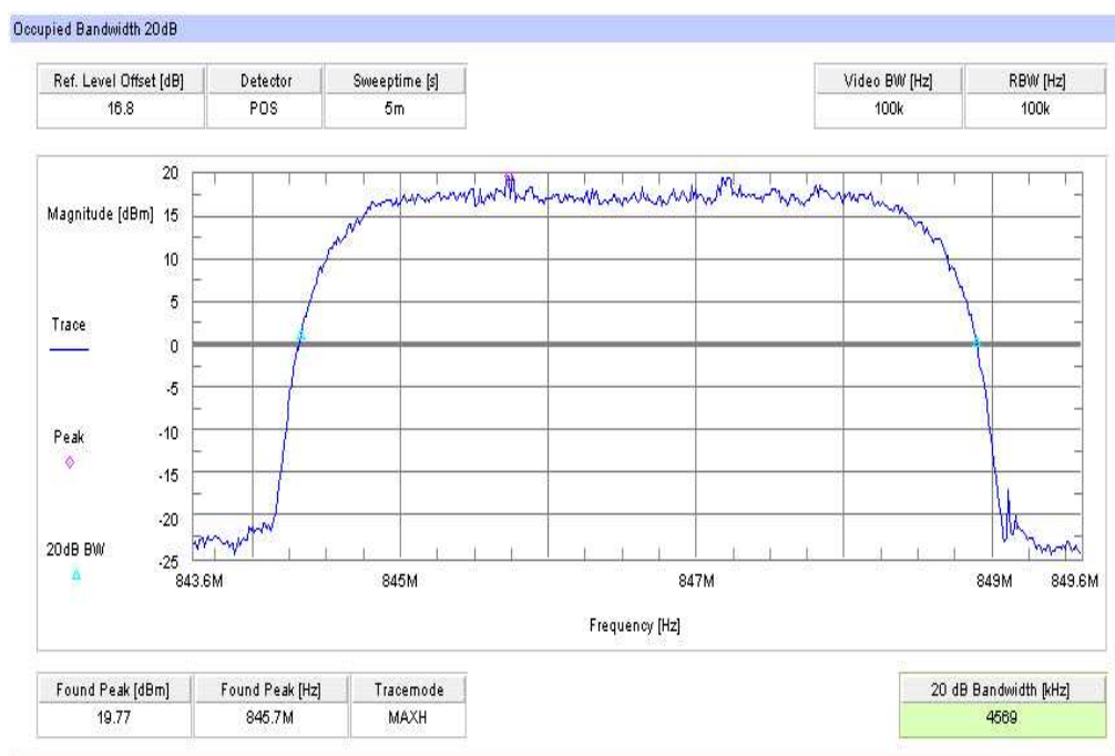
Plot 5: TX mode, channel 4233, UMTS / WCDMA, 99% (-20 dB) Occupied Bandwidth
