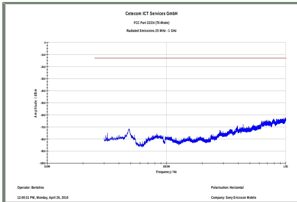
Plot 14: TX mode, channel 9538, UMTS / WCDMA, 30 MHz – 1 GHz, horizontal polarization
