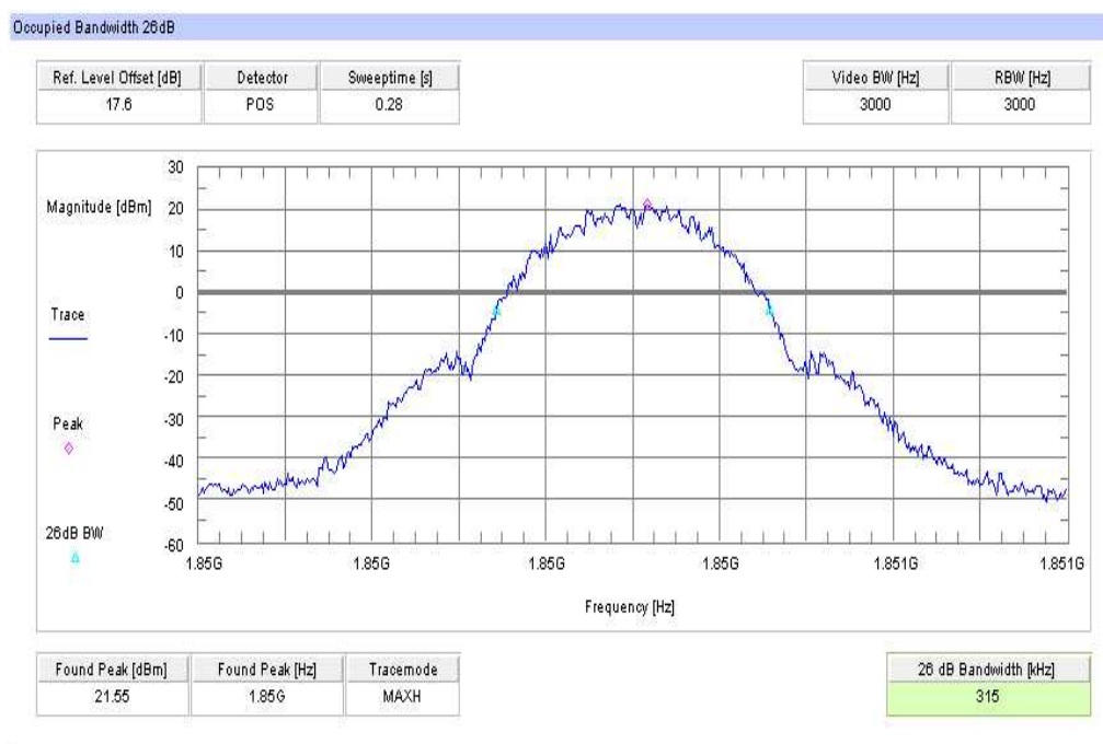
Plot 2: TX mode, channel 512, GSM, -26 dBc Bandwidth
