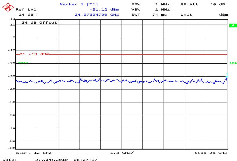
Plot 11: TX mode, channel 661, GSM, 12 GHz - 25 GHz (valid for all channels)
