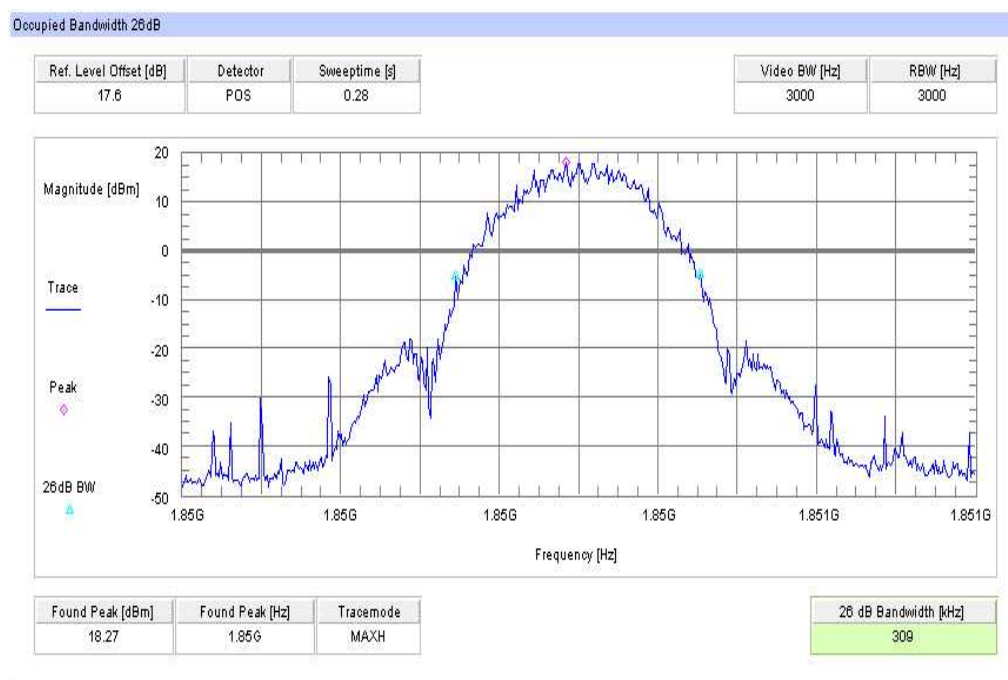
Plot 8: TX mode, channel 512, EGPRS / EDGE, -26 dBc Bandwidth
