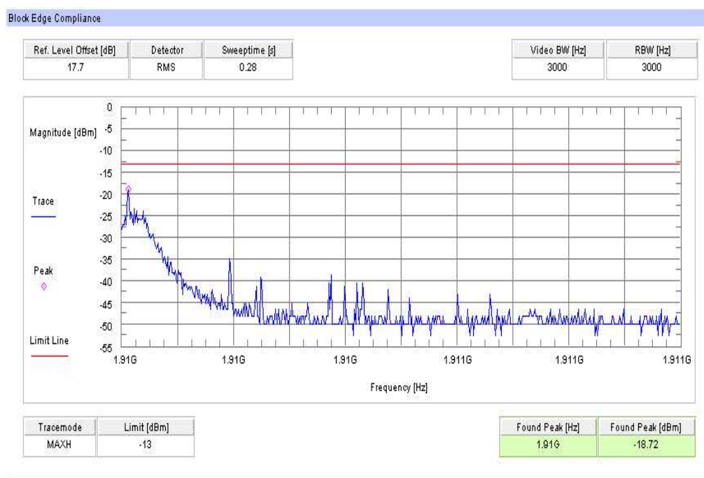
Plot 4: TX mode, channel 810, EGPRS / EDGE, block 6
