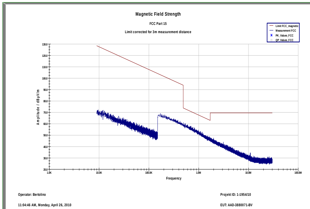
Plot 5: TX mode, channel 4180, UMTS / WCDMA, 10 kHz - 30 MHz (valid for all channels)
