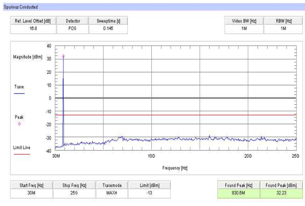
Plot 3: TX mode, channel 251, GSM, 30 MHz – 25 GHz
