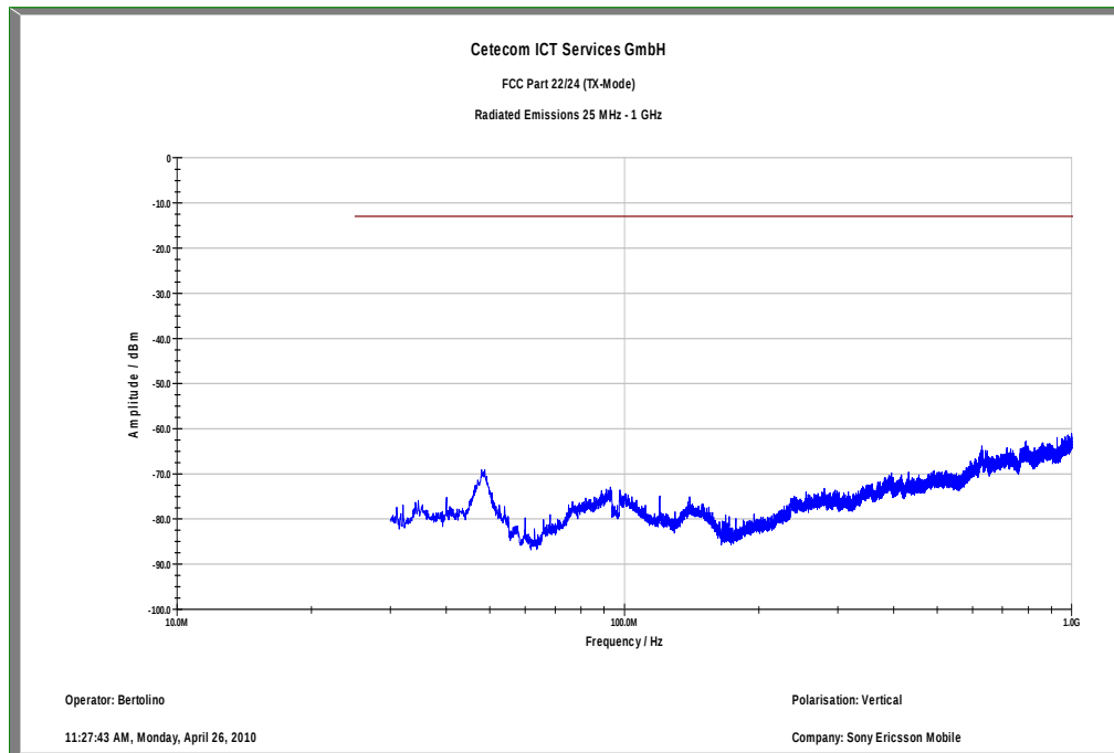
Plot 1: TX mode, channel 9262, UMTS / WCDMA, 30 MHz – 1 GHz, vertical polarization
