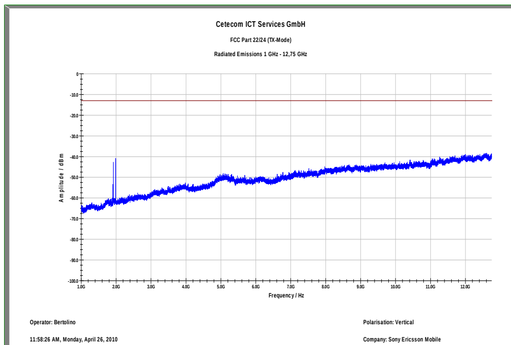
Plot 13: TX mode, channel 9538, UMTS / WCDMA, 1 GHz – 12.75 GHz, vertical polarization
