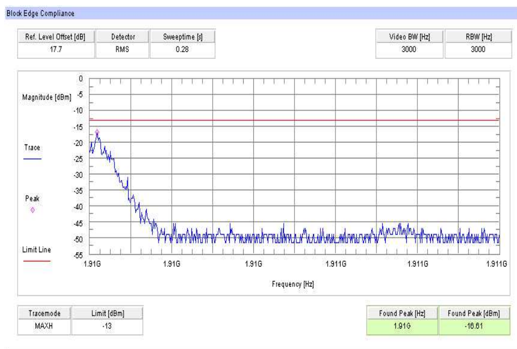
Plot 2: TX mode, channel 810, GSM, block 6
