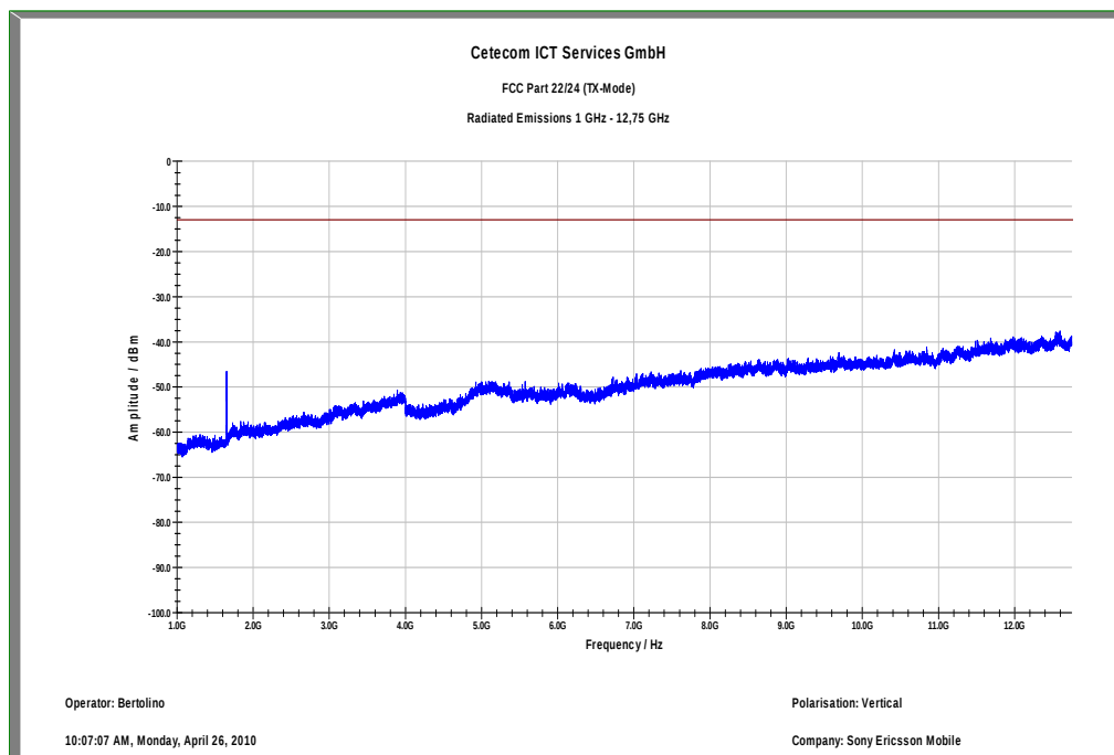
Plot 2: TX mode, channel 4132, UMTS / WCDMA, 1 GHz – 12.75 GHz, vertical polarization
