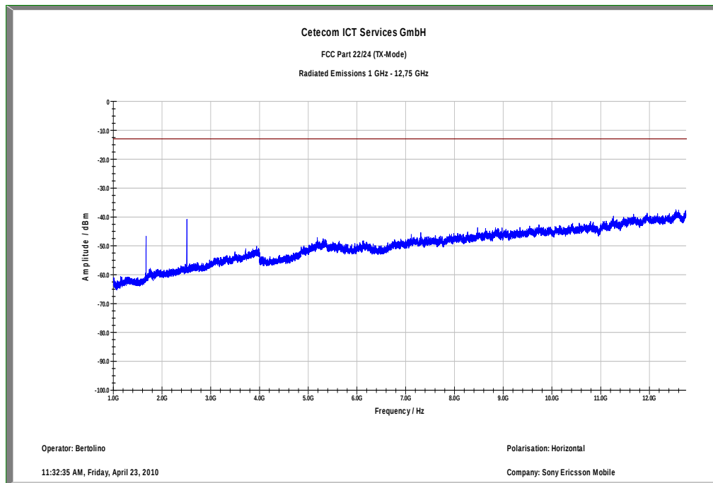
Plot 10: TX mode, channel 189, GSM, 1 GHz – 12.75 GHz, horizontal polarization
