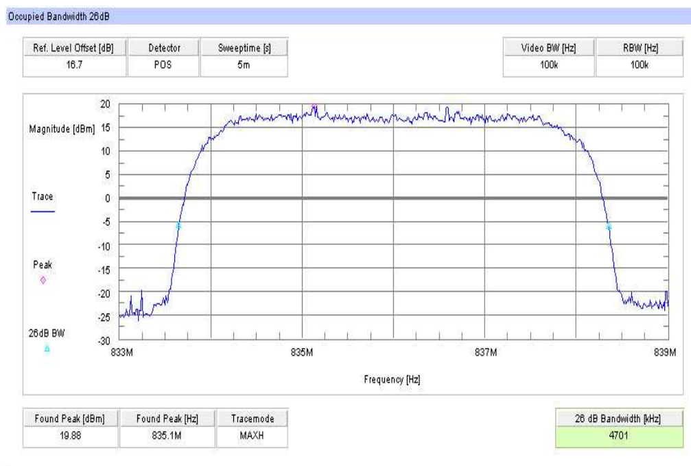
Plot 4: TX mode, channel 4180, UMTS / WCDMA, -26 dBc Bandwidth
