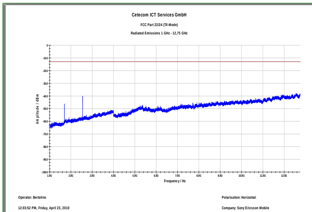
Plot 16: TX mode, channel 251, GSM, 1 GHz – 12.75 GHz, horizontal polarization
