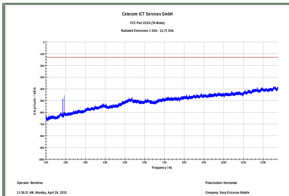
Plot 4: TX mode, channel 9262, UMTS / WCDMA, 1 GHz – 12.75 GHz, horizontal polarization
