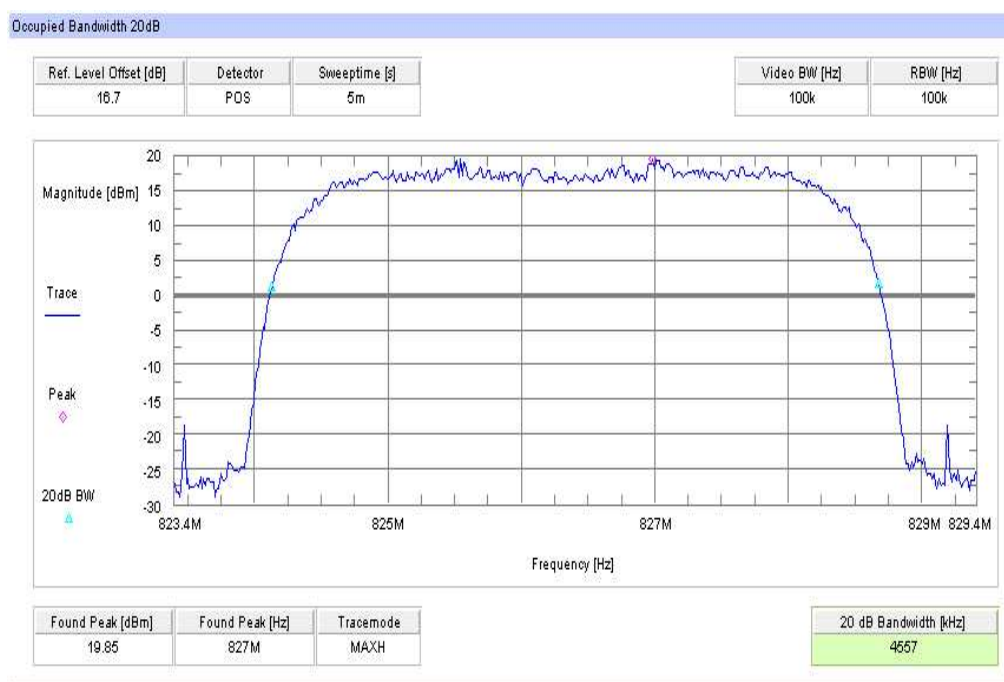
Plot 1: TX mode, channel 4132, UMTS / WCDMA, 99% (-20 dB) Occupied Bandwidth
