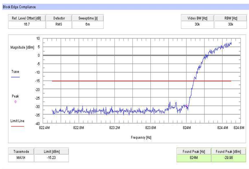
Plot 2: TX mode, channel 4132, UMTS / WCDMA
