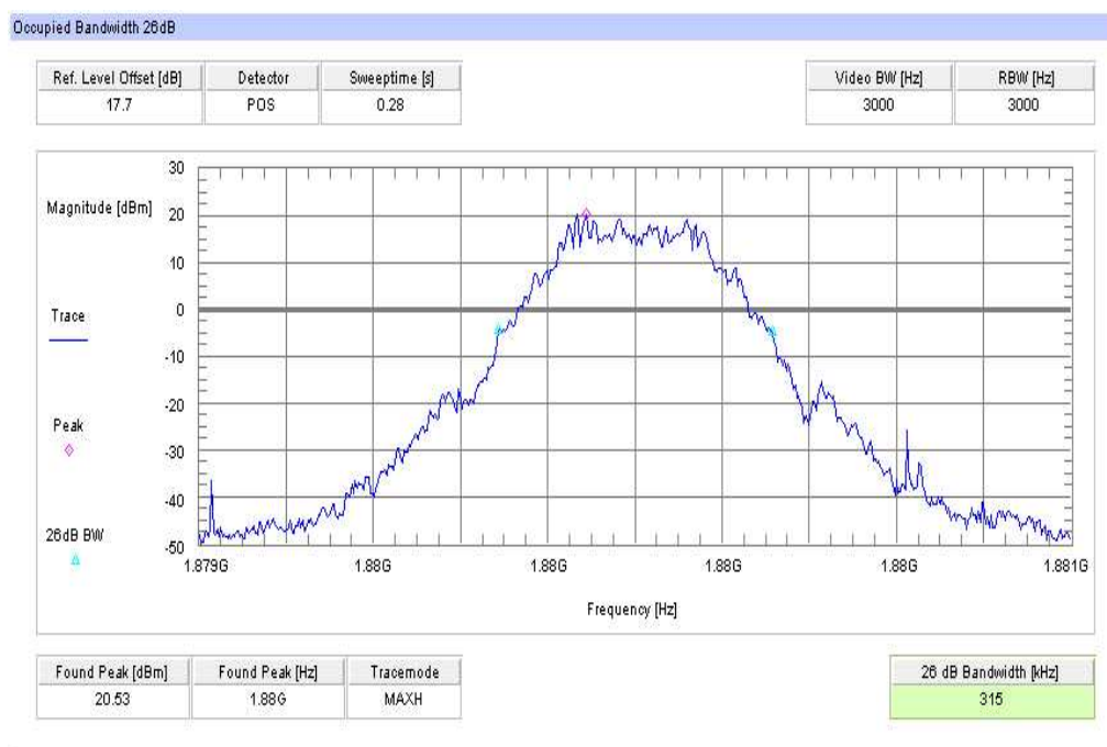
Plot 10: TX mode, channel 661, EGPRS / EDGE, -26 dBc Bandwidth
