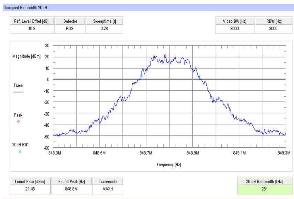
Plot 11: TX mode, channel 251, EGPRS / EDGE, 99% (-20 dB) Occupied Bandwidth
