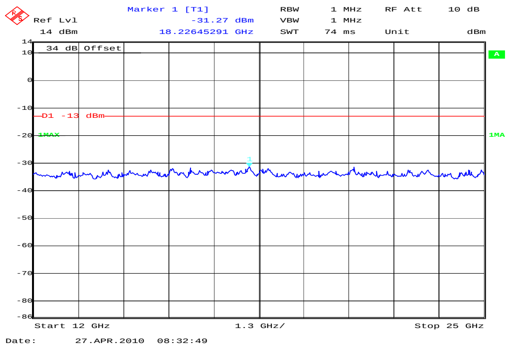
Plot 11: TX mode, channel 4180, UMTS / WCDMA, 12 GHz - 25 GHz (valid for all channels)
