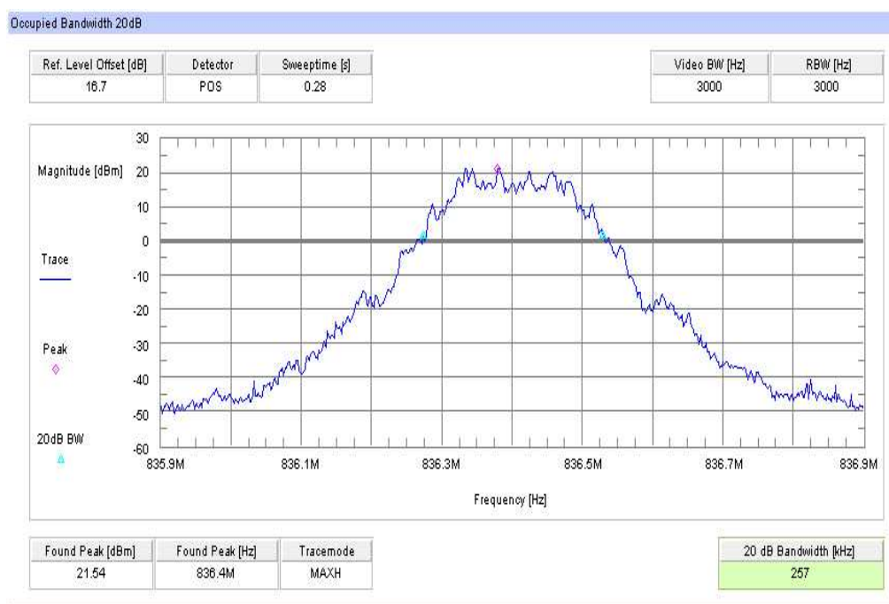
Plot 9: TX mode, channel 189, EGPRS / EDGE, 99% (-20 dB) Occupied Bandwidth
