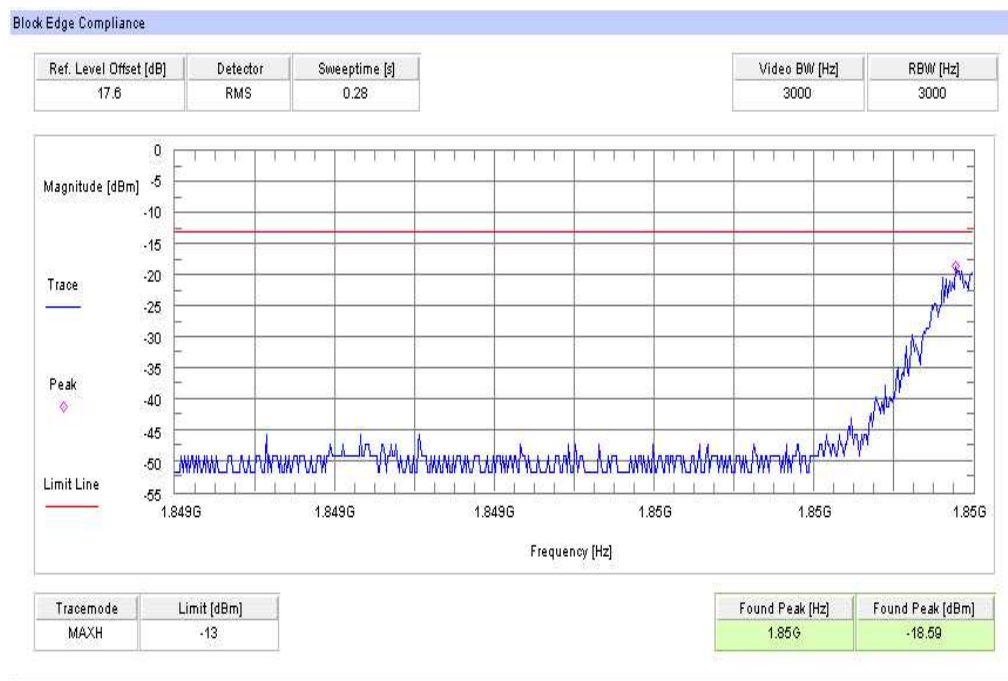
Plot 1: TX mode, channel 512, GSM, block 1
