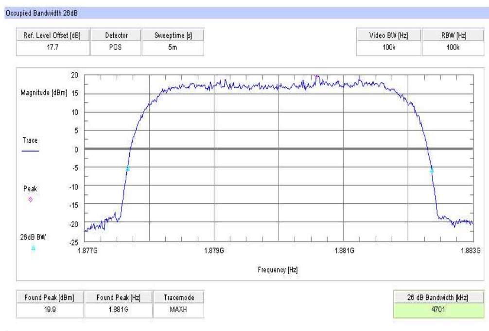
Plot 4: TX mode, channel 9400, UMTS / WCDMA, -26 dBc Bandwidth
