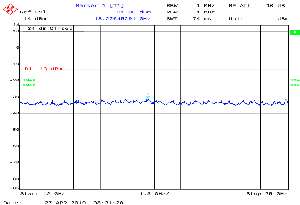
Plot 11: TX mode, channel 9400, UMTS / WCDMA, 12 GHz - 25 GHz (valid for all channels)
