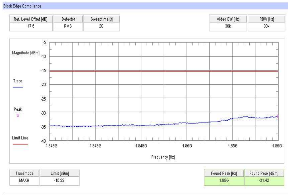
Plot 1: TX mode, channel 9262, UMTS / WCDMA
