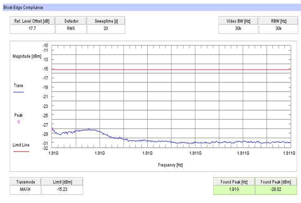
Plot 2: TX mode, channel 9538, UMTS / WCDMA
