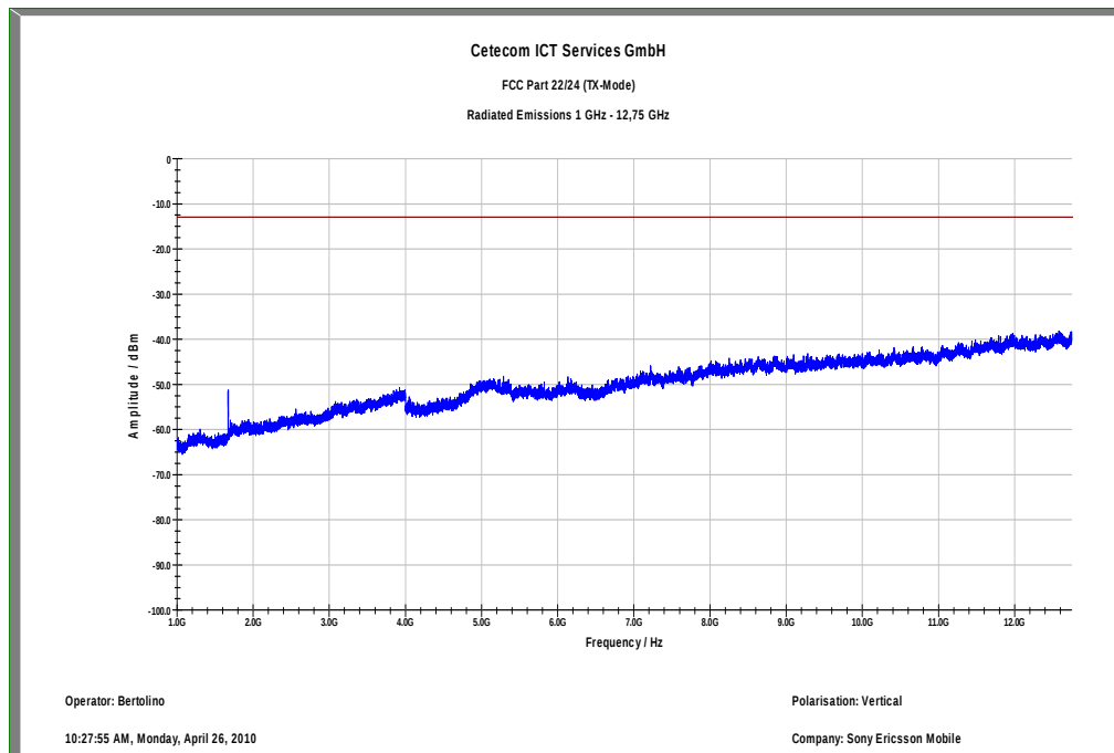
Plot 8: TX mode, channel 4180, UMTS / WCDMA, 1 GHz – 12.75 GHz, vertical polarization
