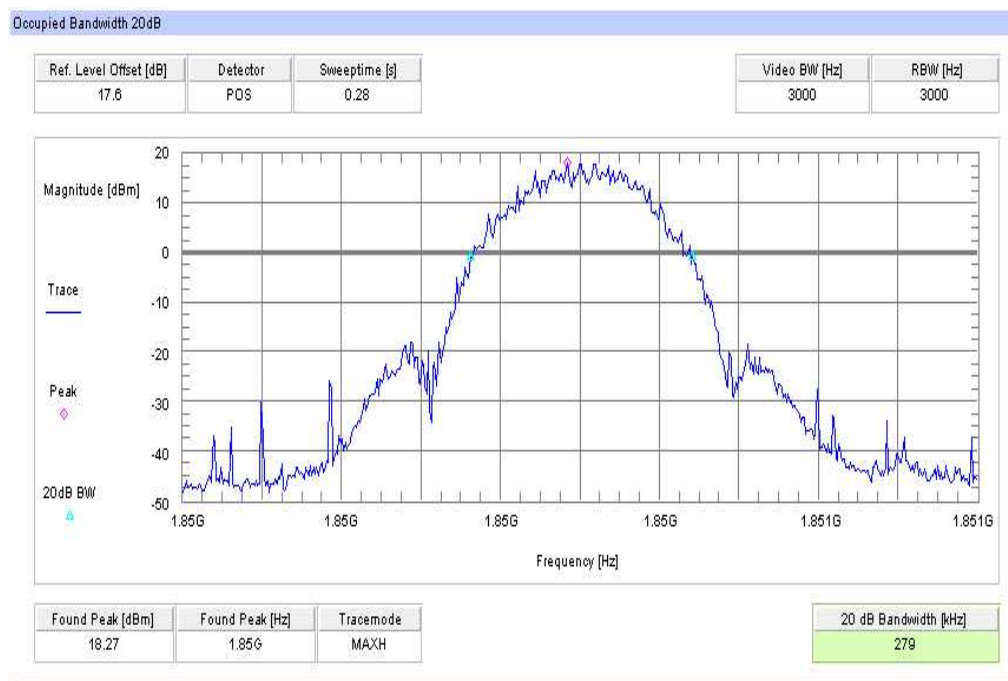
Plot 7: TX mode, channel 512, EGPRS / EDGE, 99% (-20 dB) Occupied Bandwidth
