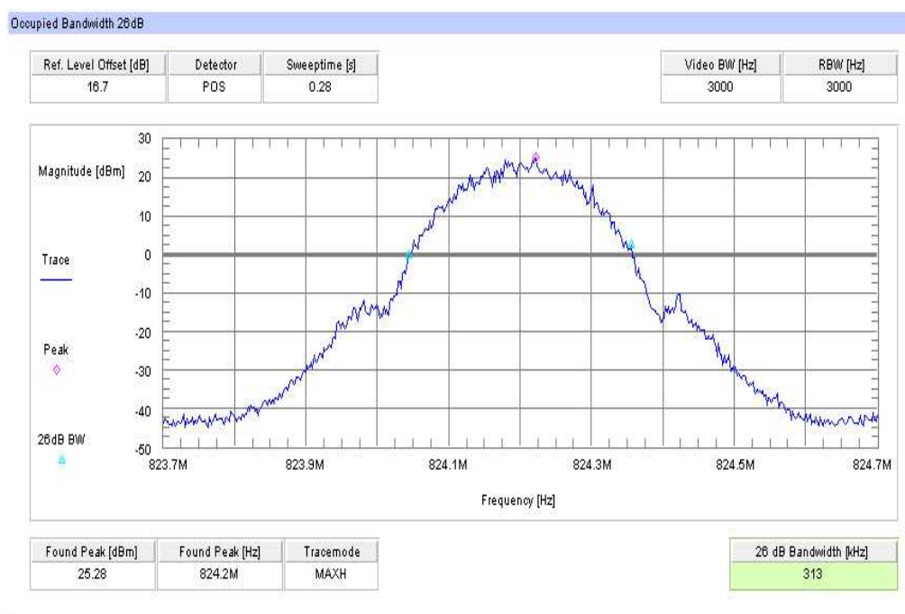
Plot 2: TX mode, channel 128, GSM, -26 dBc Bandwidth
