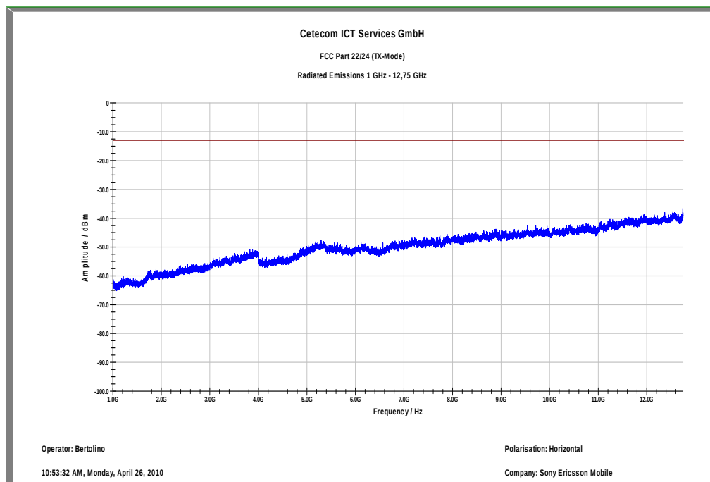
Plot 15: TX mode, channel 4233, UMTS / WCDMA, 1 GHz – 12.75 GHz, horizontal polarization
