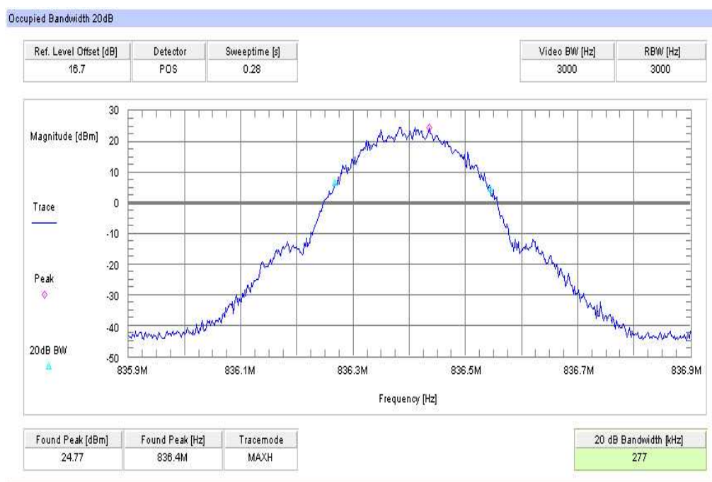
Plot 3: TX mode, channel 189, GSM, 99% (-20 dB) Occupied Bandwidth
