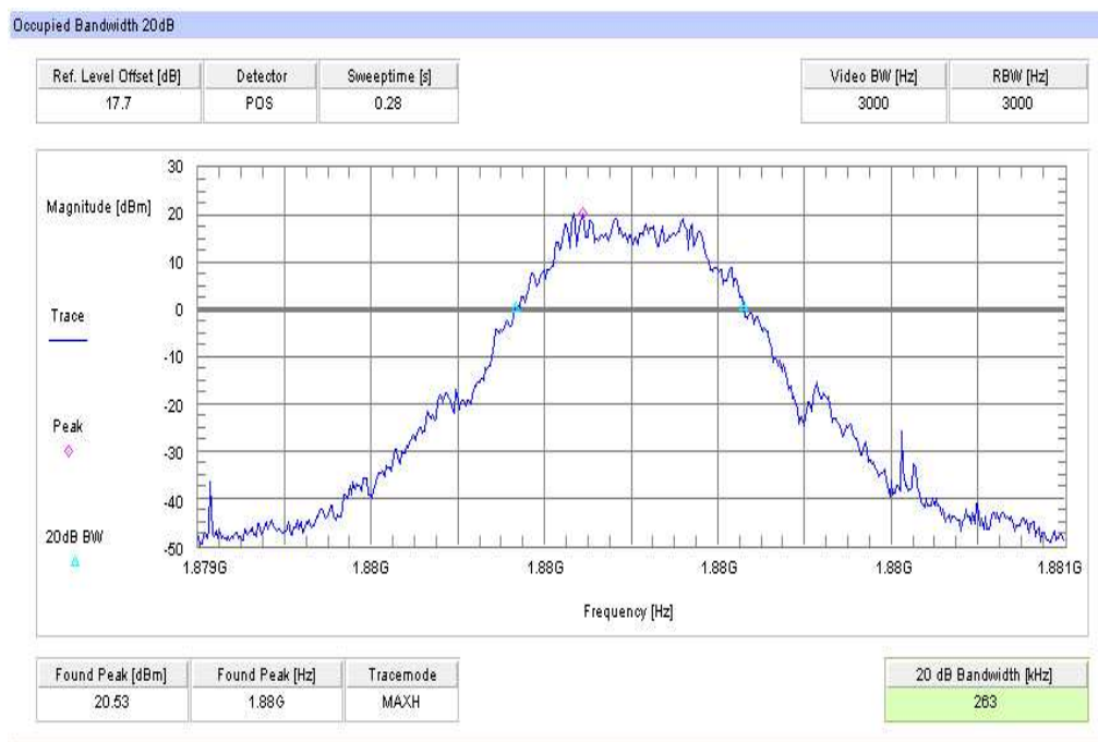
Plot 9: TX mode, channel 661, EGPRS / EDGE, 99% (-20 dB) Occupied Bandwidth
