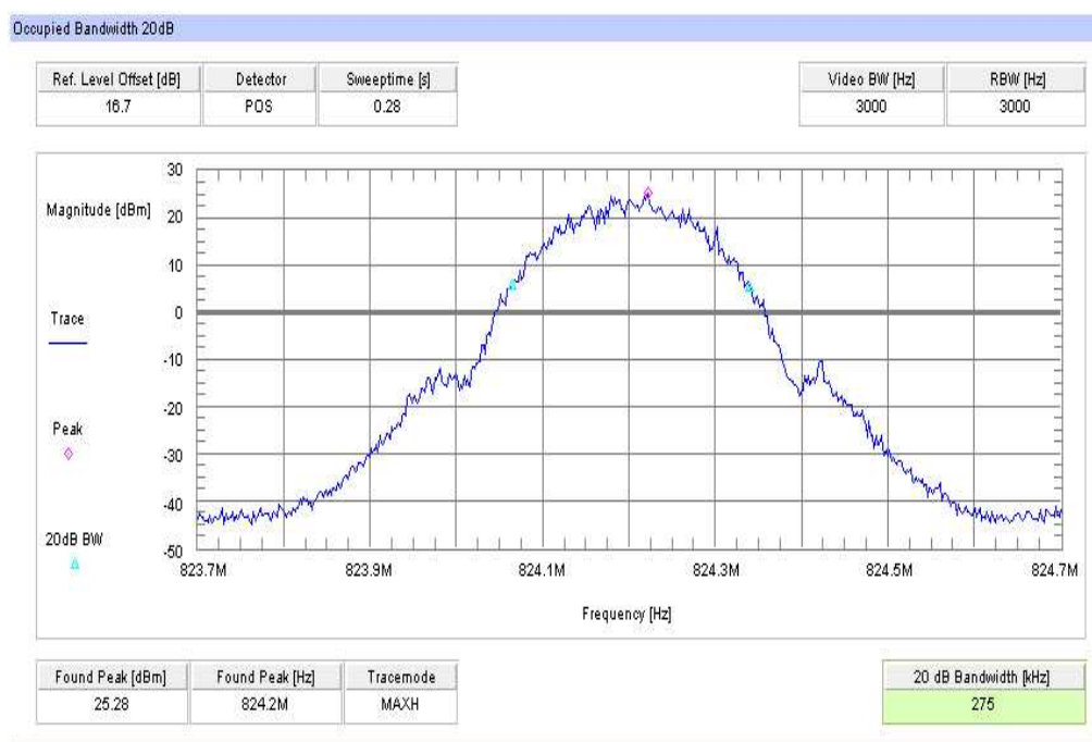
Plot 1: TX mode, channel 128, GSM, 99% (-20 dB) Occupied Bandwidth
