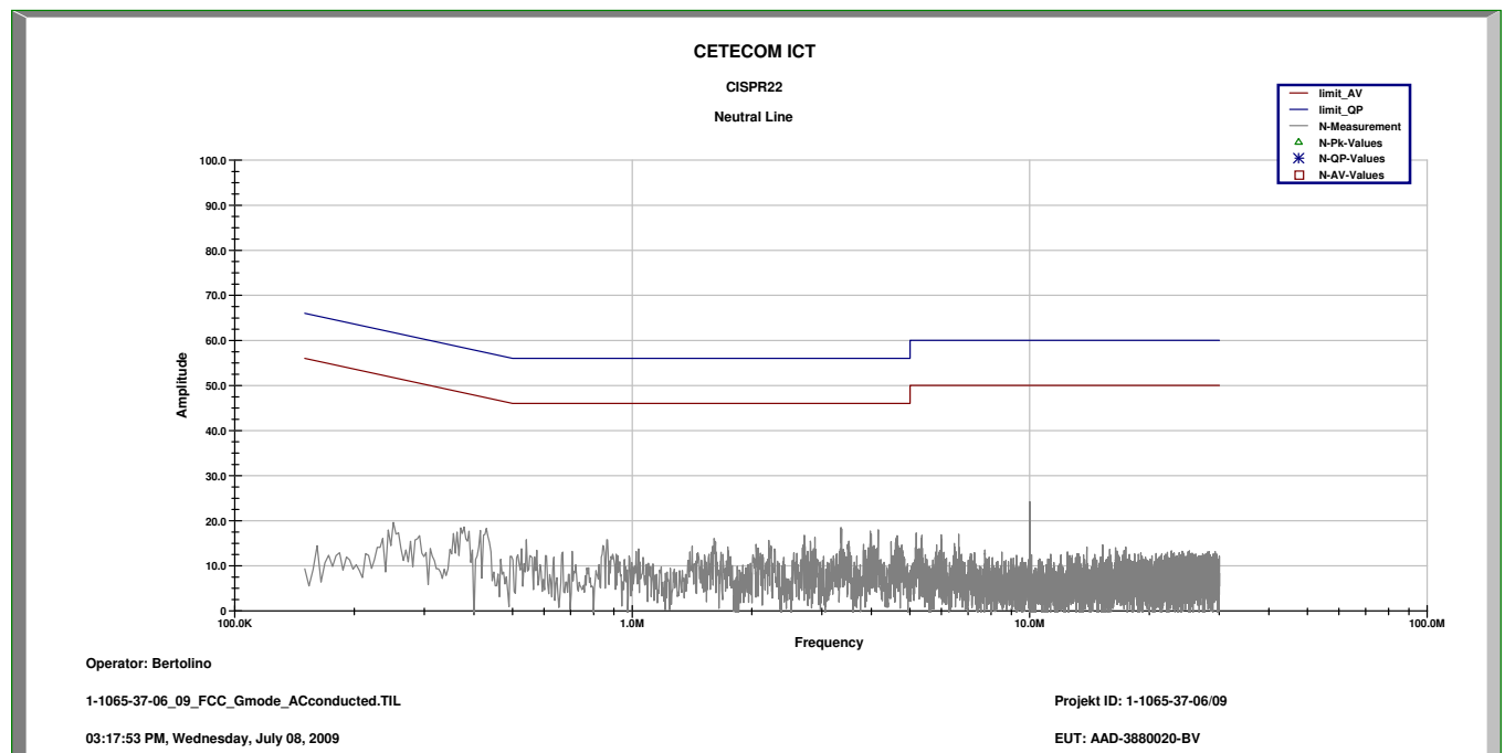
Plot 4: Neutral line, TX mode, OFDM
