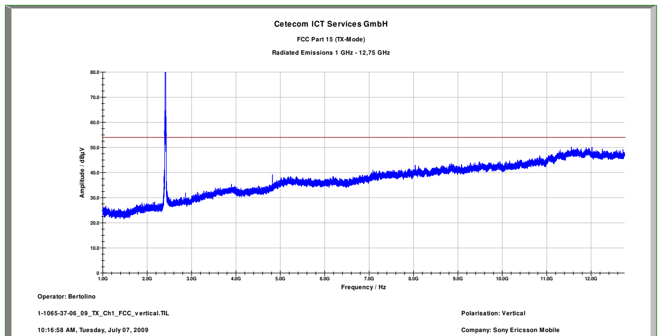
Plot 2: 1 GHz – 12.75 GHz (lowest channel), vertical
