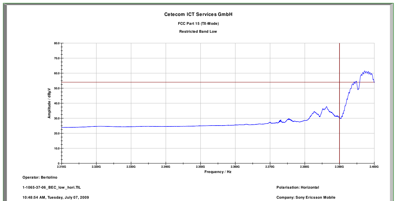
Plot 3: Restricted band low, horizontal
