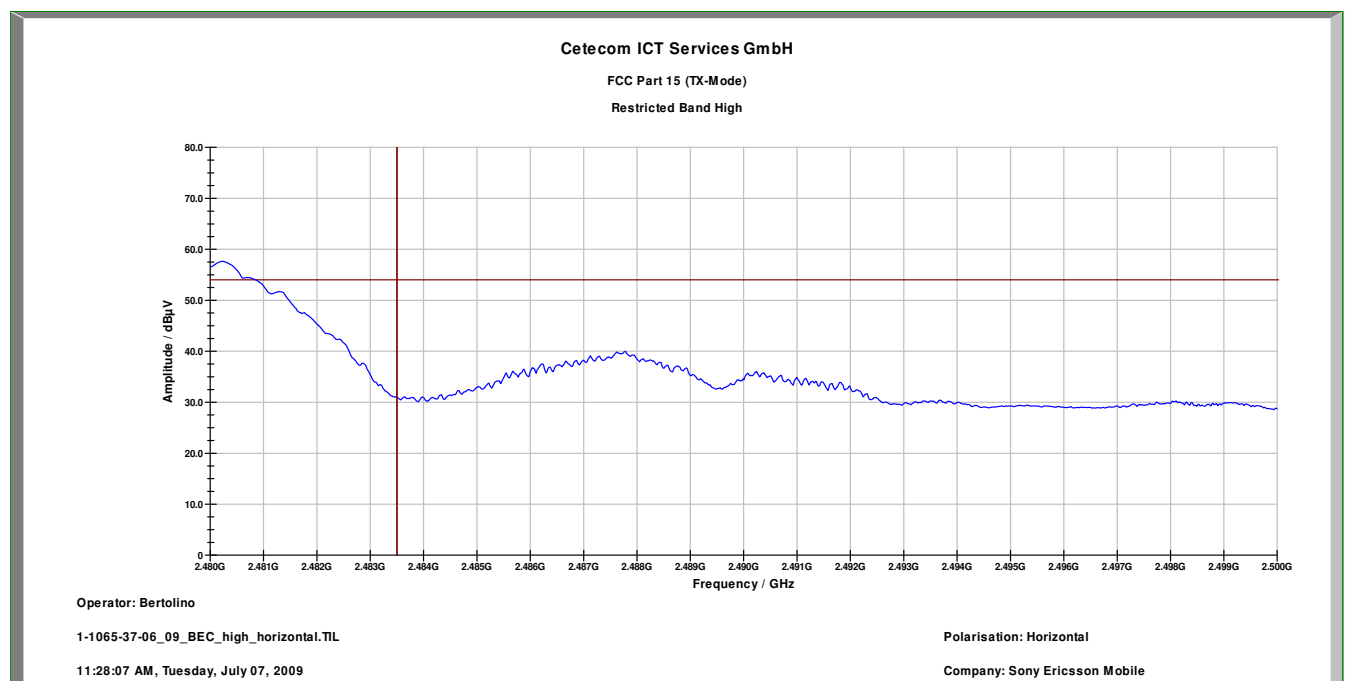
Plot 4: Restricted band high, horizontal
