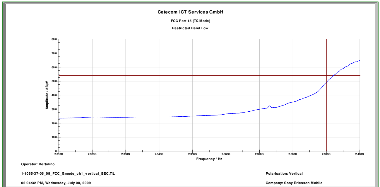
Plot 1: Restricted band low, vertical
