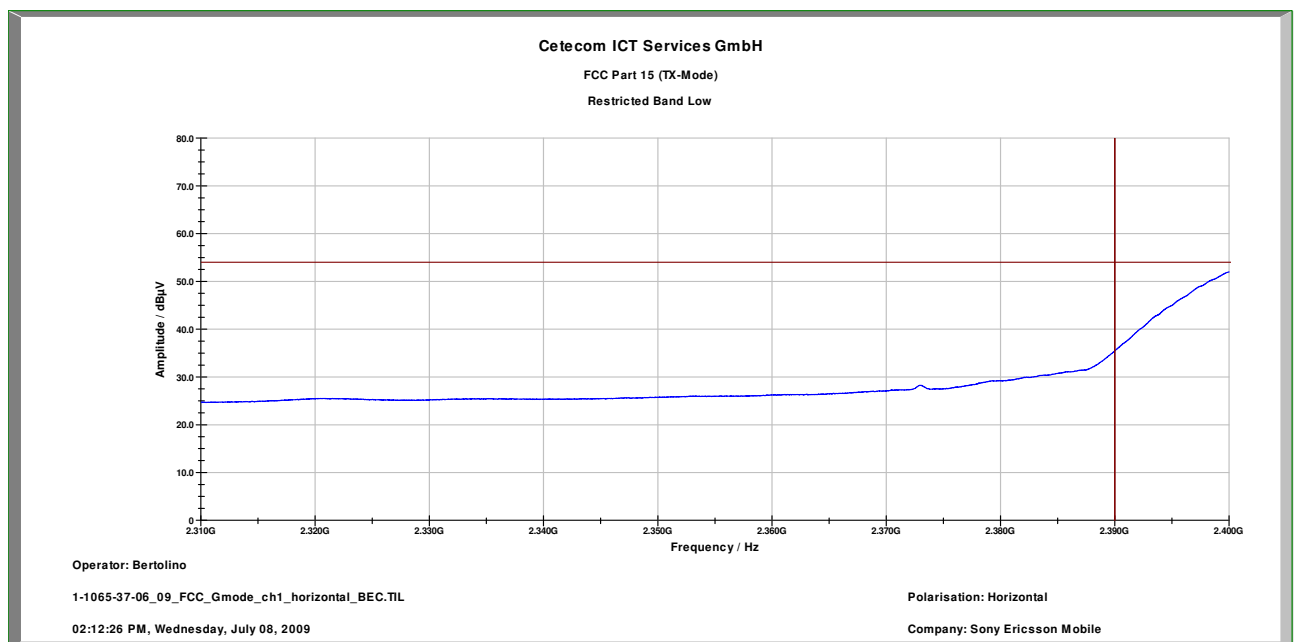
Plot 3: Restricted band low, horizontal
