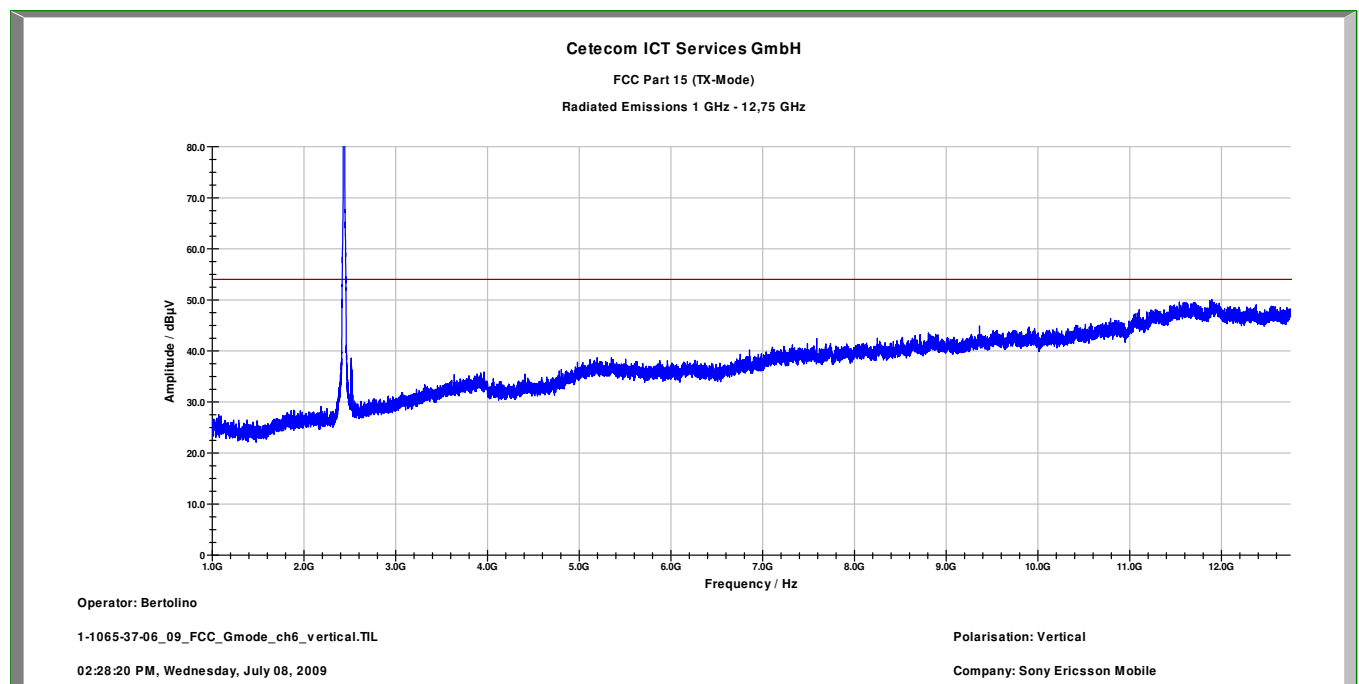
Plot 6: 1 GHz – 12.75 GHz (middle channel), vertical
