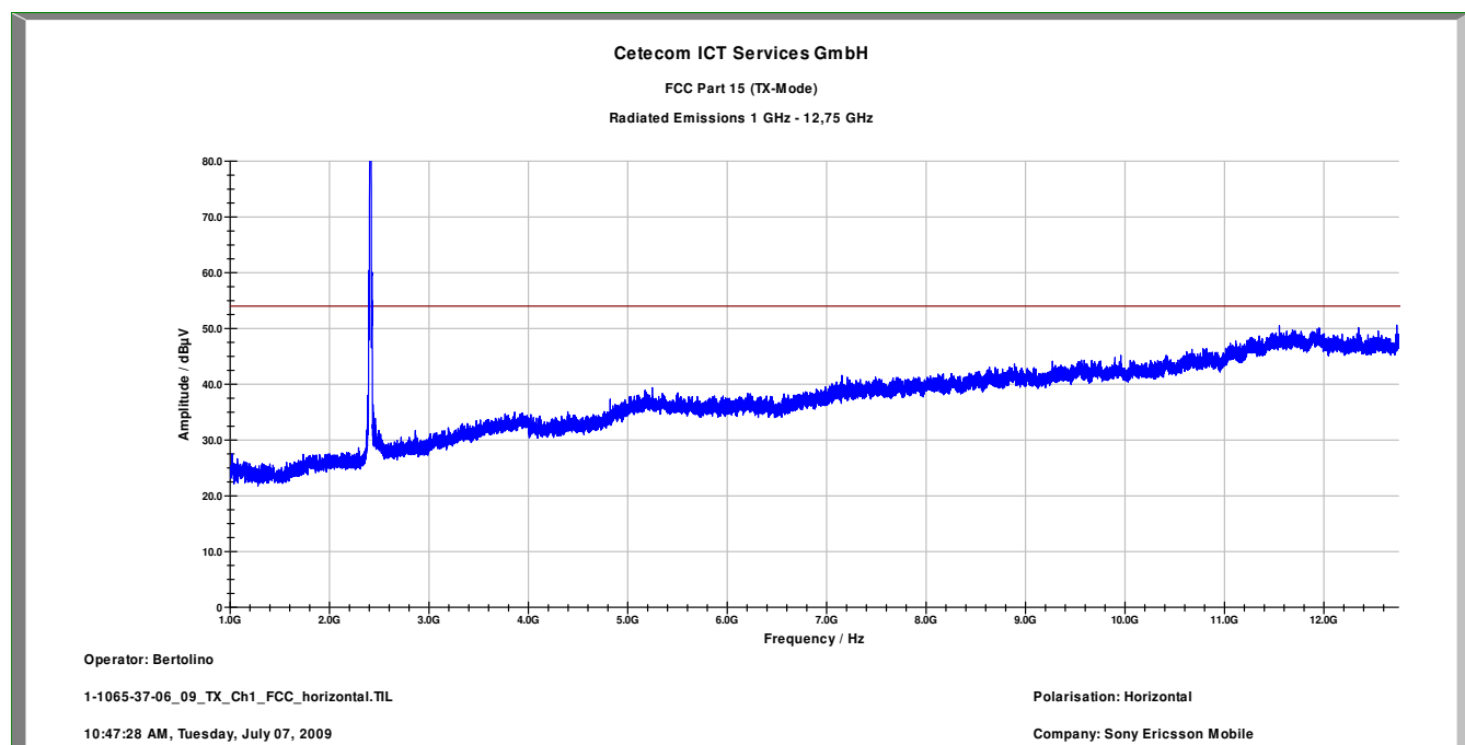
Plot 3: 1 – 12.75 GHz (lowest channel), horizontal
