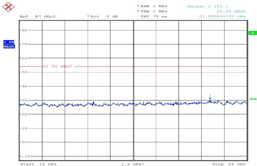
Plot 4: 12 - 25 GHz (valid for all channels), vertical & horizontal
