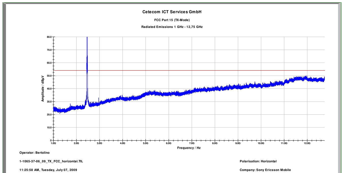
Plot 10: 1 – 12.75 GHz (highest channel), horizontal
