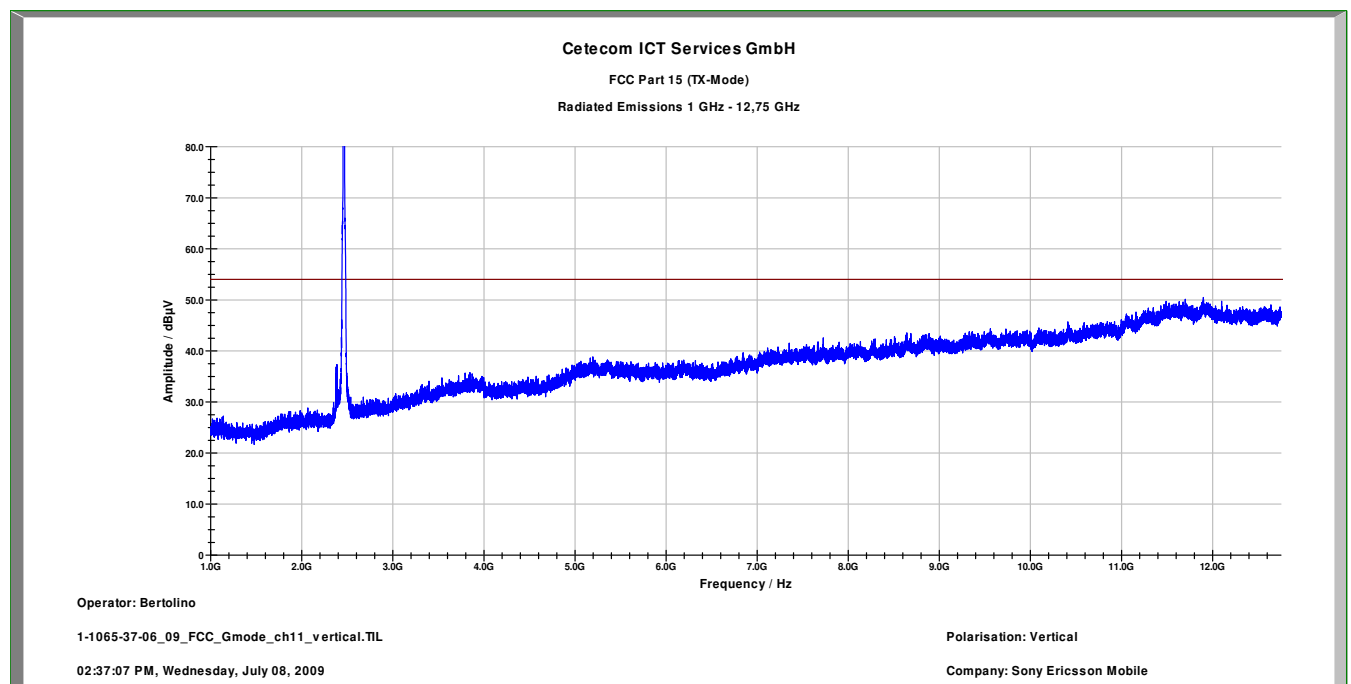
Plot 9: 1 GHz – 12.75 GHz (highest channel), vertical
