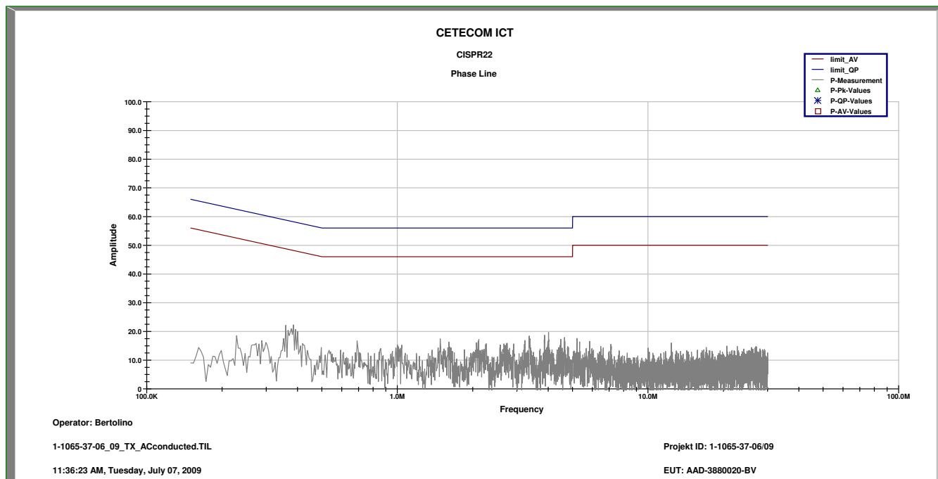
Plot 1: Phase line, TX mode, DSSS
