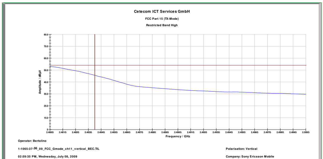
Plot 2: Restricted band high, vertical
