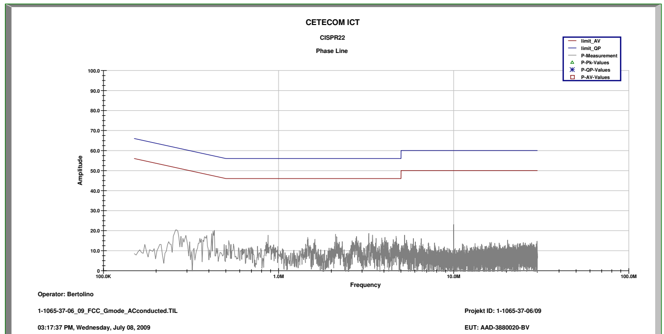
Plot 3: Phase line, TX mode, OFDM
