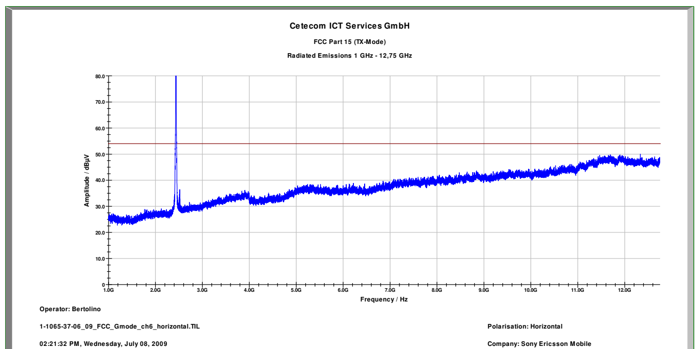
Plot 7: 1 – 12.75 GHz (middle channel), horizontal
