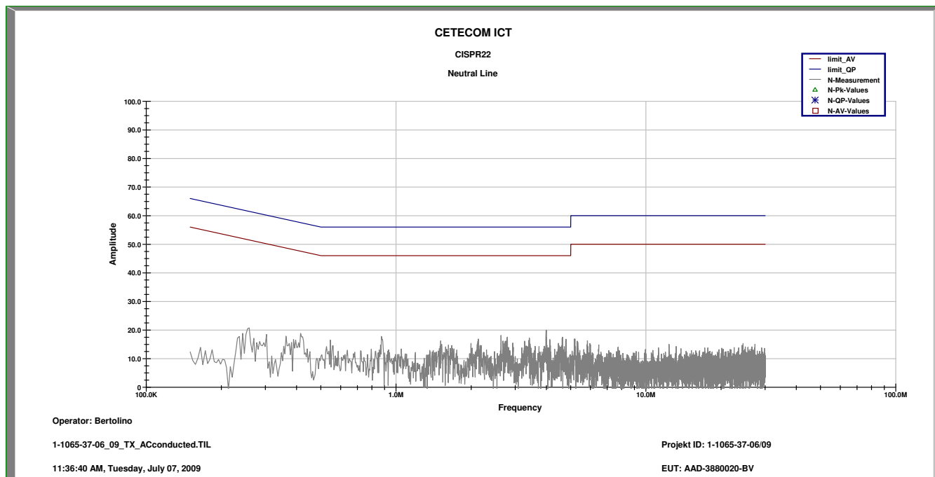
Plot 2: Neutral line, TX mode, DSSS
