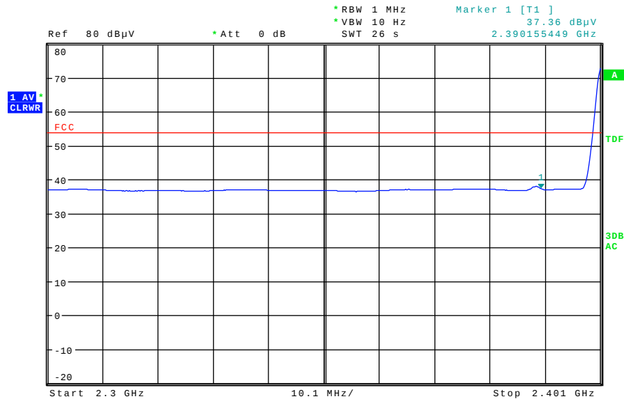
Plot 1: Band edge compliance and far away emissions – Lowest Channel
