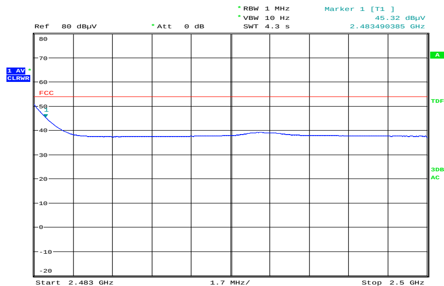
Plot 2: Band edge compliance and far away emissions – Highest Channel
