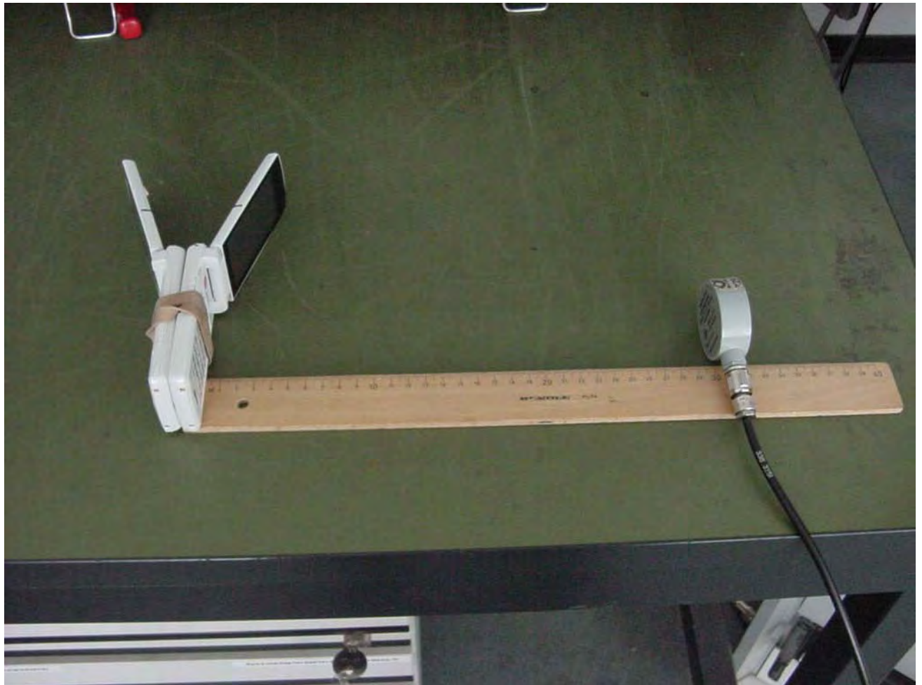
Photo No.4: Field strength measurement
