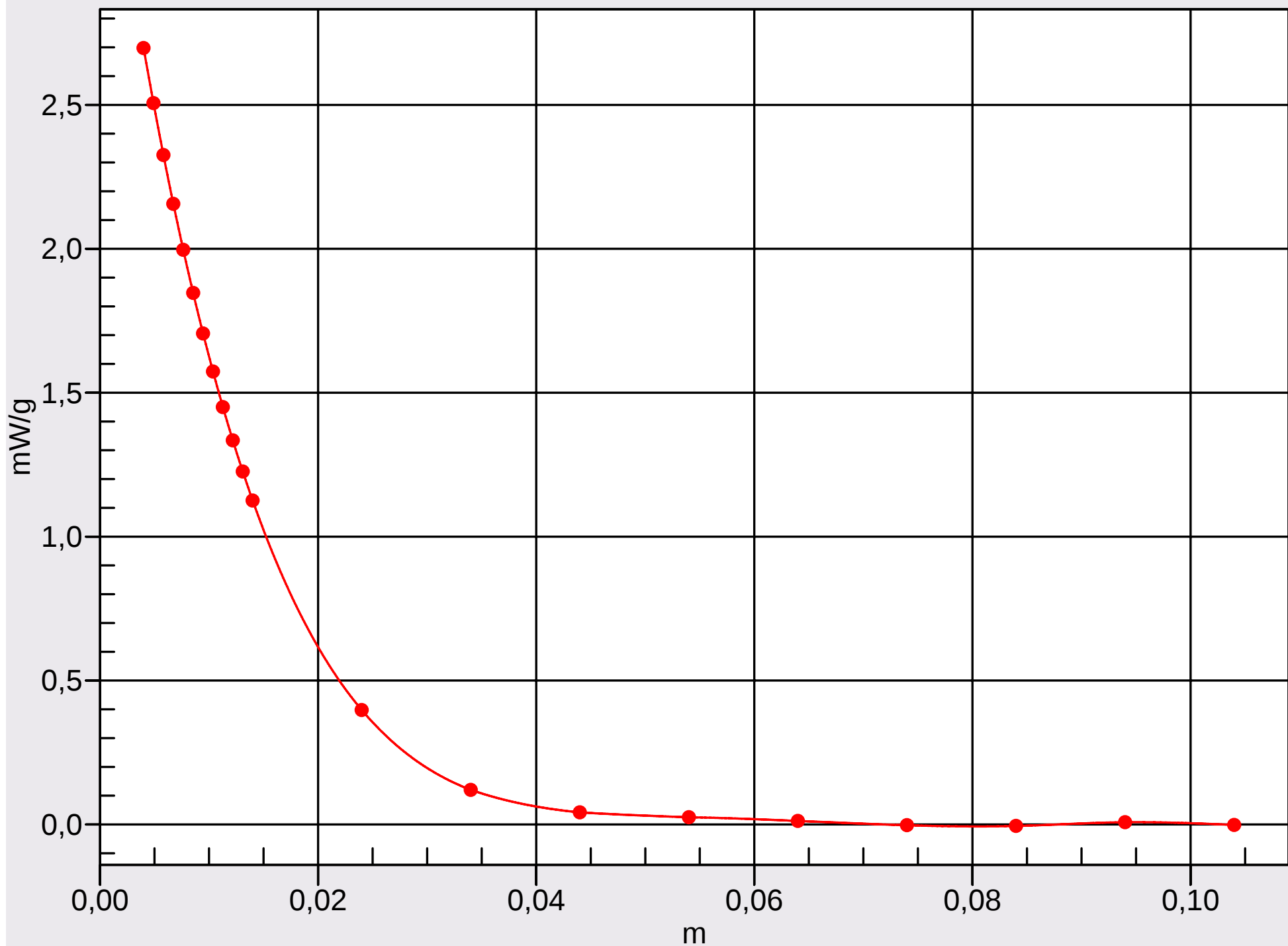
Interpolated SAR(x,y,z,f0) HSL1900; Z Scan: Value Along Z, X=0, Y=0
