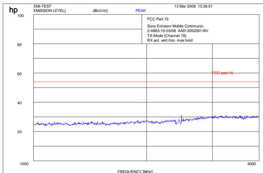
Plot: 1 - 4 GHz vertical/horizontal (highest channel)
