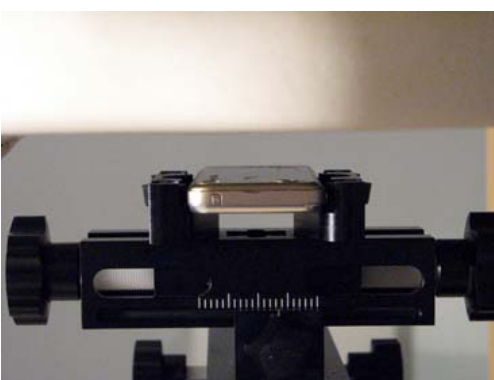
Device position towards the body: Phone on 15mm distance against Phantom
