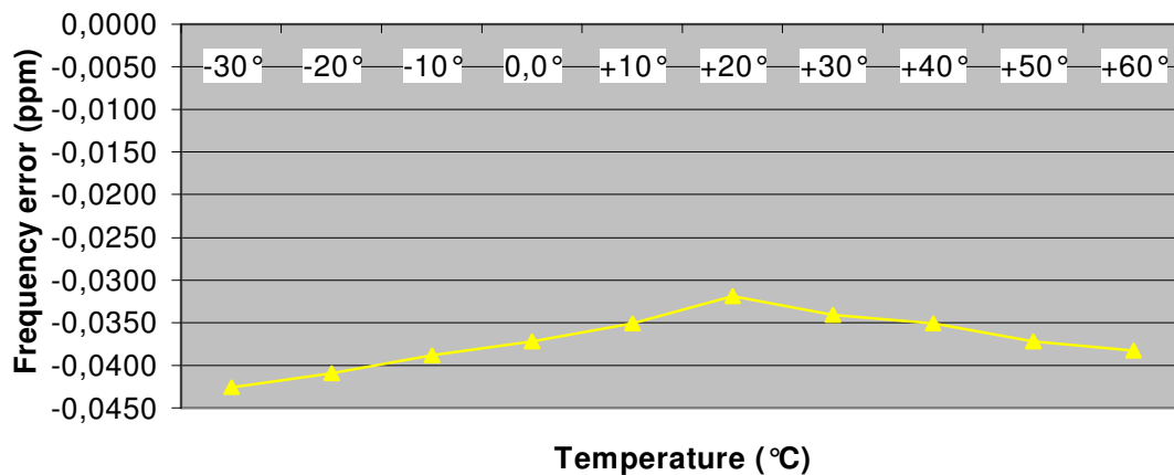
Frequency Error vs. Temperatur
