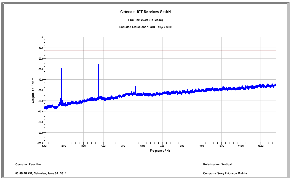
Plot 3: Channel 661 (1 GHz – 12.75 GHz)
