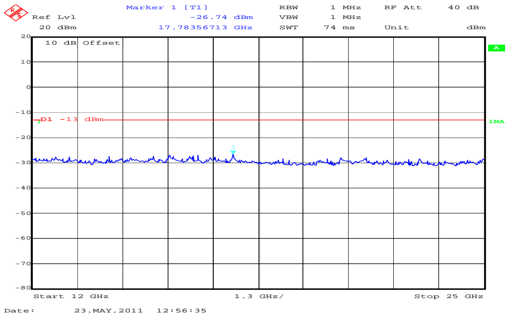
Plot 4: Channel 661 (12 GHz - 25 GHz)
