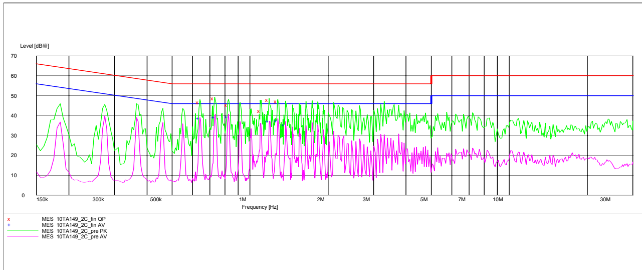
Fig. 110 AC Powerline Conducted Emission with charger-Idle Mode
