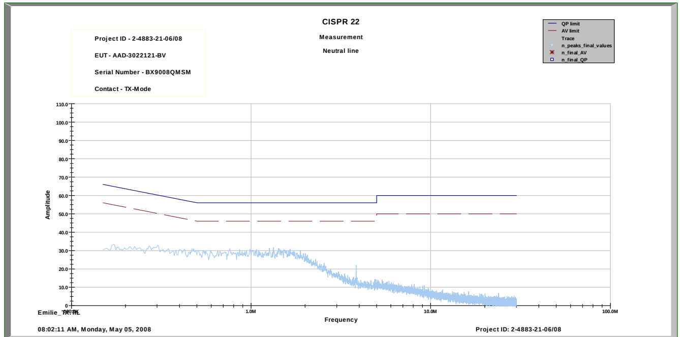
Plot 1: TX mode
