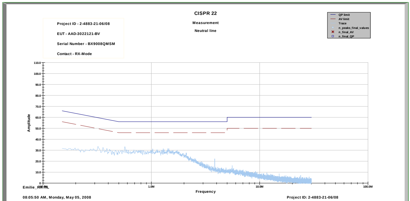
Plot 3: RX mode
