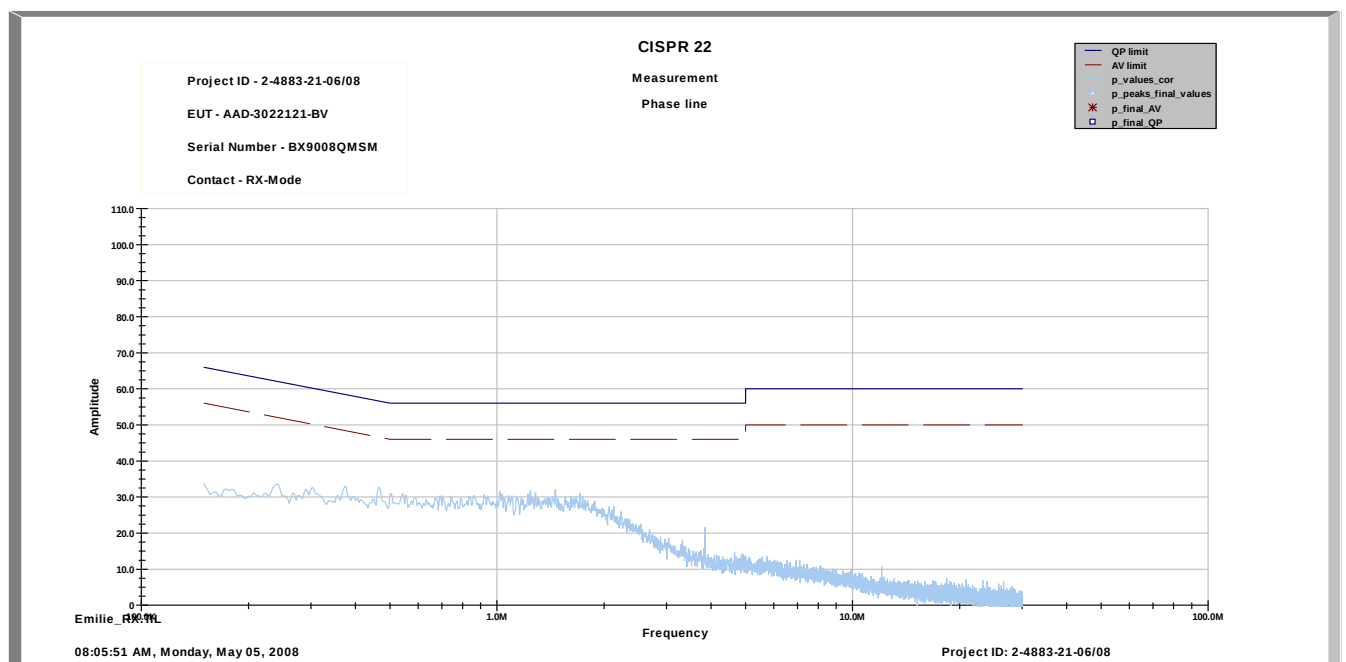
Plot 4: RX mode
