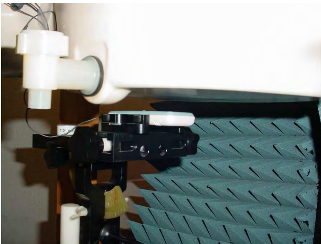
Photo 20: Test position body worn front side (15 mm distance)
