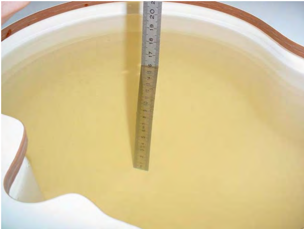
Photo 24: Liquid depth 850 MHz body simulating liquid
