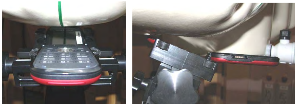
DUT position towards the head: Tilt (touch + 15°) position
