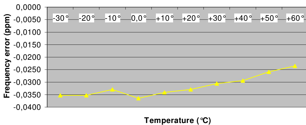
Frequency Error vs. Temperature
