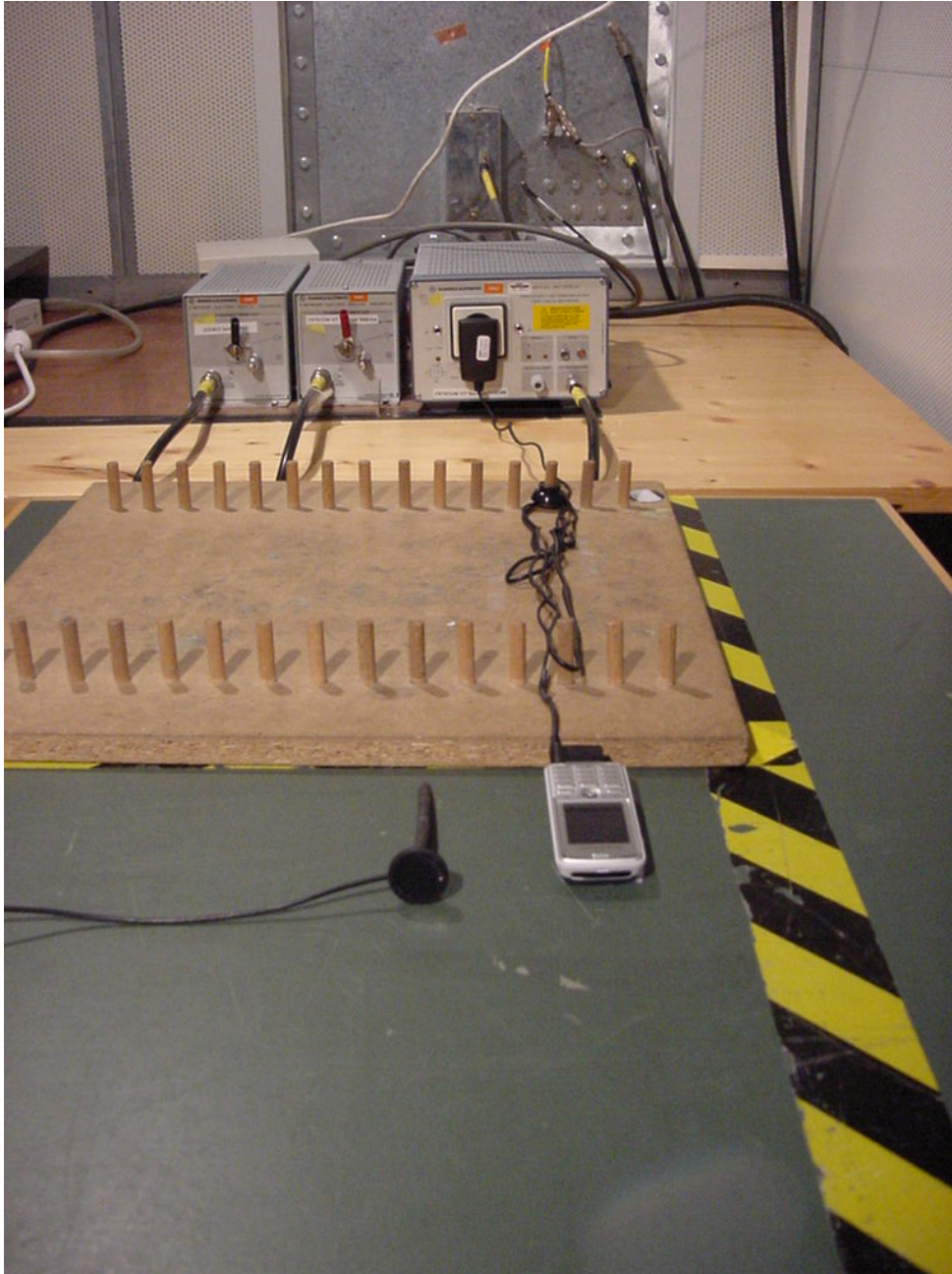
Photo 3 (Conducted Emissions):
