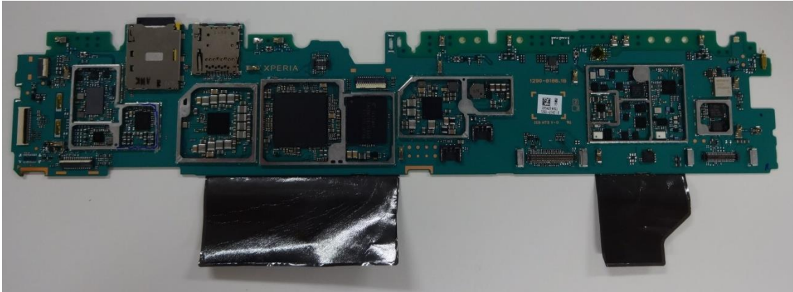
Internal PWB without Shield cases (Front-side)
