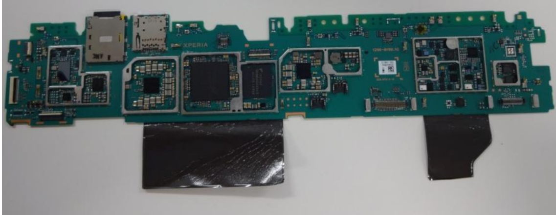
Internal PWB without Shield cases (Front-side)
