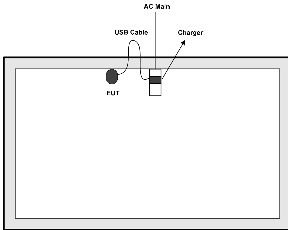
Test Setup Diagram - Radiated Test (Below 1GHz) - Mode 2
