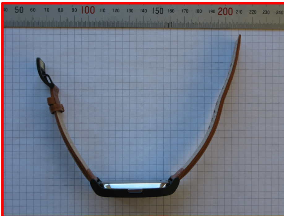
Photograph I1.4 – Right Edge of Device with 1294-5702 (Carrier) and 1276-4067 (Leather Band)
