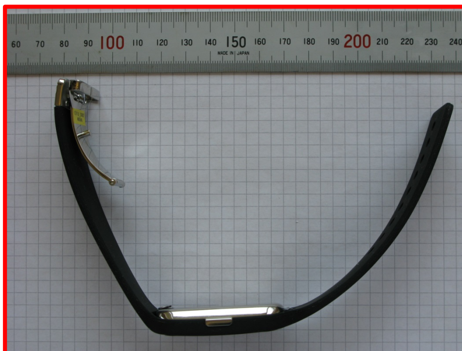
Photograph I1.8 – Right Edge of the Device with “Classic” strap 1289-1690
