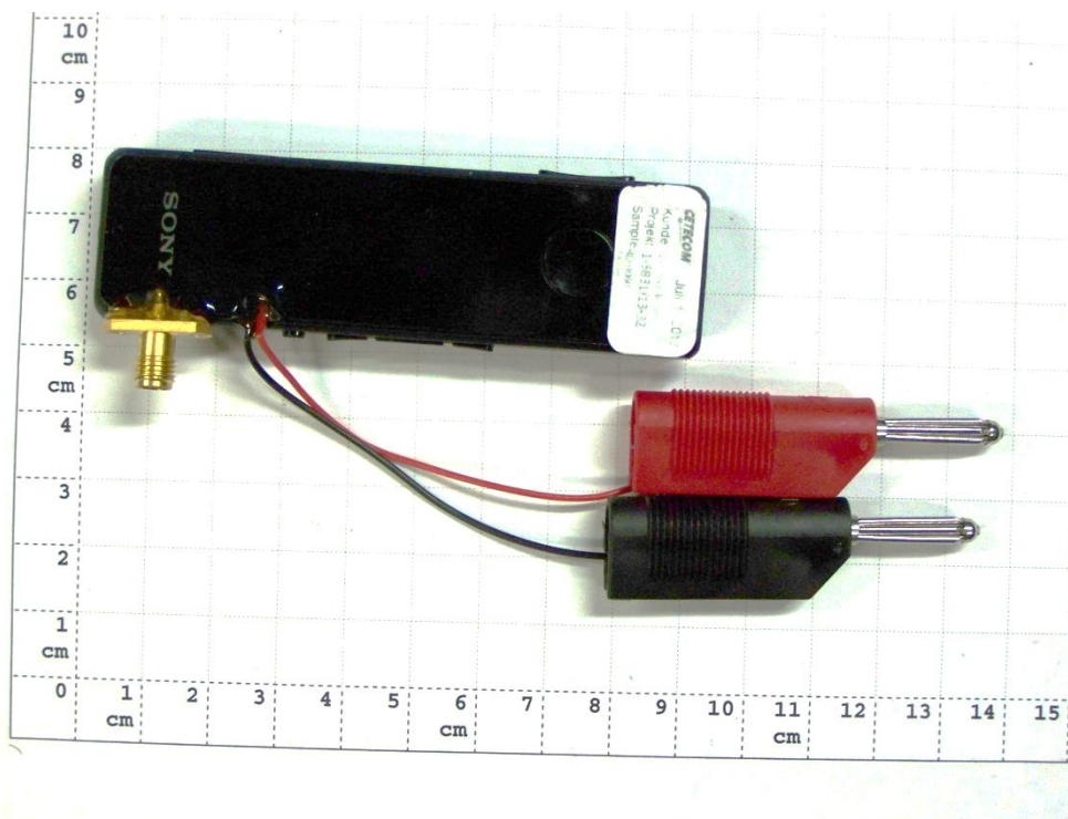
EUT b – modified sample for conducted RF-tests
